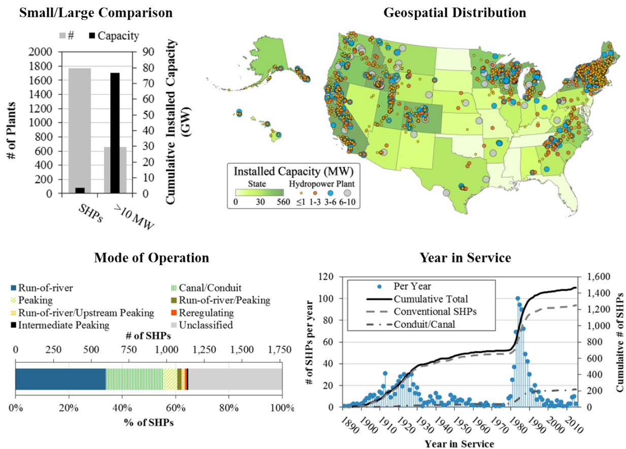
Figure 1 Characteristics of the U.S. Small Hydro Fleet
