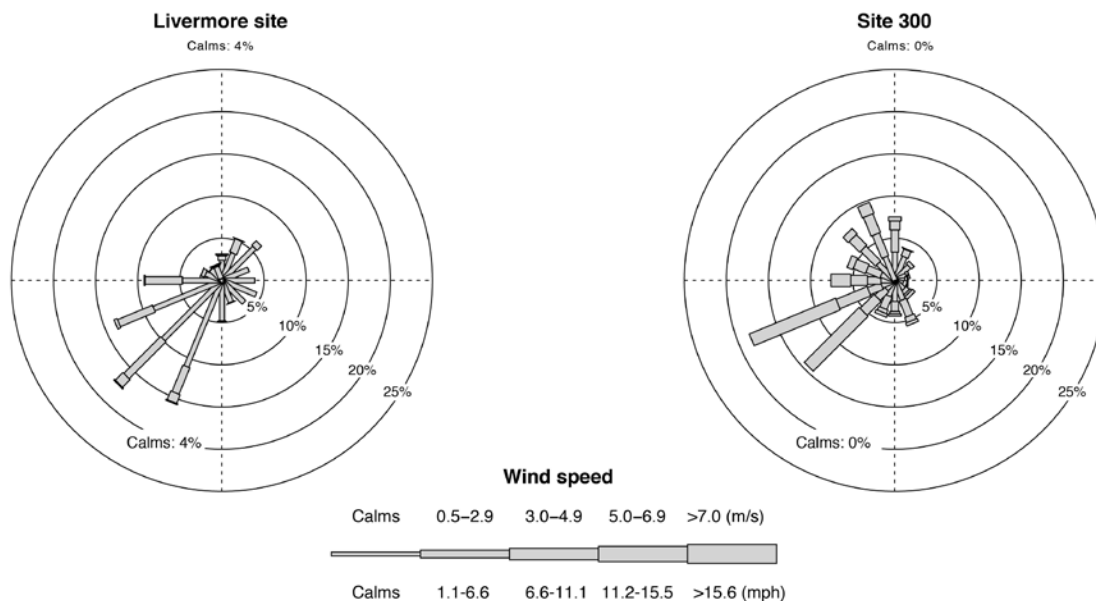
Figure 1-2. Wind roses showing wind direction and wind speed frequencies at the Livermore Site and Site 300 during 2016. The length of each spoke is proportional to the frequency at which the wind blows from the indicated direction. Different line widths of each spoke represent wind speed classes.
