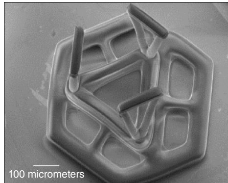
Livermore's design for a micromirror array comprises upwards of 10,000 hexagonal-element arrays, each measuring 1 millimeter square. The images show (left) a single fabricated mirror and (right) three microflexures printed on the underside of a micromirror, awaiting attachment to a paddle.
