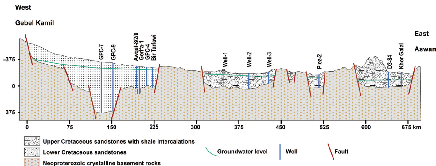
Figure 9. Schematic geological west-east cross section along the Uweinat-Aswan uplift (profile A-A'; Fig. 6) generated from well data and basement relief map (Fig. 7).
