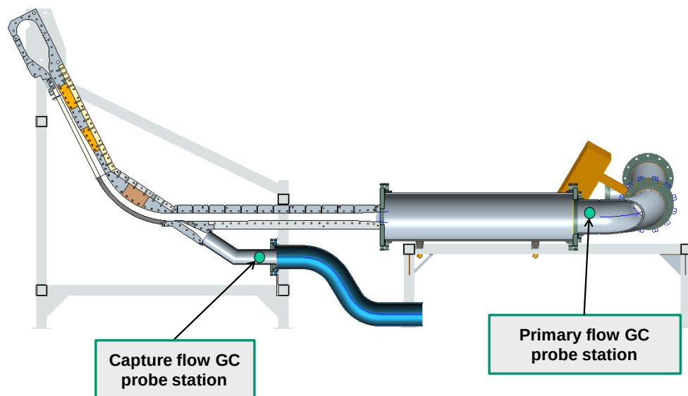
Figure 33: Gas Sampling Probe Locations for Gas Chromatography (GC) Measurements
