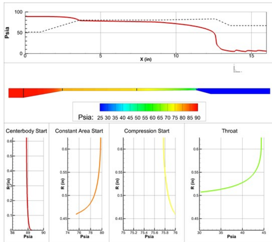
Figure 64 CFD Results for 0.919 OD Centerbody - Pressure
