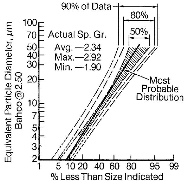
Exhibit 3-5 Flyash particle-size distribution in pulverized coal fired boilers.[7]
