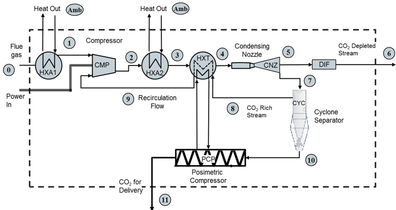
Figure 1-1 Block Flow Diagram of the Updated ICES Process
