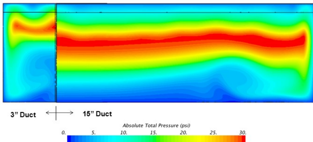
Figure 21 Comparison of total pressure contours at end of curved duct for current 3" wide rig (left) and 15" wide rig (right).
