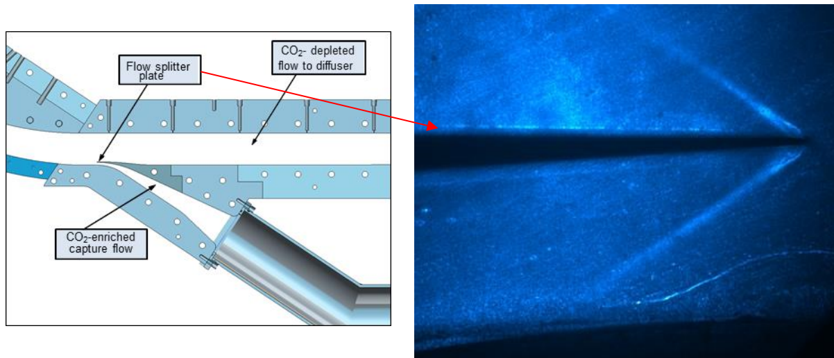
Figure 42 Capture duct configuration and Schlieren image of the splitter plate lip.
