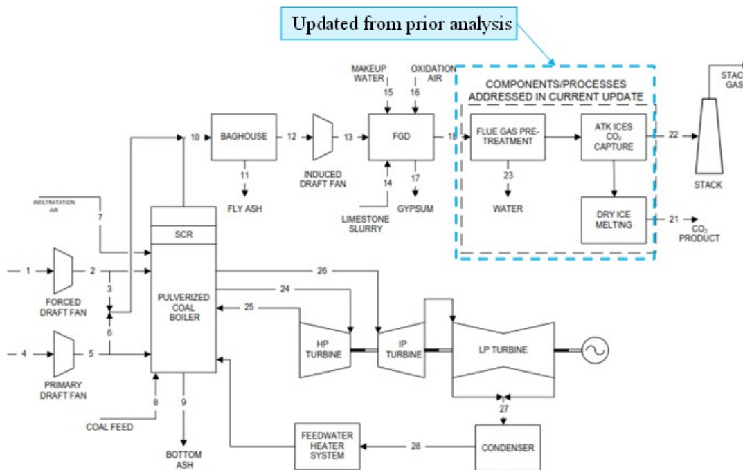
Figure 92 Updated Plant Block Diagram
