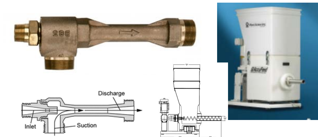
Figure 53 Commercial components for powder seeder
