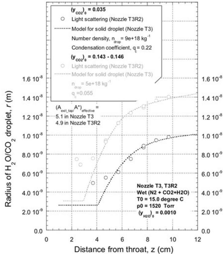
Figure 14: The size of the CO 2 particles derived LSM (circles) and model calculations (dashed lines).
