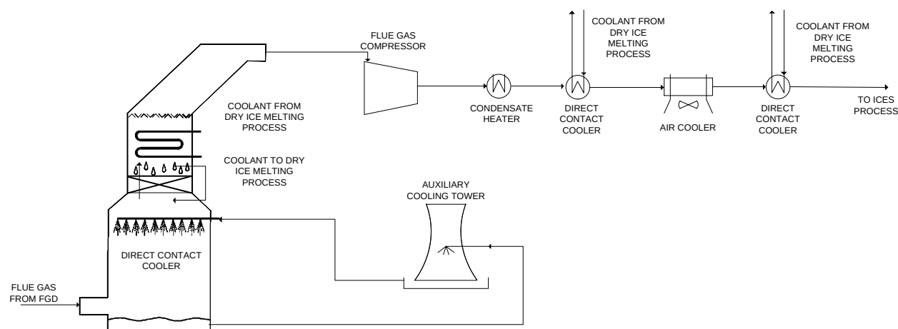
Exhibit 3-3 Flue Gas Pretreatment Option 1
