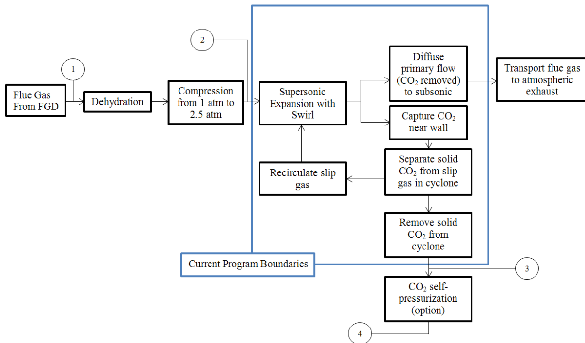
Exhibit 2-5 ICES Process Flow Diagram
