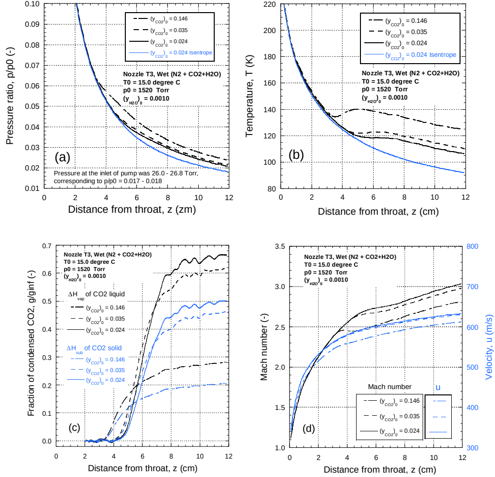
Figure 8: Heterogeneous nucleation experiments of CO_2 on H_2O in Nozzle T3. (a) The static pressure ratios, (b) temperatures, (c) fraction of CO_2 condensed, and (d) Mach number and velocity. Although the fraction of CO_2 condensed calculation shows the results for condensation of the liquid and solid, the results in Figure 7 suggest that the particles consist of solid CO_2 .
