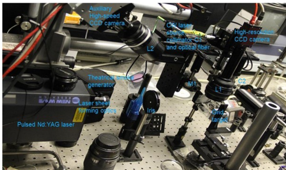
Figure 75 Particle Sizing and Real-Time Monitoring System (PS-RTM).
