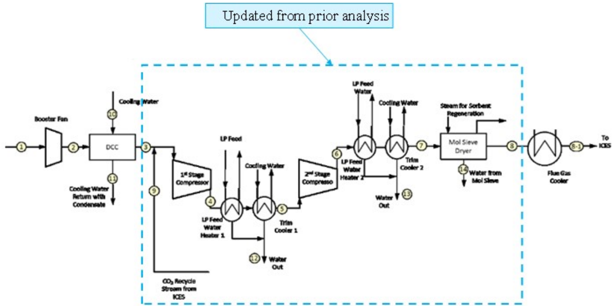
Figure 93 Details of Flue Gas Pre-treatment System
