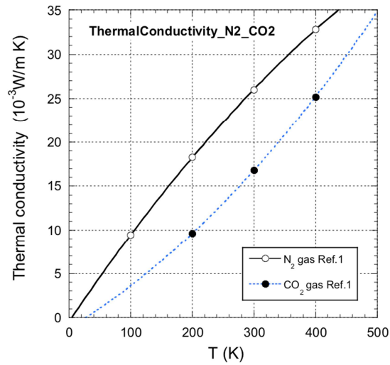
Figure A-2. The thermal conductivities of CO 2 and N 2 (Ref. 22). The dependence of thermal conductivity on pressure is negligible at pressures below 10 atm.
