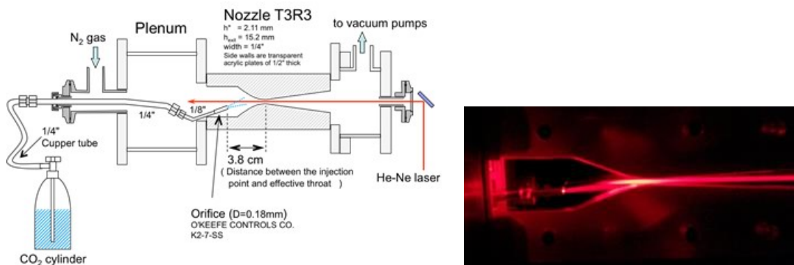
Figure 15 (left) The modified flow system includes an orifice to introduce CO 2 particles into the flow. (right) The HeNe laser illuminates the stream of particles exiting the orifice and flowing through the nozzle.
