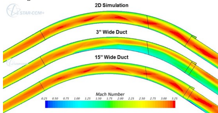
Figure 19 Comparison of centerline Mach number contours through supersonic turn for 2D (upper) and 3D 3" duct (middle) and 3D 15" duct (lower) configurations.
