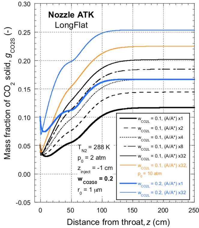
Figure 28. The mass fraction of CO 2 solid, g_{\text{CO}_2\text{s}} as a function of position in the more rapidly expanding Long Flat ATK nozzles. Conditions are indicated in the legend. The mass fraction of CO 2 in the incoming gas stream was fixed at 0.2.
