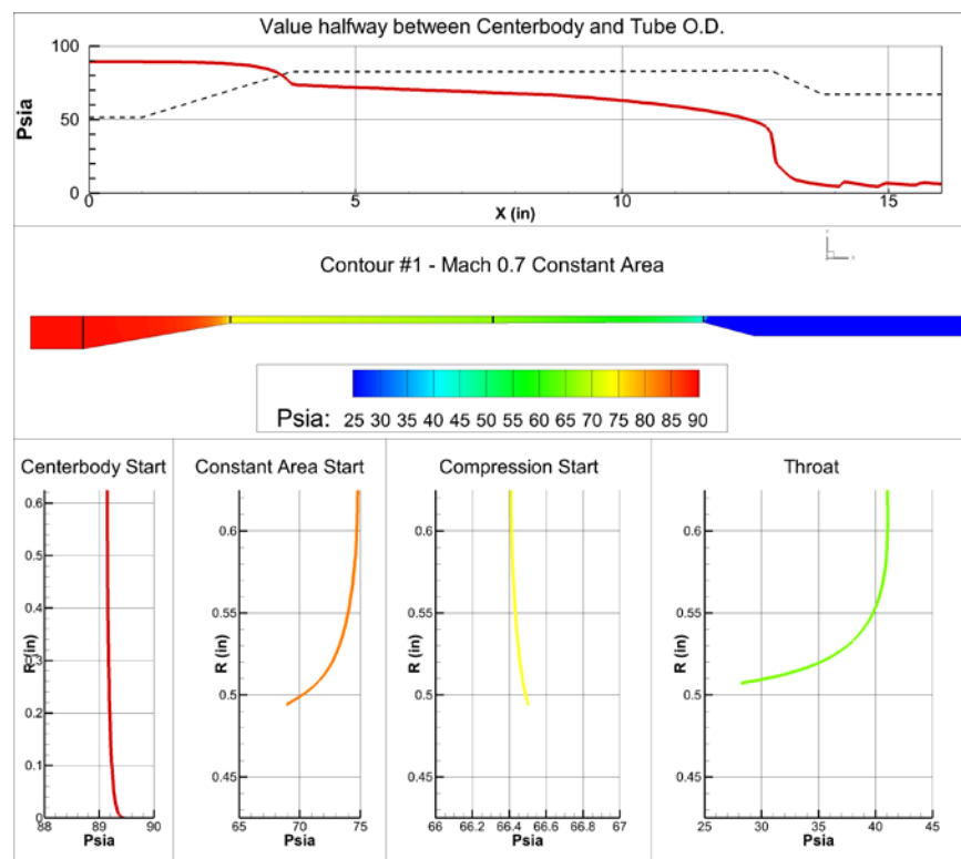
Figure 5.3.7: CFD Results for 0.988 OD Centerbody - Pressure
