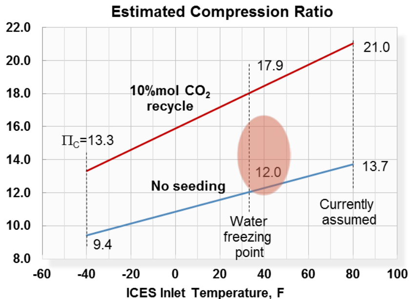
Figure 59 ICES Derived upstream compression ratio requirements
