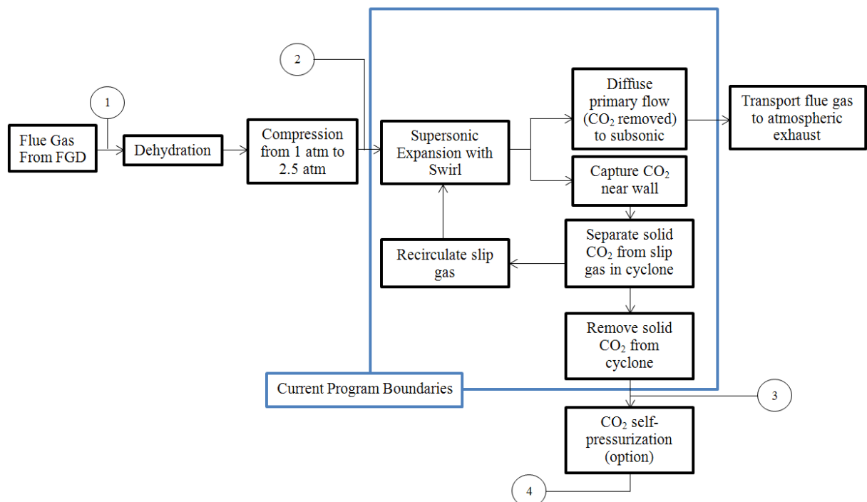
Exhibit 3-1 ICES Process Flow Diagram
