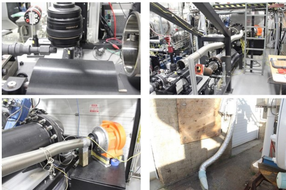
Figure 84 Updated Subsonic ICES Exhaust System
