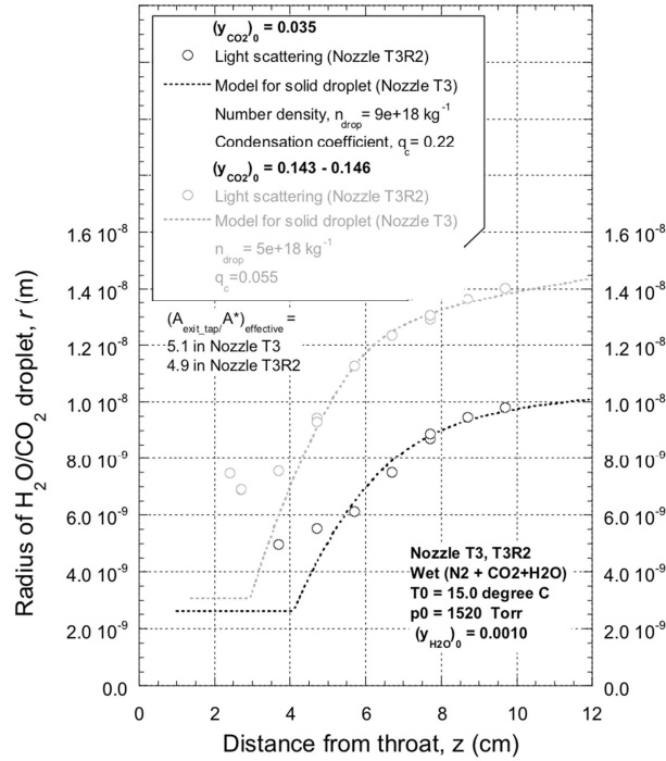
Figure 15: The size of the CO 2 particles derived LSM (circles) and model calculations (dashed lines).
