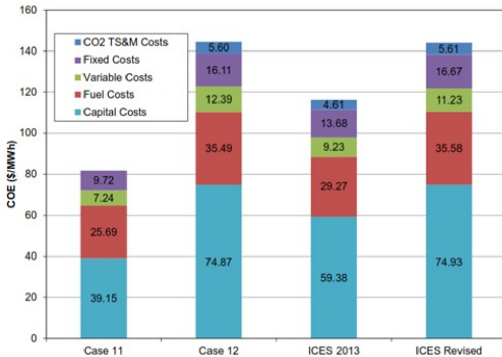
Figure 94 Summary of Economic Comparison of ICES to Case 11 and Case 12 of Bituminous Baseline Report
