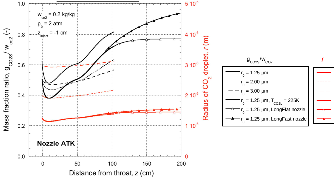
Figure 24. The mass fraction ratio and particle size predicted for the ATK nozzle as a function of the initial particle size and \text{CO}_2 liquid temperature. The default liquid temperature is 300 K. The results for two alternate nozzle shapes are also shown.
