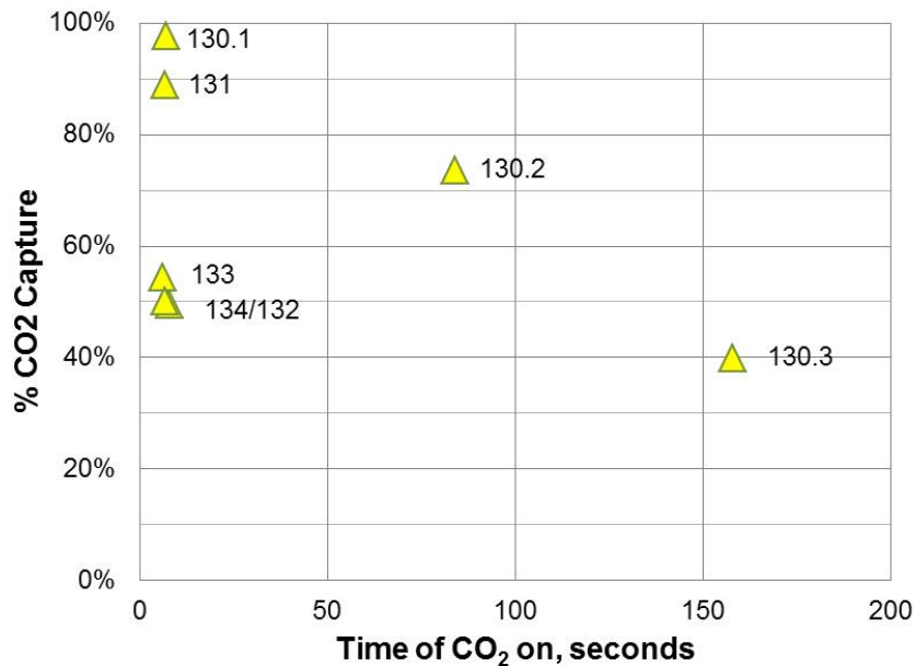
Figure 45 Bench Scale Test Results – percent CO 2 captured as a function of test run time.
