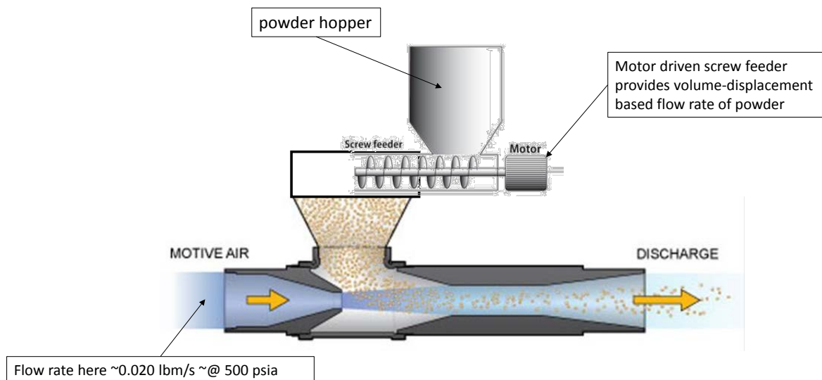
Figure 52 Powder seeder system schematic
