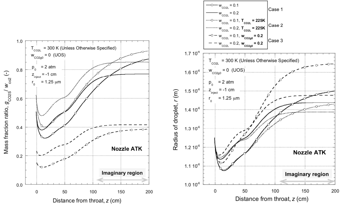
Figure 25. The mass fraction ratio (left) and particle size (right) predicted for the ATK Long Flat nozzle as a function of the initial CO_2 liquid mass fraction w_{CO_2L} , liquid temperature, and CO_2 gas mass fraction w_{CO_2g0} .
