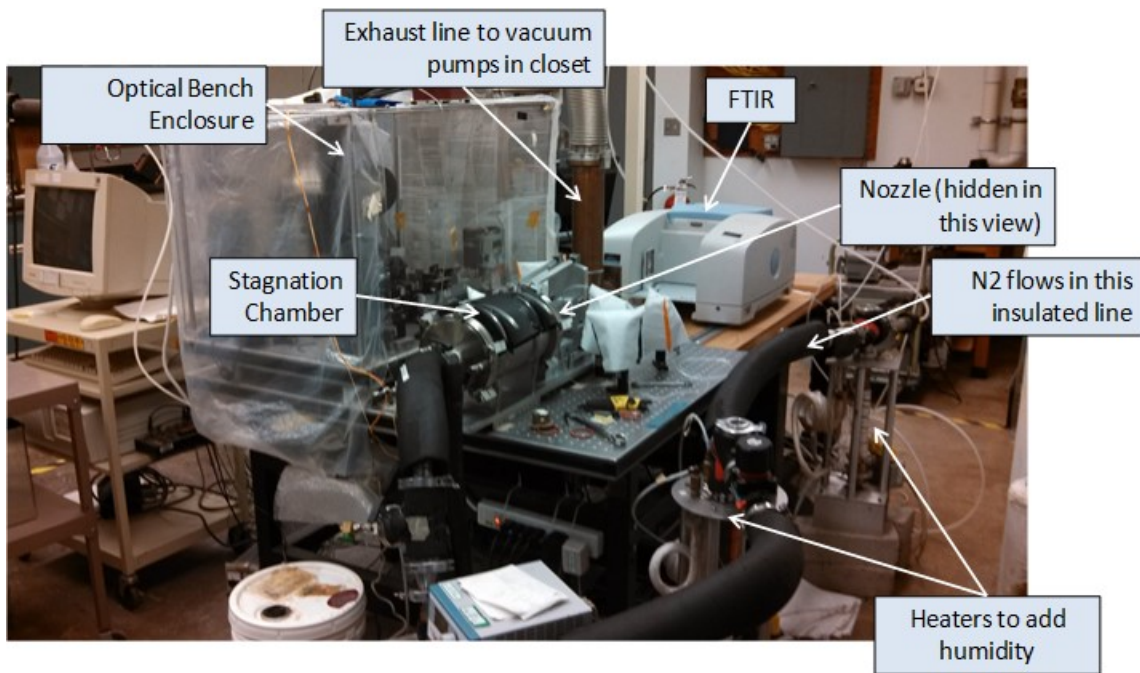
Figure 1 OSU Supersonic Aerosol Test Laboratory
