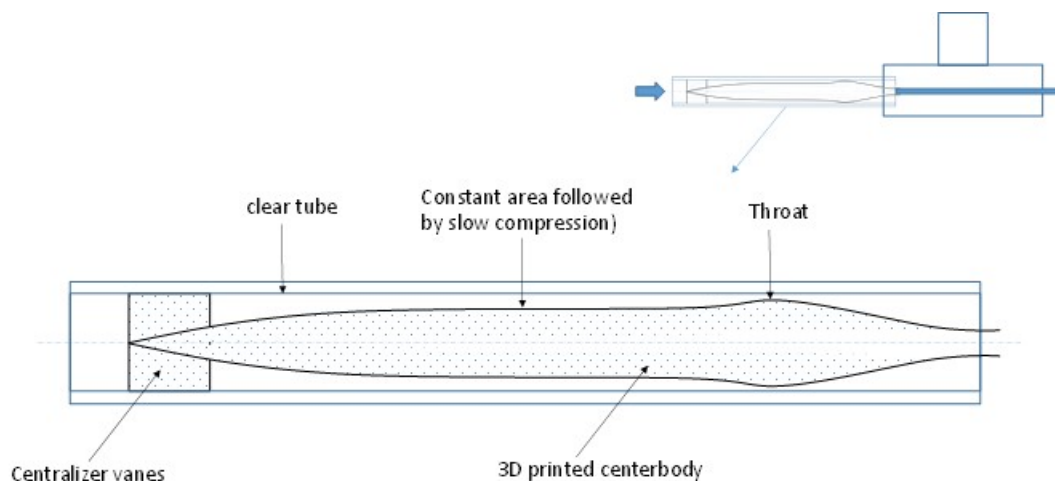
Figure 63 Conceptual Subsonic ICES Test Article
