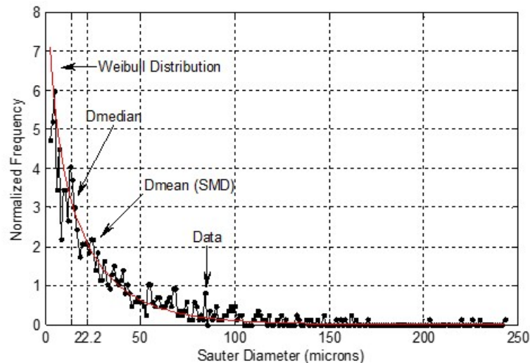
Figure 38: Histogram showing the CO 2 particle size distribution and the Weibull probability density function fit to data. Measurements taken at an axial distance of 5.0 inches downstream of a 0.023" diameter nozzle with a 6" long shroud tube.
