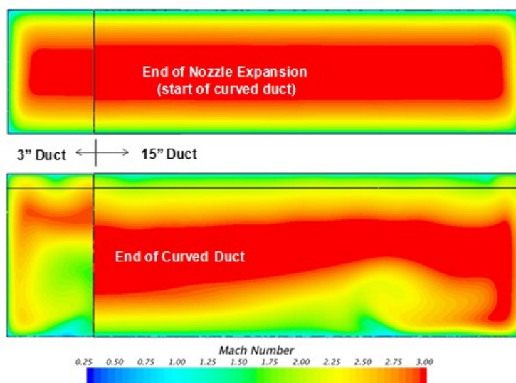
Figure 20 Comparison of Mach number contours at start and end of curved duct for current 3" wide rig (left) and 15" wide rig (right).
