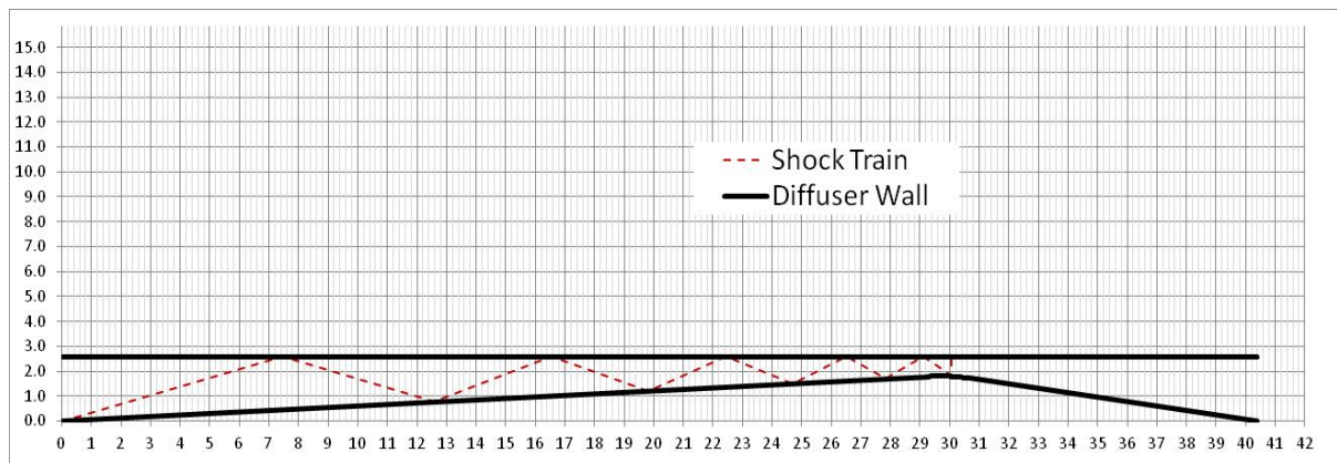
Figure 18 Initial diffuser design based on 2D supersonic wave analysis
