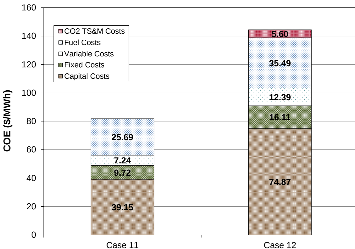
Exhibit 3-14 Comparison and Breakdown of COE for NETL/DOE Baseline Case 11 and Case 12
