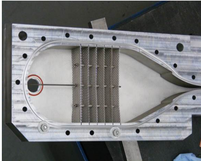
Figure 51 Current ICES plenum showing turbulence-reducing screens
