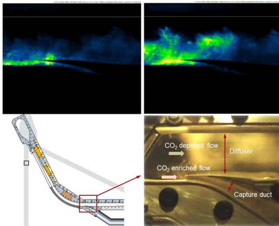
Figure 39: Laser images and photo of the capture duct entrance region.
