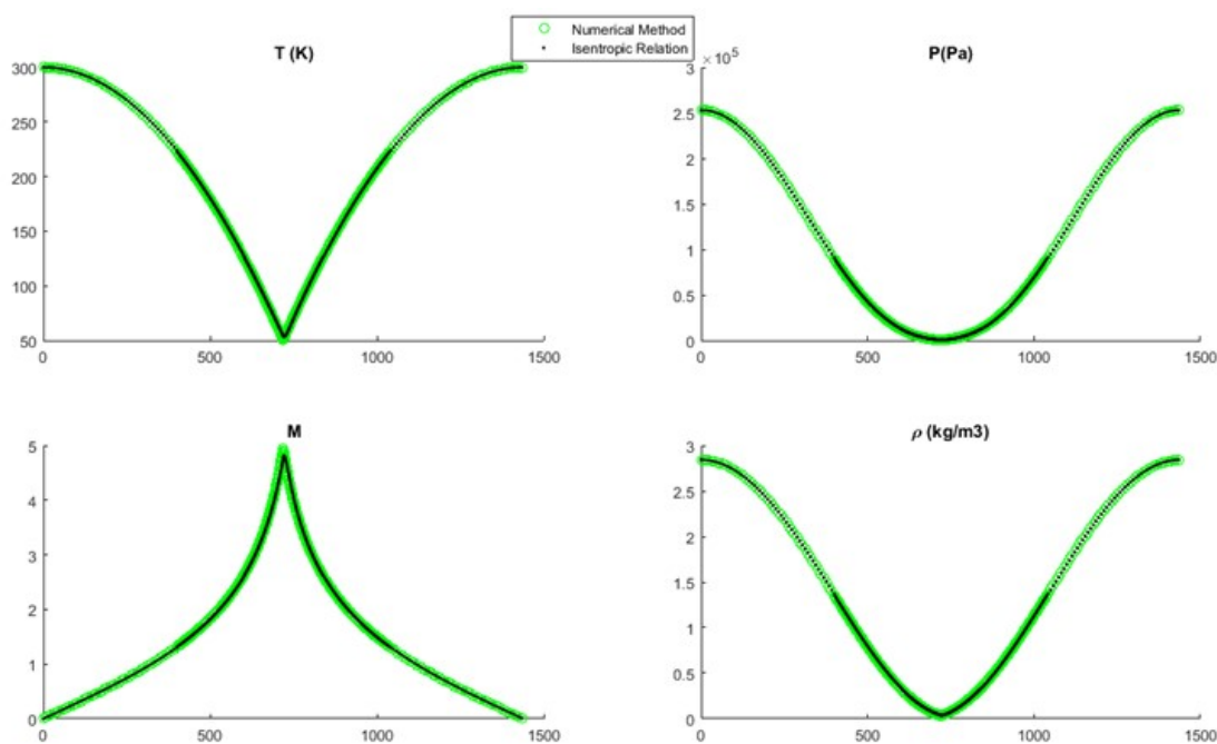
Figure 54: Numerical vs isentropic model verification for N_2
