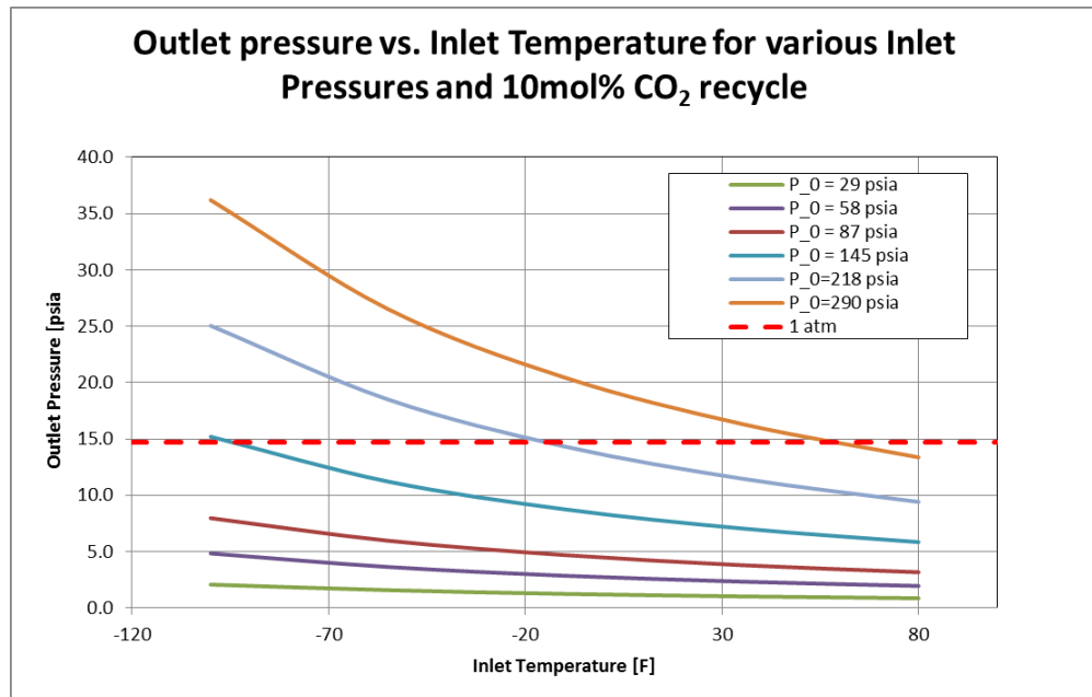
Figure 57 ICES Pressure recovery assuming 10mol% CO 2 seeding
