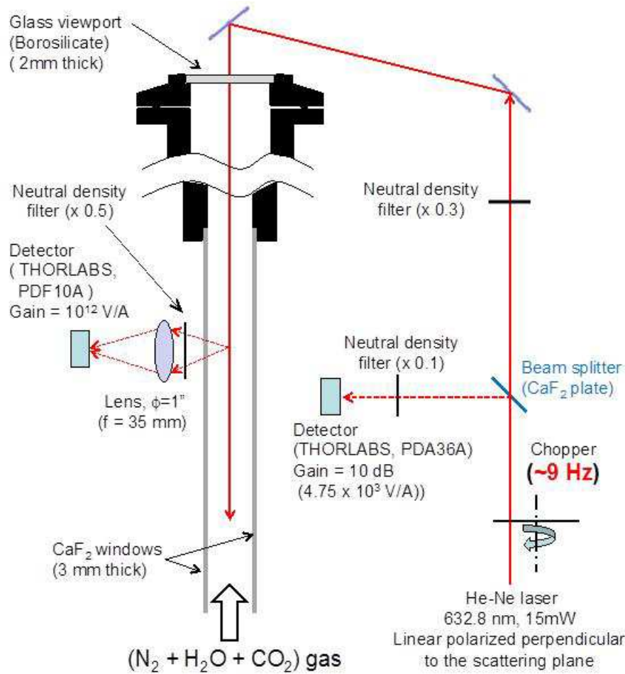
Figure 10: In the light scattering setup, the beam travels along the nozzle axis entering from the downstream end of the nozzle. Scattered light is detected at 90 degrees.
