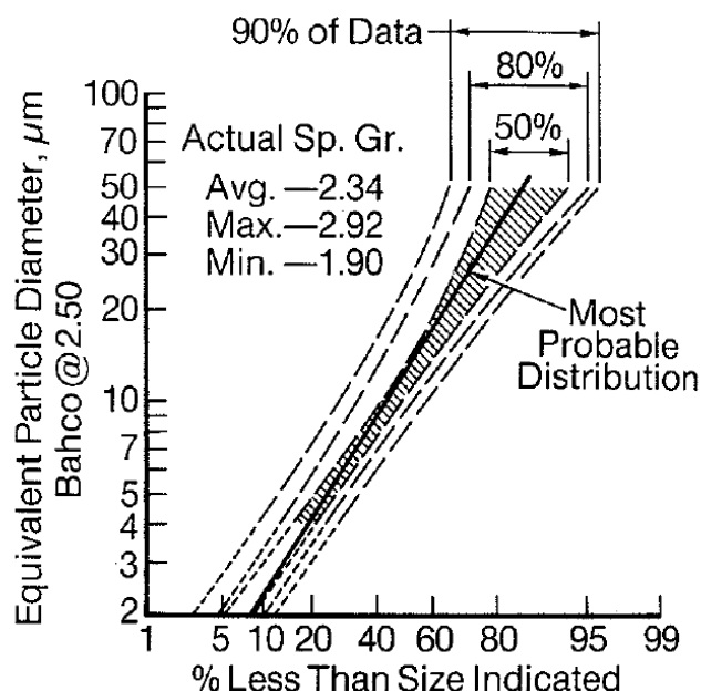
Exhibit 2-9 Flyash particle-size distribution in pulverized coal fired boilers.[7]
