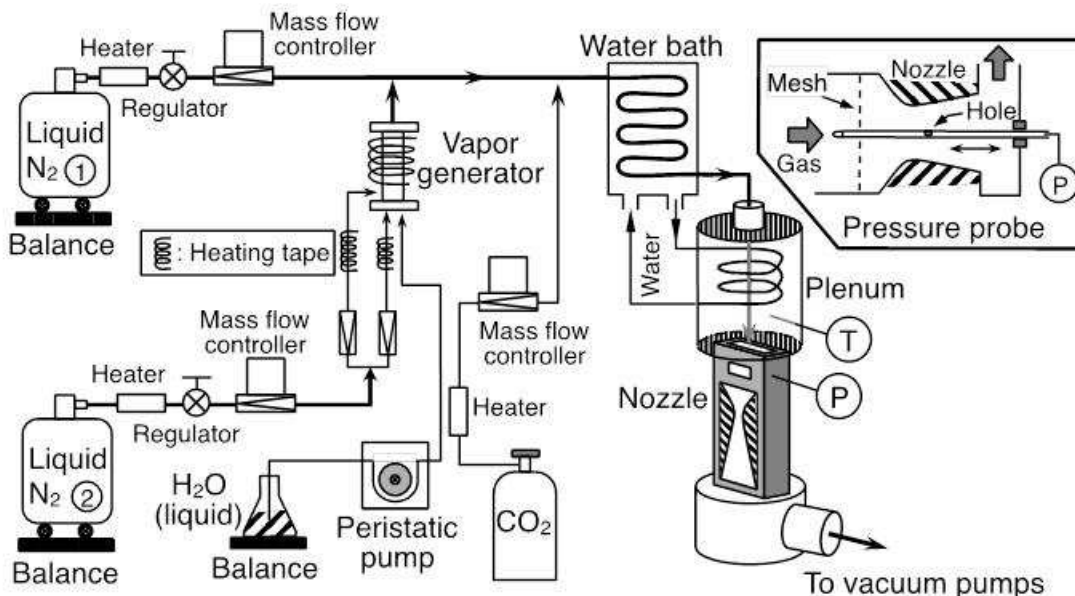
Figure 5: A schematic diagram of the experimental setup.
