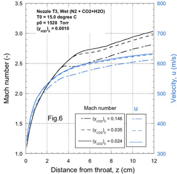
Figure 10: Mach number and velocity (u) for the heterogeneous condensation experiments.
