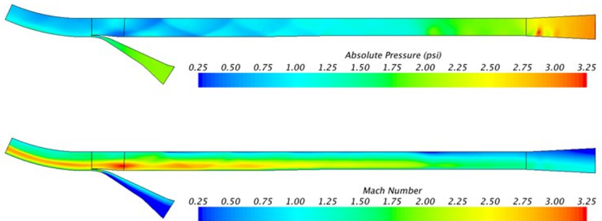
Figure 25 Pressure and Mach number results of diffuser and splitter plate/capture duct
