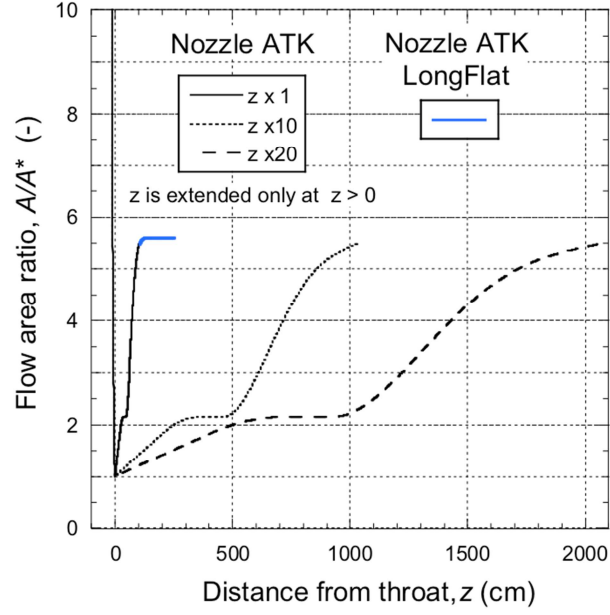
Figure 26. The nominal flow areas of the scaled ATK nozzles.
