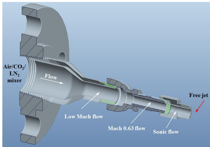
Figure 80: New configuration of the test article (subsonic ICES).
