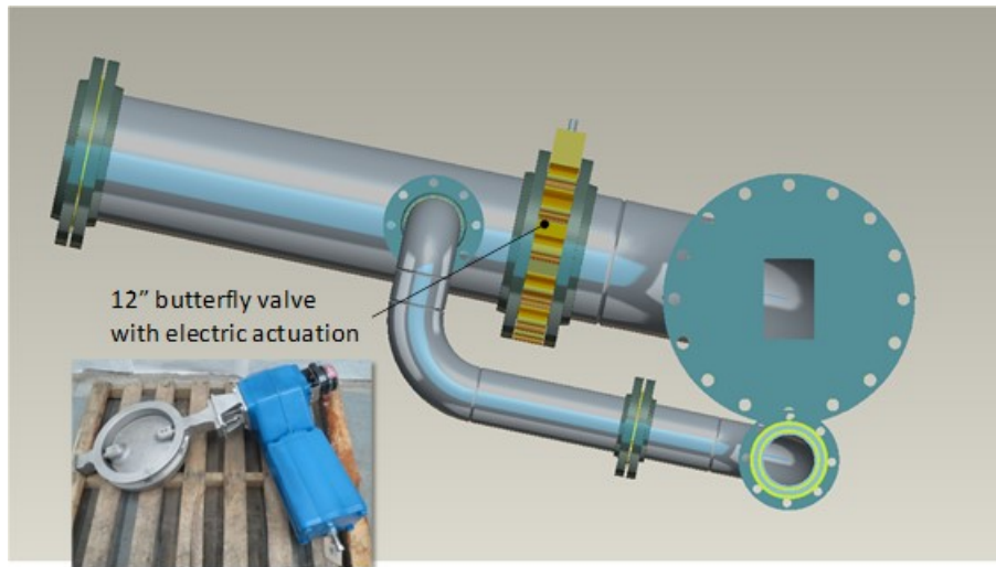
Figure 28: Exhaust system with backpressure control
