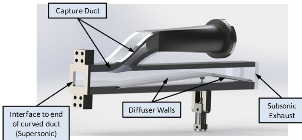
Figure 17 Preliminary capture duct and variable geometry diffuser
