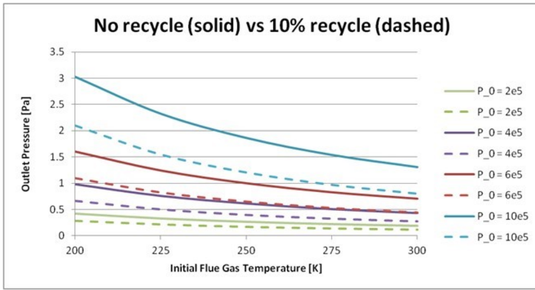
Figure 56 Effect of CO 2 recycle rate and initial temperature and pressure on diffuser outlet pressure. Outlet pressure > 1 bar required for atmospheric discharge.
