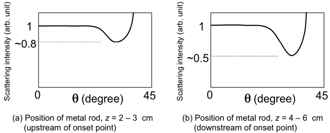
Figure 17: Qualitative light scattering intensity measured as a function of the angle of the flow perturbing rod.
