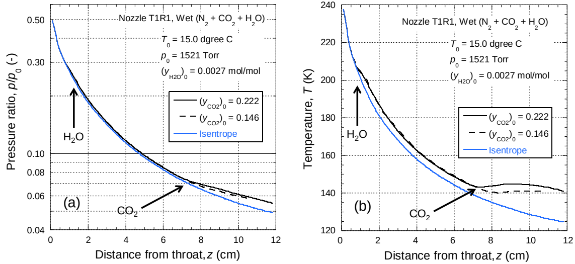
Figure 6. Heterogeneous nucleation of CO_2 on H_2O . The static pressure ratios (a) and temperatures (b) in the presence (black lines) and absence (blue line) of H_2O . The expansion is isentropic and CO_2 does not condense when H_2O is absent. The inlet concentration of water is fixed at a mole fraction of 0.0027, and the onset of water condensation is indicated by the leftmost arrow in the pressure/temperature plots. The onset of CO_2 condensation (right arrow) moves to higher pressure and temperature as the mole fraction of CO_2 ( y_{CO_2,0} ) increases, but always occurs at temperatures significantly colder than those required for the condensation of water.
