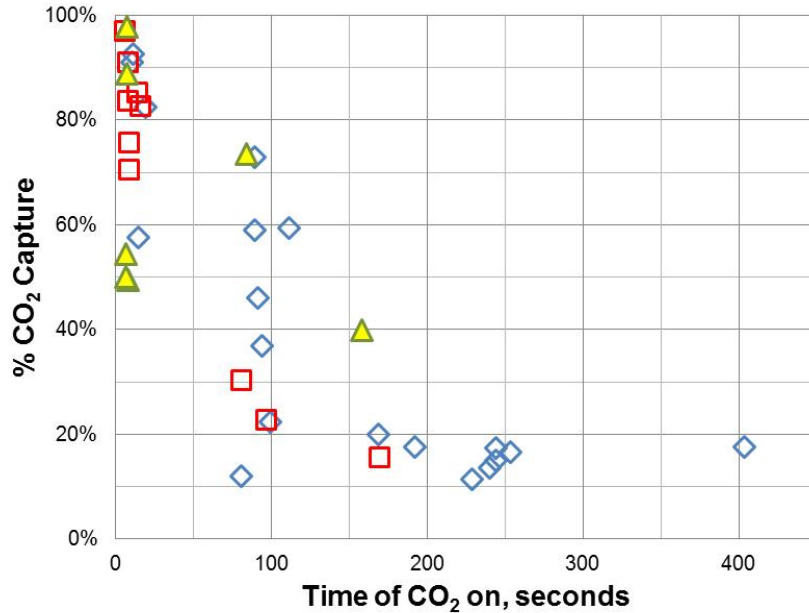
Figure 44 Bench Scale Test Results – percent CO 2 captured as a function of test run time.
