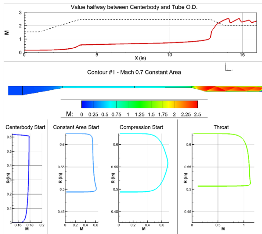
Figure 68 CFD Results for 0.988 OD Centerbody – Mach Number
