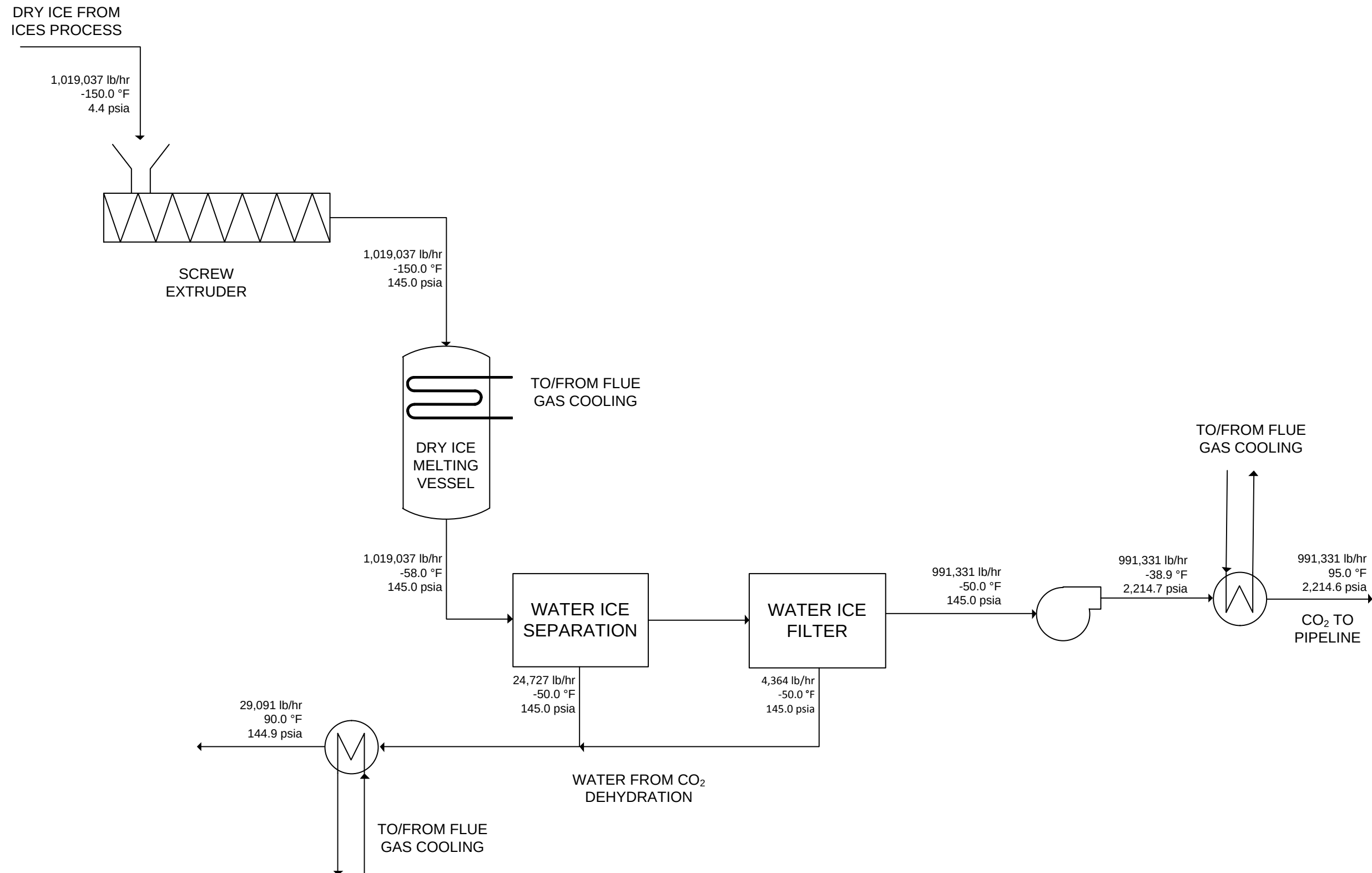
Exhibit 4-7 Heat and Mass Balance Details for Dry Ice Melting Equipment
