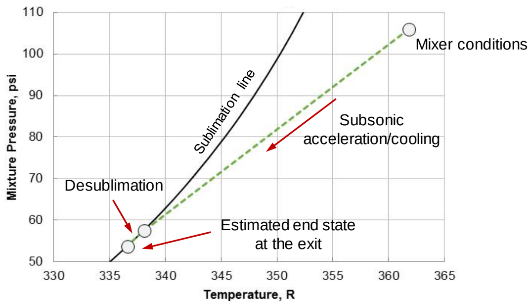
Figure 82 CO 2 sublimation and condensation lines in P-T diagram.
