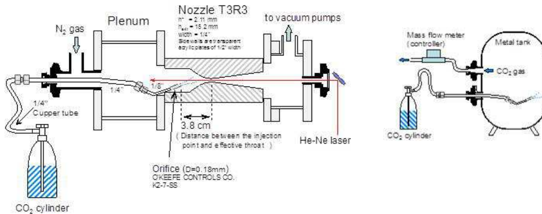
Figure 18: (left) OSU experimental setup for CO 2 injection into the nozzle. (right) The CO 2 flow calibration setup.
