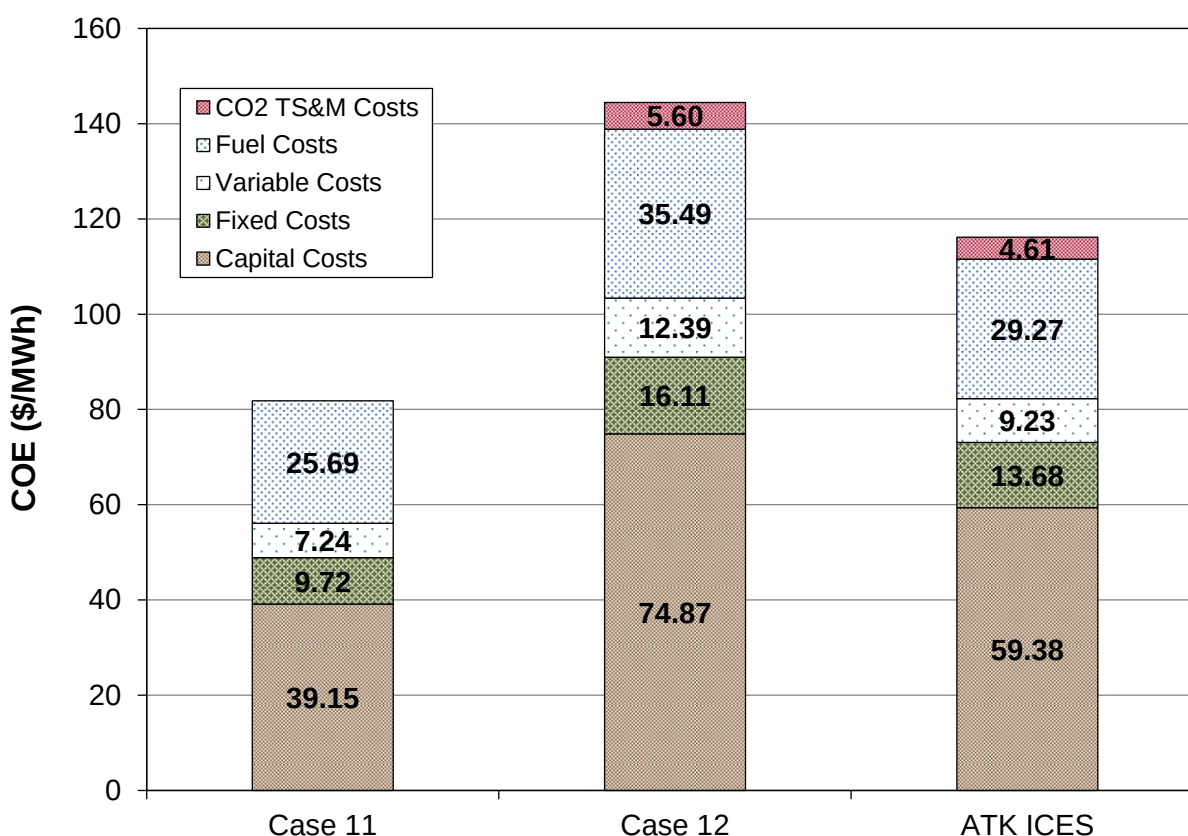
Exhibit 4-16 Comparison and Breakdown of COE for the DOE/NETL Baseline Cases and the ATK ICES Case
