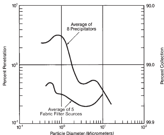
Exhibit 2-10 Particle Penetration of Fabric Filters as a Function of Particle Size.[8]
