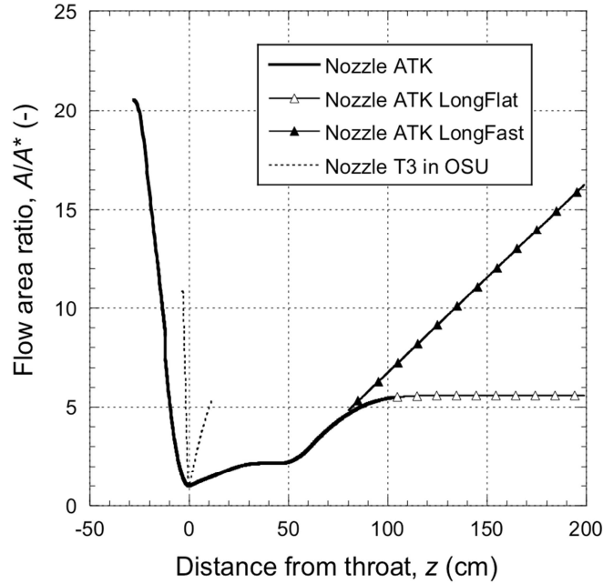
Figure 23. The nominal flow area ratios of the ATK nozzle and the two modified versions.
