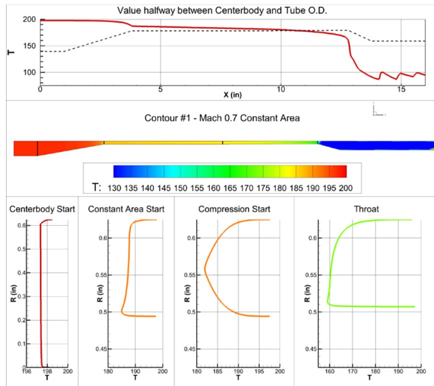
Figure 67 : CFD Results for 0.988 OD Centerbody - Temperature
