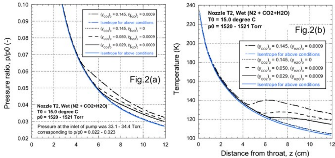
Figure 6 The (a) pressure profiles and (b) temperature profiles as mixtures of N 2 + 0.09 mol% H 2 O and 3 different CO 2 concentrations flow through nozzle T2. CO 2 condensation occurs for all cases in which water is present. In contrast, when a mixture of N 2 + 14.5 mol% CO 2 flows through the nozzle there is no condensation even at temperatures approaching 100 K.
