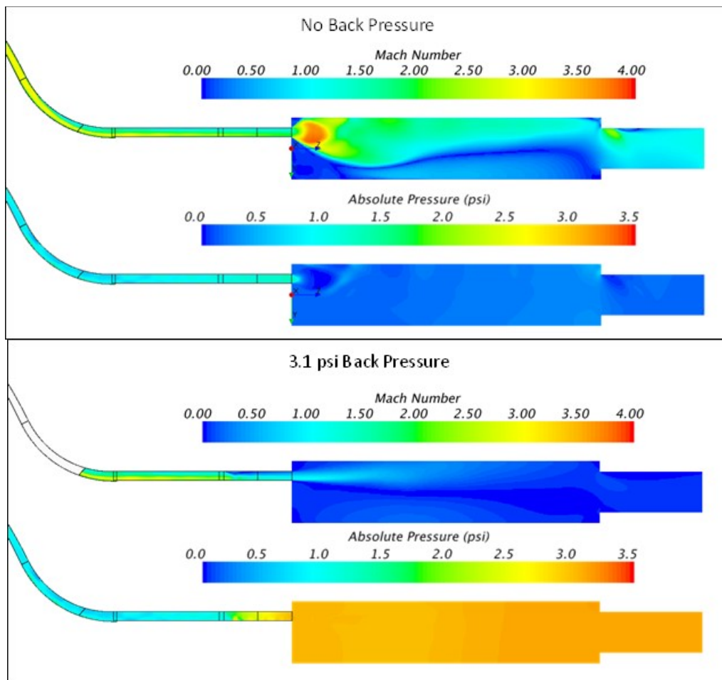
Figure 24 CFD results of ICES vacuum path
