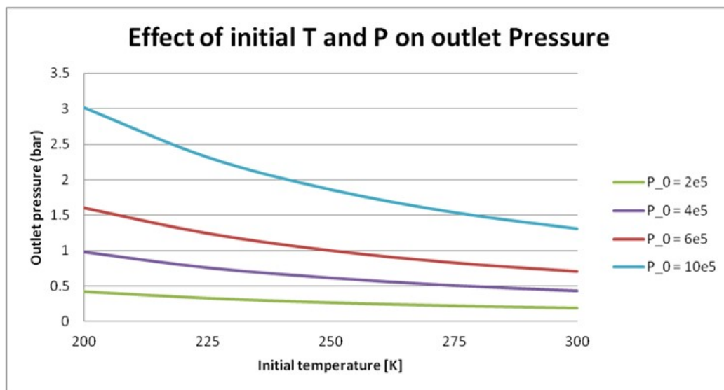
Figure 55 Effect of initial temperature and pressure on diffuser outlet pressure. Outlet pressure > 1 bar required for atmospheric discharge.
