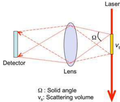
Figure 11: Geometric constraints determine the amount of light reaching the detector.
