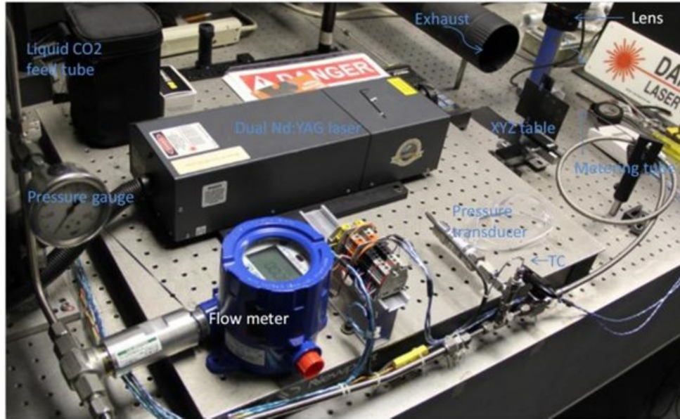
Figure 34: CO 2 Particle Size Test Bench
