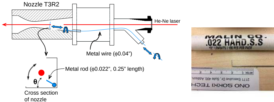
Figure 16: The experimental setup for the flow perturbation experiments.
