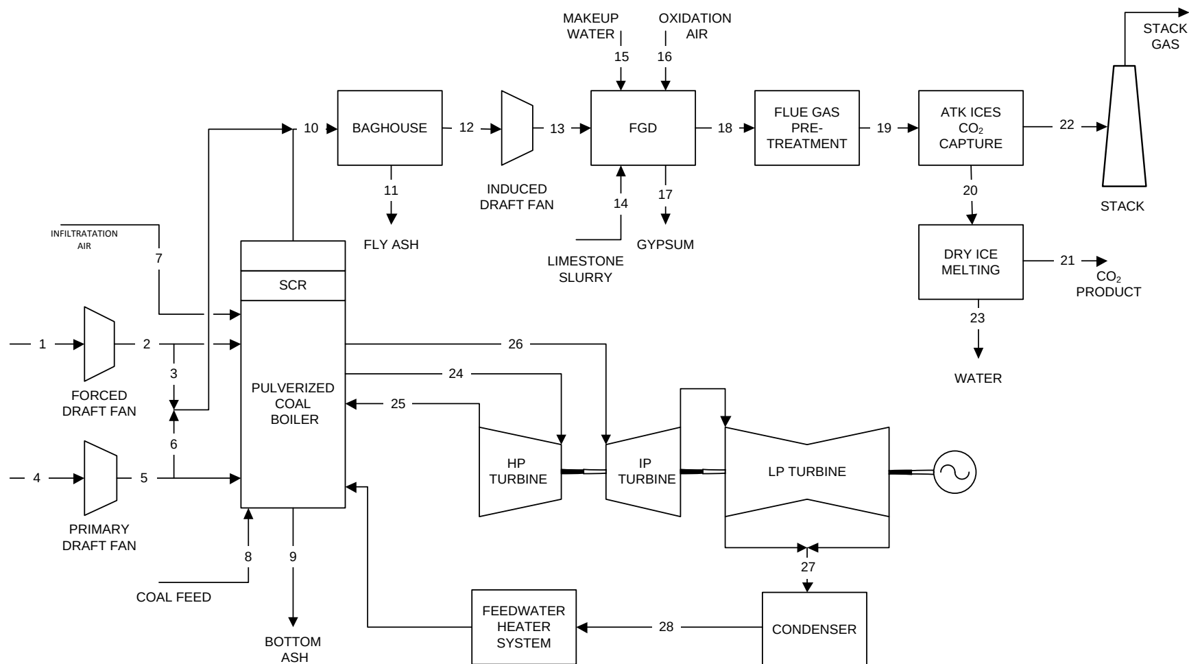
Exhibit 4-2 ATK ICES Case Block Flow Diagram, Supercritical Unit with CO 2 Capture
