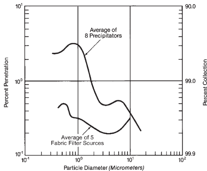
Exhibit 3-6 Particle Penetration of Fabric Filters as a Function of Particle Size.[8]
