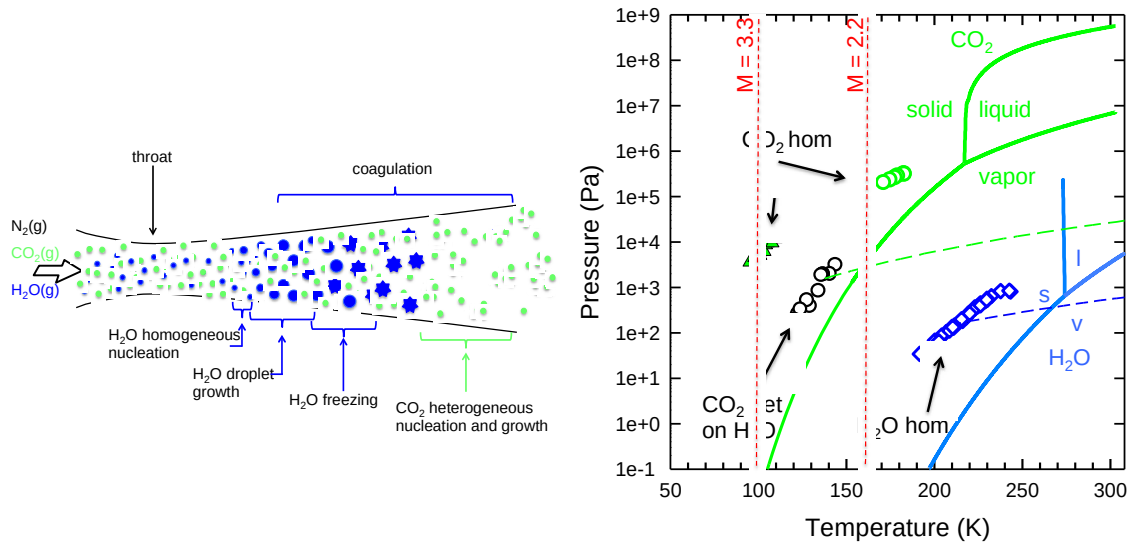
Figure 4: Heterogeneous nucleation in a supersonic nozzle. (left) As water vapor and CO 2 flow through a supersonic nozzle, water condenses and freezes at temperatures well above the sublimation temperature for CO 2 . Further cooling of the flow initiates heterogeneous nucleation of CO 2 onto the frozen water droplets. (right) On a combined phase diagram for CO 2 (green) and H 2 O (blue), the solid lines indicate the equilibrium phase boundaries for the solid, liquid and vapor regions. The conditions corresponding to the homogeneous nucleation of water 6 and CO 2 in supersonic flows are indicated by the blue and green symbols. The circles are from Duff 3 and the triangles are our estimates based on the theory corresponding states. 7 The black symbols are our very recent measurements for the onset of heterogeneous nucleation of CO 2 on water particles. The dashed lines trace the p - T history of CO 2 (green) and H 2 O (blue) as a mixture (14.5% CO 2 , 0.75% H 2 O, balance N 2 ) containing these species expands across the nozzle from T_0 = 308 K and p_0 = 2 atm. The red vertical lines correspond to the indicated Mach numbers. Water condenses when the blue dashed line intersects the blue diamonds. CO 2 condenses heterogeneously when the green dashed line intersects the black circles. To our knowledge these are the first deliberate and well characterized heterogeneous nucleation experiments conducted in a supersonic nozzle.
