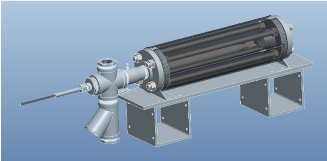
Figure 71: Subsonic ICES Test Article Assembly
