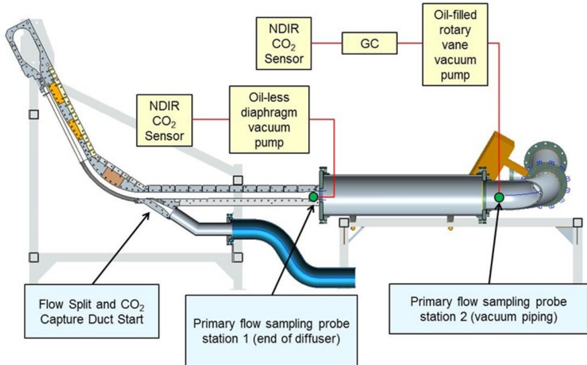
Figure 46 Gas sampling arrangement in the last test series.
