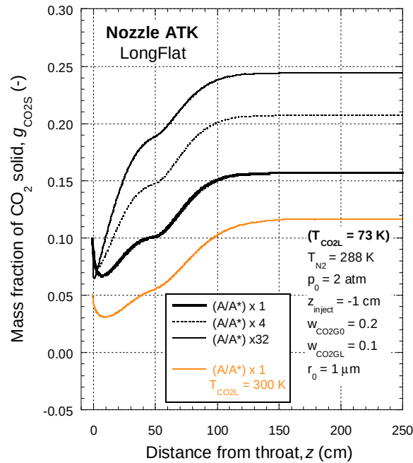
Figure 29. The mass fraction of CO 2 solid, g_{CO2s} as a function of position in the more rapidly expanding Long Flat ATK nozzles. Conditions are indicated in the legend. The orange line corresponds to Case 3.
