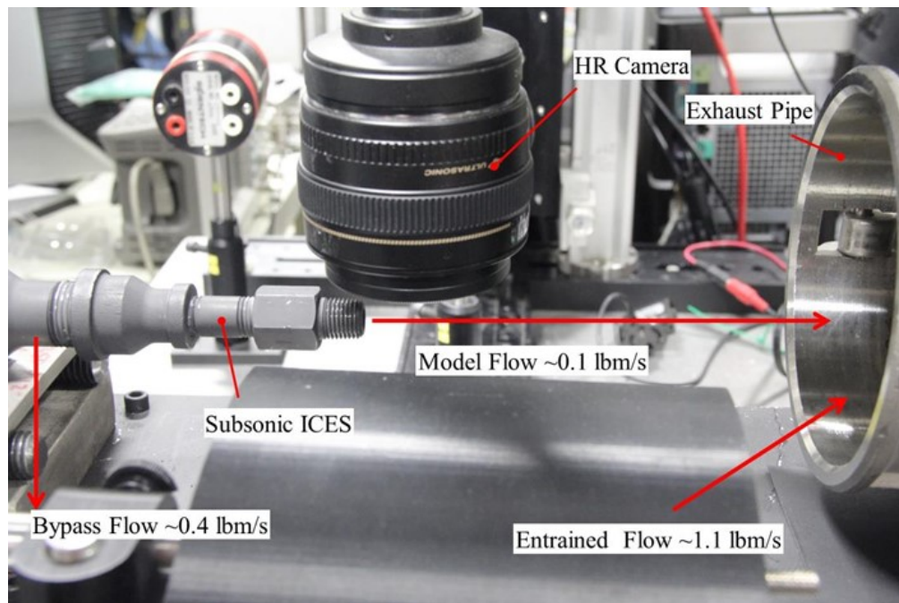
Figure 83 Major Components of the Updated Subsonic ICES Rig with Flow Splits
