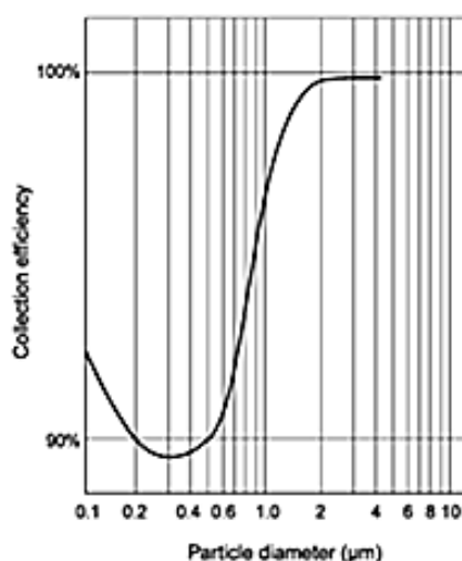
Exhibit 2-12 Collection Efficiency of wet FGD as a Function of Particle Size[7].
