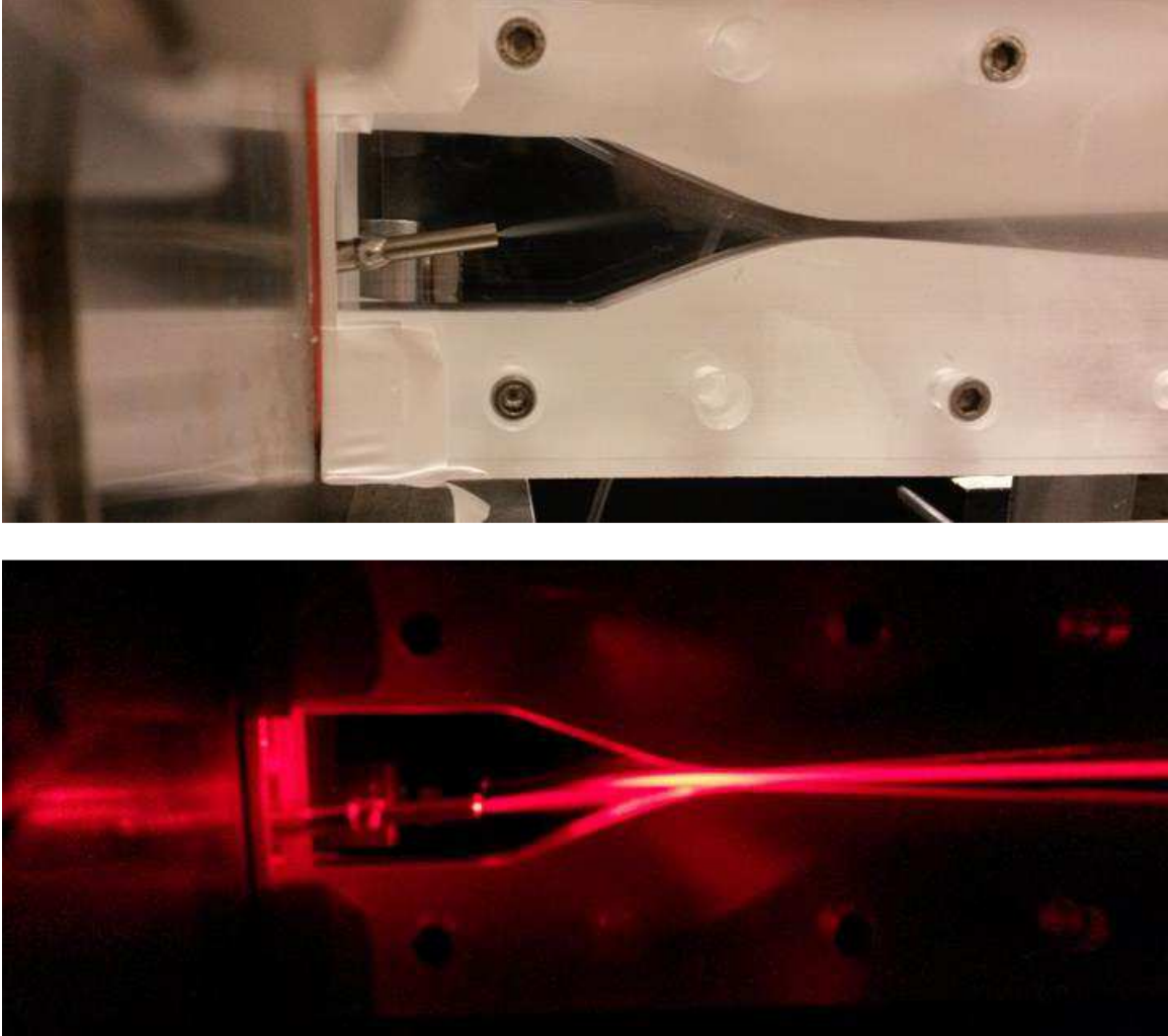
Figure 19. (top) The CO 2 injector nozzle integrated into Nozzle T3. (bottom) Light scattering confirms the presence of particles far downstream of the injection point.
