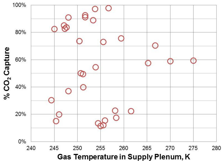
Figure 41 Bench Scale Test Results – percent CO 2 captured as a function of incoming temperature
