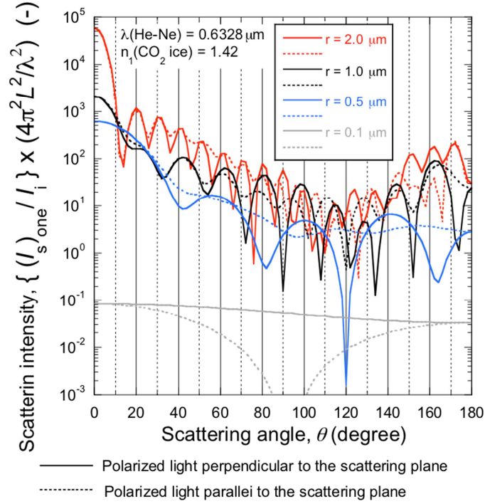
Figure 21: Scattering intensity from micron sized particles is calculated using Mie theory for the noted wavelength and index of refraction.
