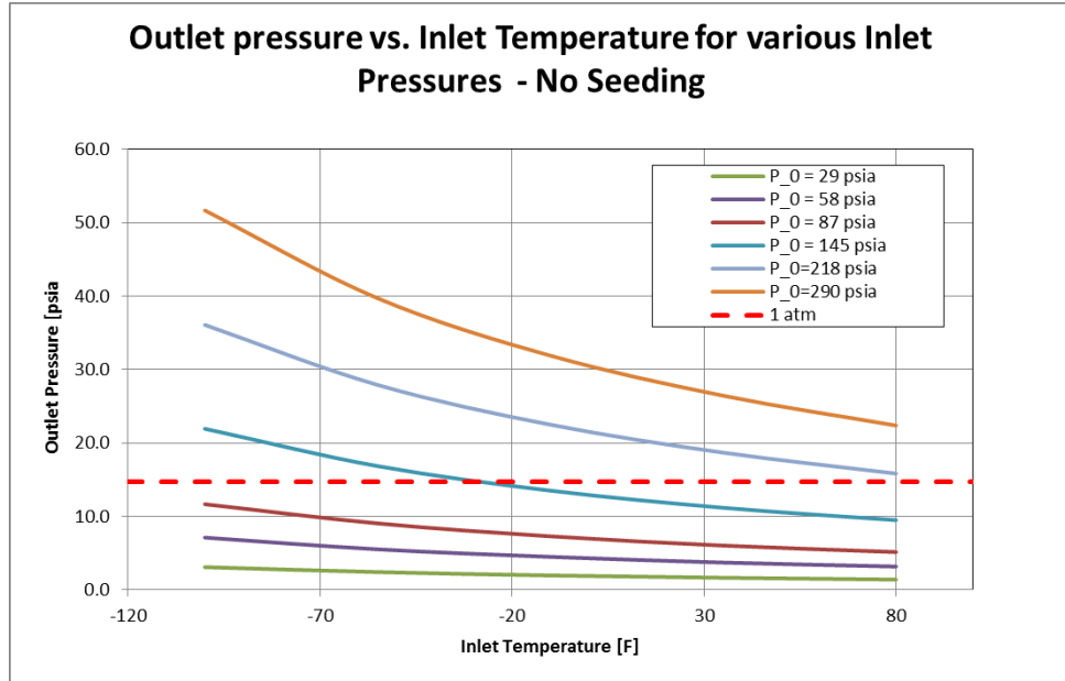
Figure 58 ICES Pressure recovery assuming no seeding
