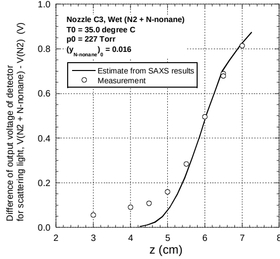
Figure 12: The difference in voltage between the experiments in which nonane is condensing and the dry trace. The symbols are the experimental values the black line is estimated based on the calibration factor established for water and the SAXS measurements.
