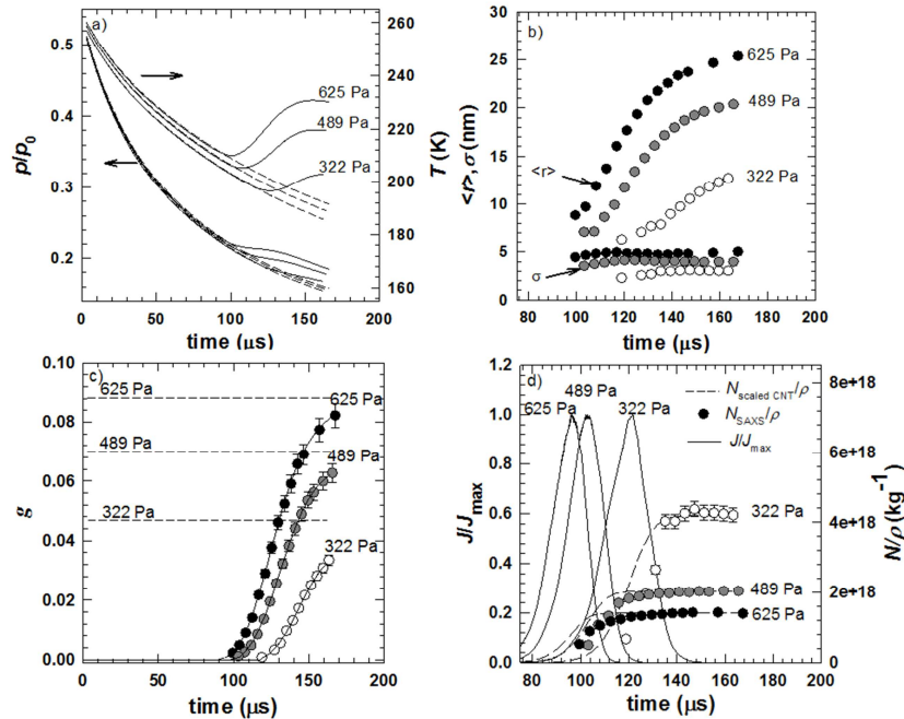
Figure 2. Position resolved measurements of nonane condensation in a supersonic nozzle.
