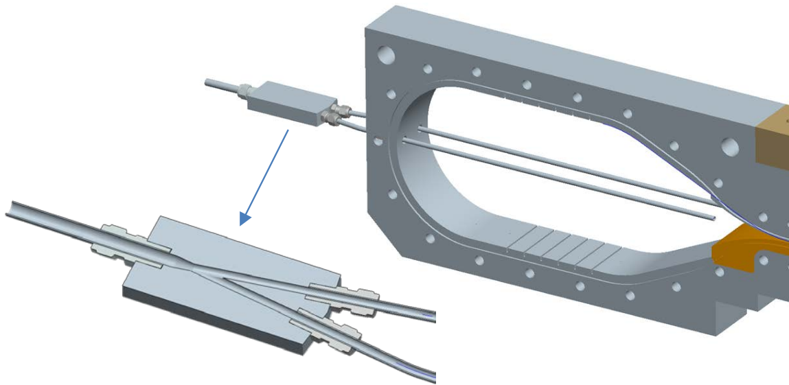
Figure 50 Powder seeder tubing in ICES plenum
