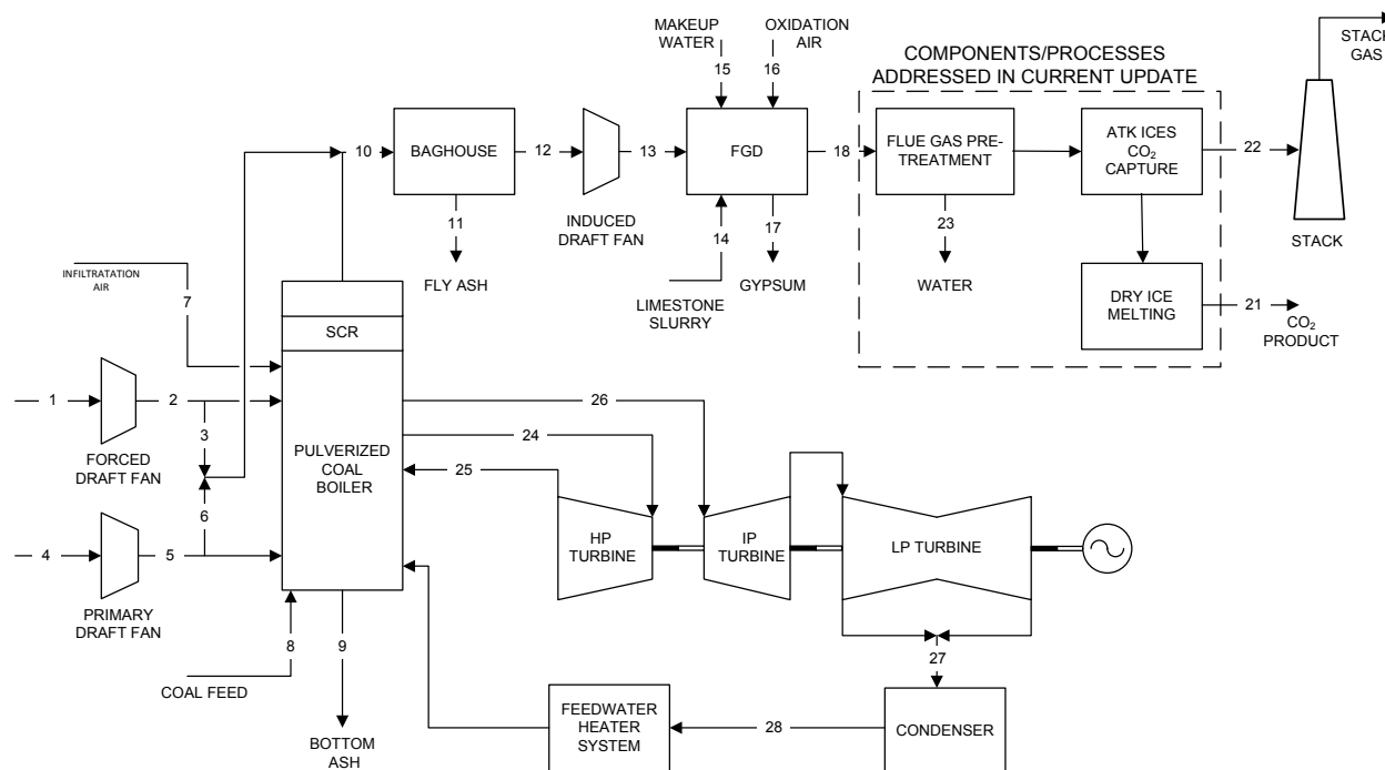
Figure 2-2 Block Flow Diagram of the Power Plant Equipped with modified ICES system
