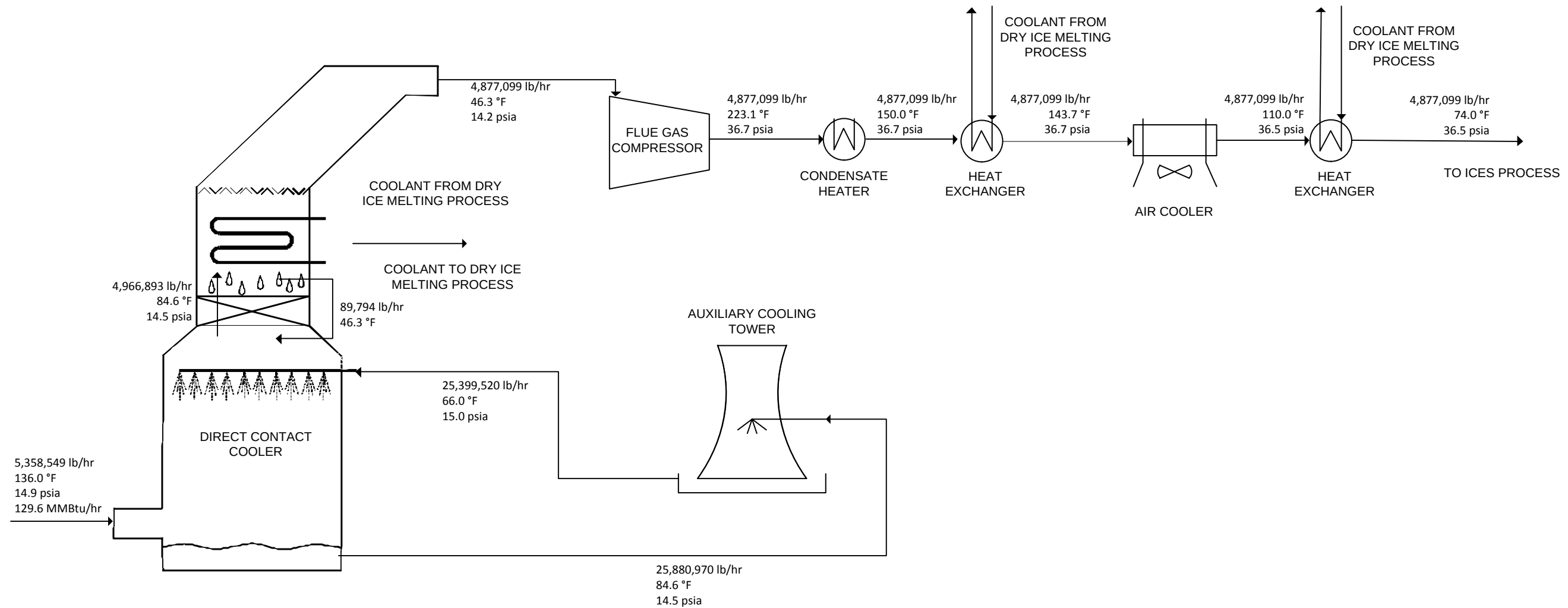
Exhibit 4-6 Heat and Mass Balance Details for Flue Gas Pretreatment Equipment
