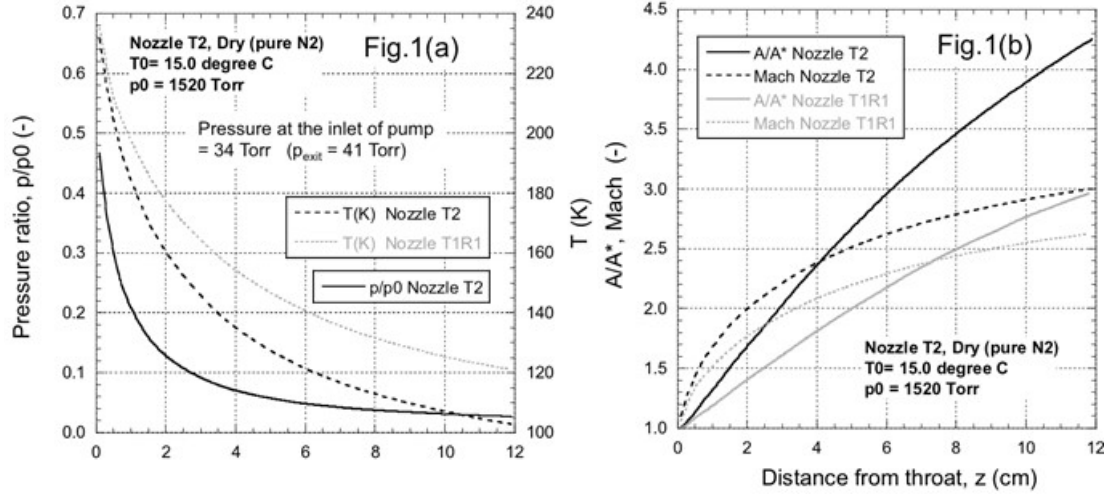
Figure 5 (a) The measured pressure profile for T2 and the derived temperature profiles for T2 and T1R1 as N 2 flows through the nozzle from T_0 = 15 C. The stagnation pressure p_0 = 1520 Torr and the exit pressure is 41 Torr. The exit temperature reaches \sim 102 K. (b) In nozzle T2 the effective area ratio at the nozzle exit is \sim 4.3 , and the Mach number approaches 3. The data for nozzle T1R1 is also shown.
