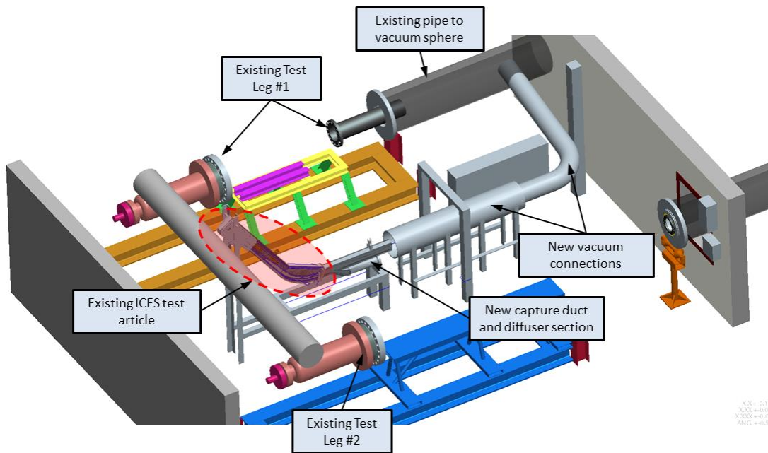
Figure 26 CAD rendering of ICES test article integrated between Orbital ATK Test Leg #1 and #2
