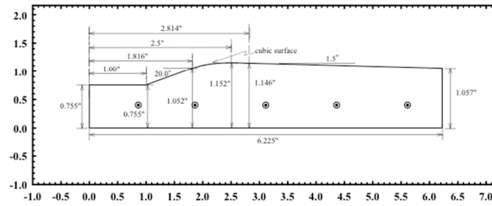
Figure 1. The profile of the nozzle used in the D2O-nonane condensation experiments.
