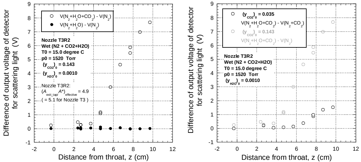
Figure 13: (left) The difference in voltage between the experiments in which H 2 O alone (filled circles) or CO 2 + H 2 O (open circles) are condensing and the dry trace. (right) The difference in voltage between the experiments in which CO 2 + H 2 O (open circles) are condensing and the dry trace – either N 2 or N 2 +CO 2 - for the experiments with y_{CO_2} = 0.035 (dark) and those for y_{CO_2} = 0.143 (light).
