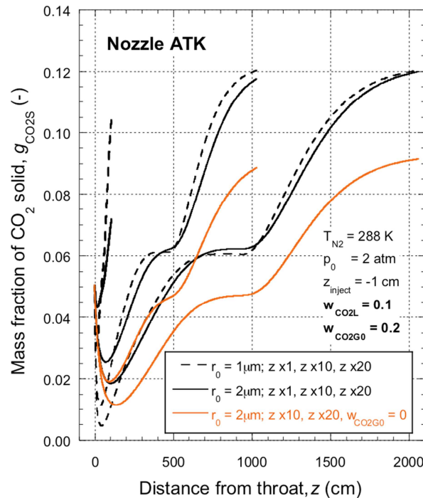
Figure 27. The mass fraction of \text{CO}_2 solid as a function of position in the scaled ATK nozzles. Conditions correspond to Case 3 (black lines) and Case 1 (orange lines).
