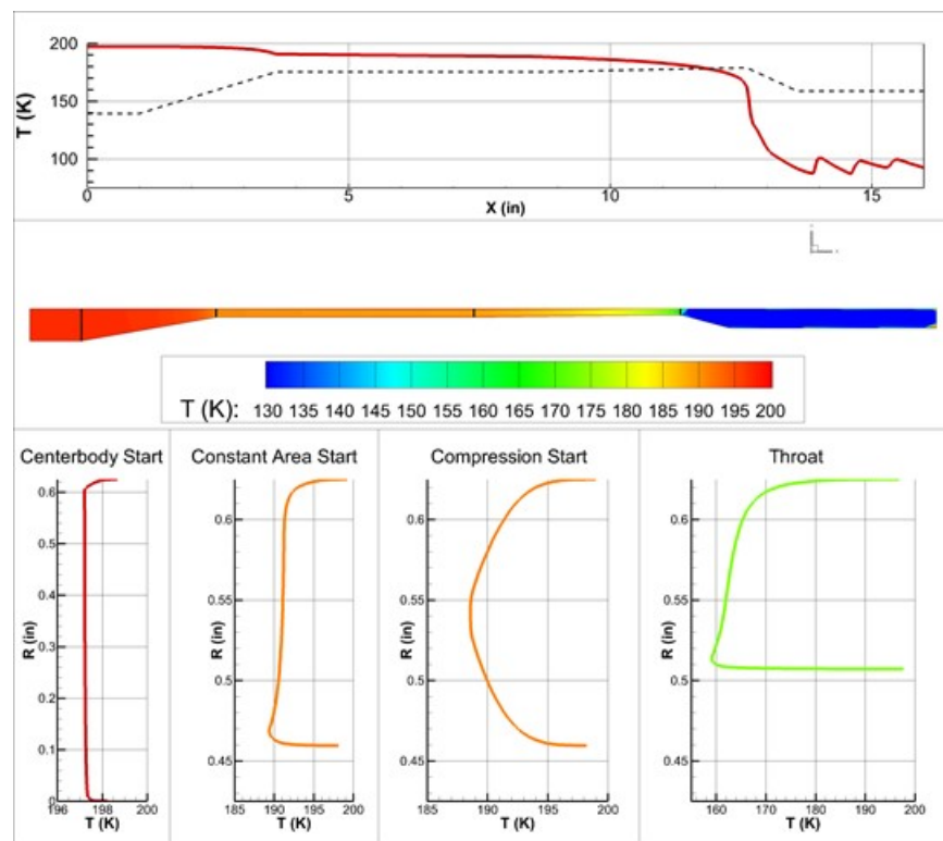
Figure 65 CFD Results for 0.919 OD Centerbody - Temperature
