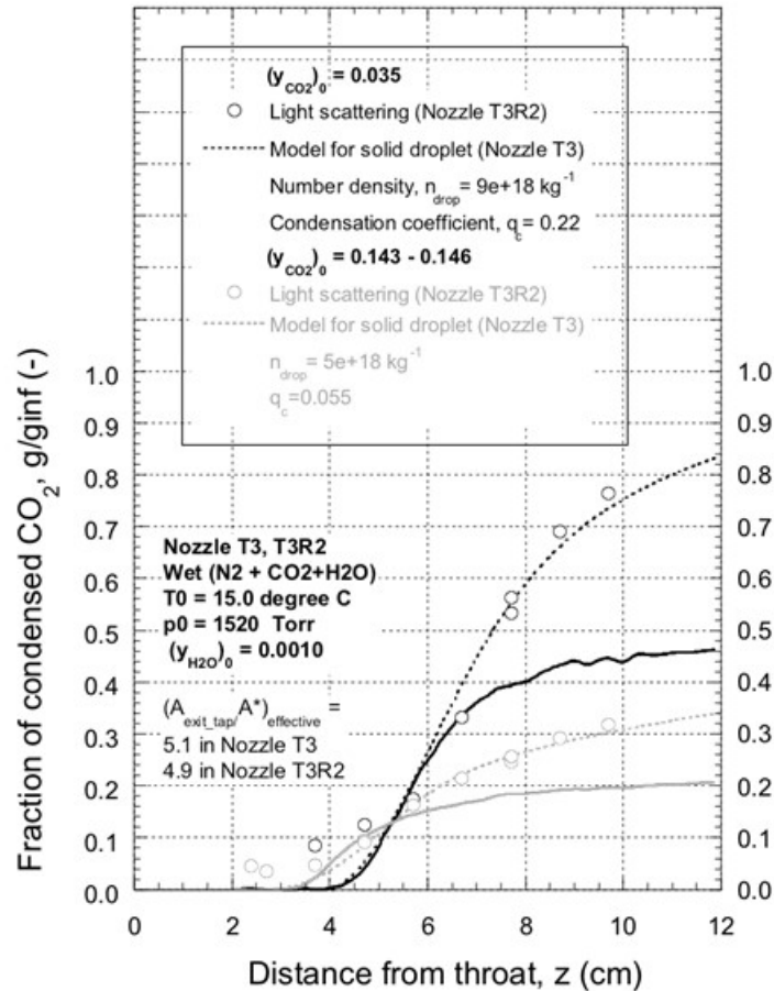
Figure 13 The fraction of CO 2 condensed that was derived from pressure trace measurement (PTM, solid black line), light scattering measurement (LSM, open circles), and model calculations (dashed line)
