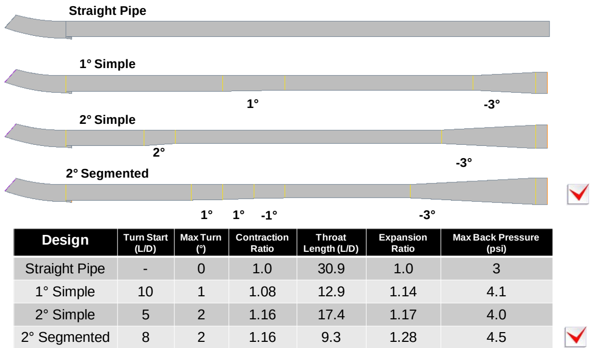
Figure 23: Fixed geometry diffuser and backpressure summary
