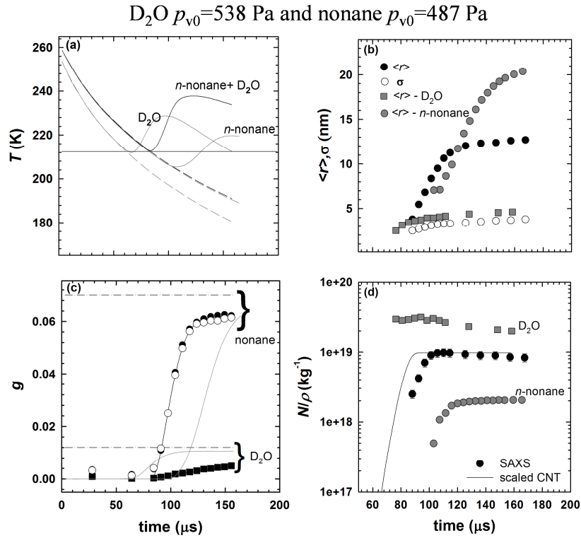
Figure 3. Position resolved measurements of nonane-D 2 O co-condensation in a supersonic nozzle.
