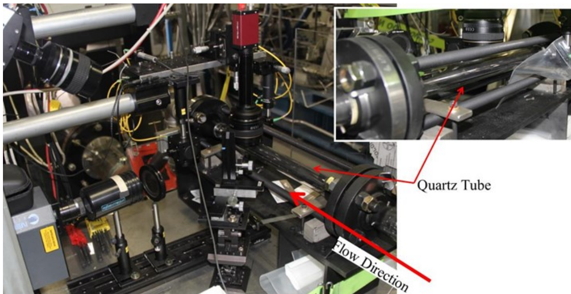
Figure 73: Initial Subsonic ICES Test Configuration
