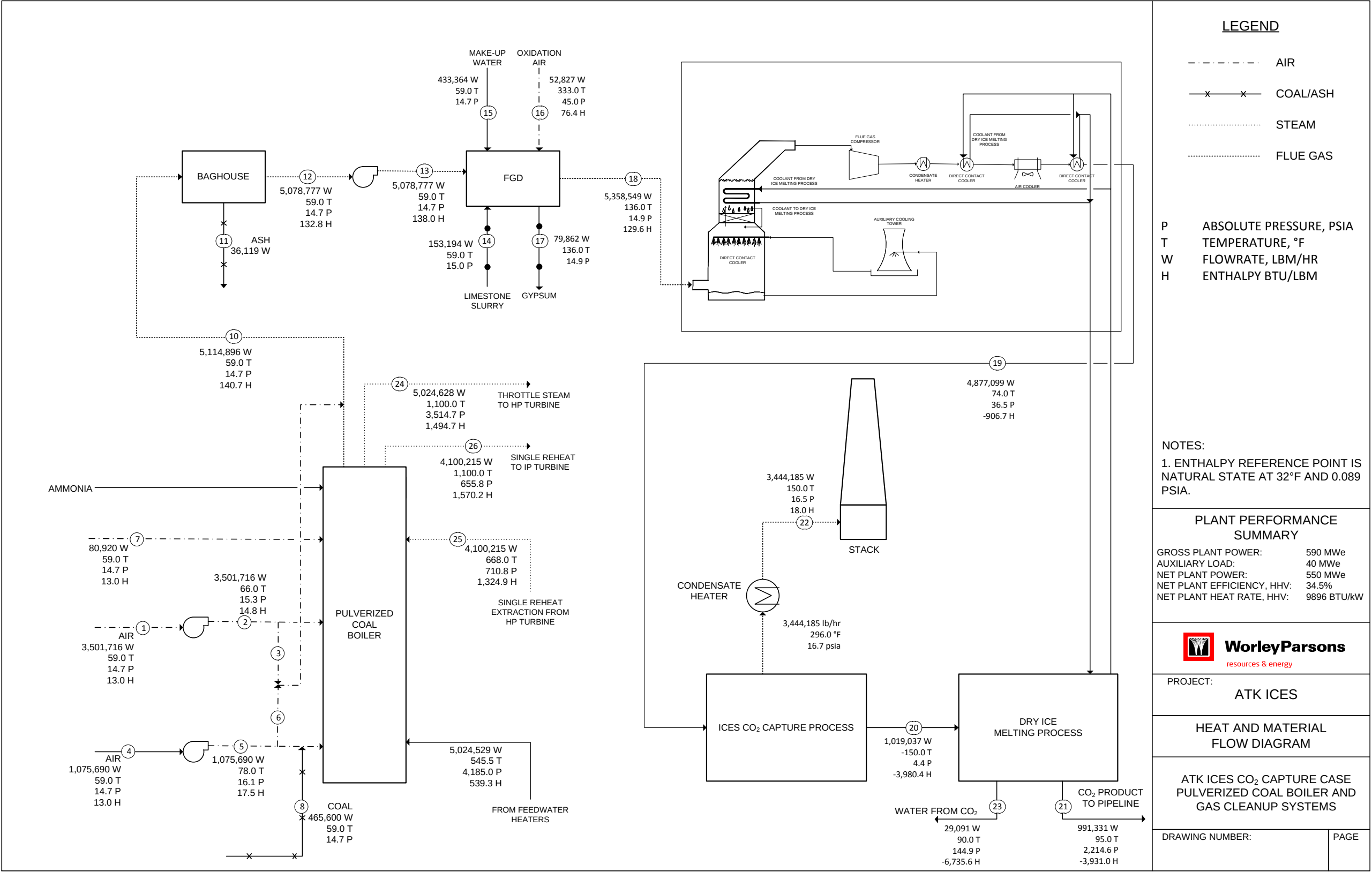
Exhibit 4-5 ATK ICES Case Heat and Mass Balance, Supercritical PC Boiler with CO 2 Capture
