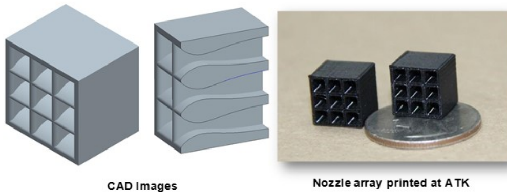
Figure 2 CAD model and photo of nine-cell grating nozzle concept
