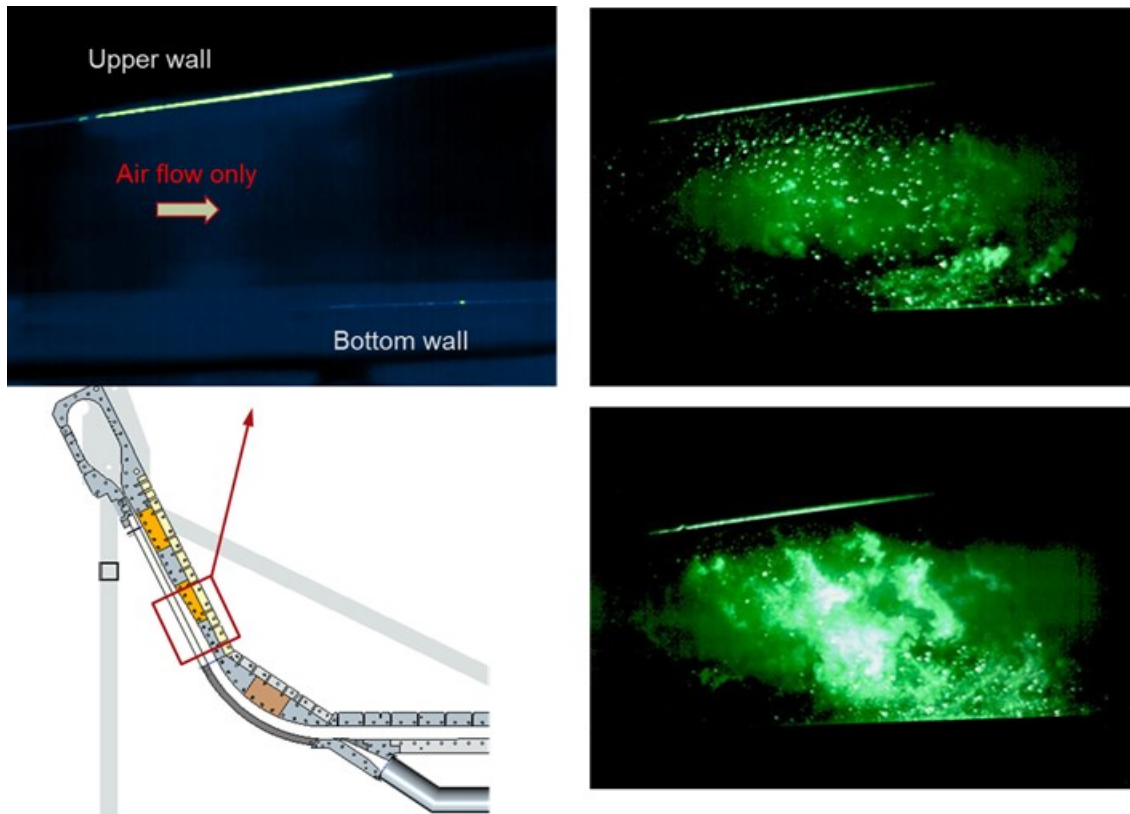
Figure 40: Laser images of the flow upstream of the turning duct (before CO 2 migration).
