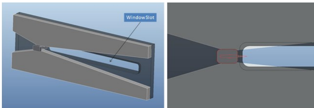
Figure 3 CAD model of single centerbody nozzle for OSU
