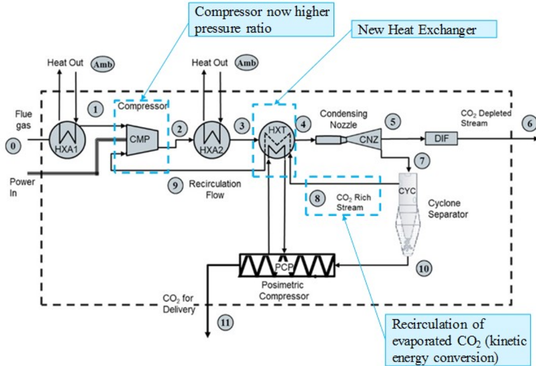
Figure 62 Final ICES System Schematic
