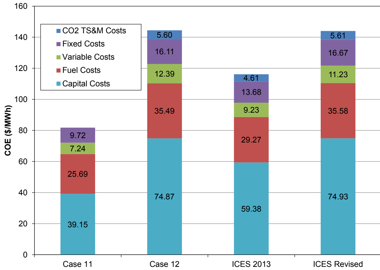
Figure 3-1 Comparison and Breakdown of COE for the DOE/NETL Baseline Cases and the ICES Cases
