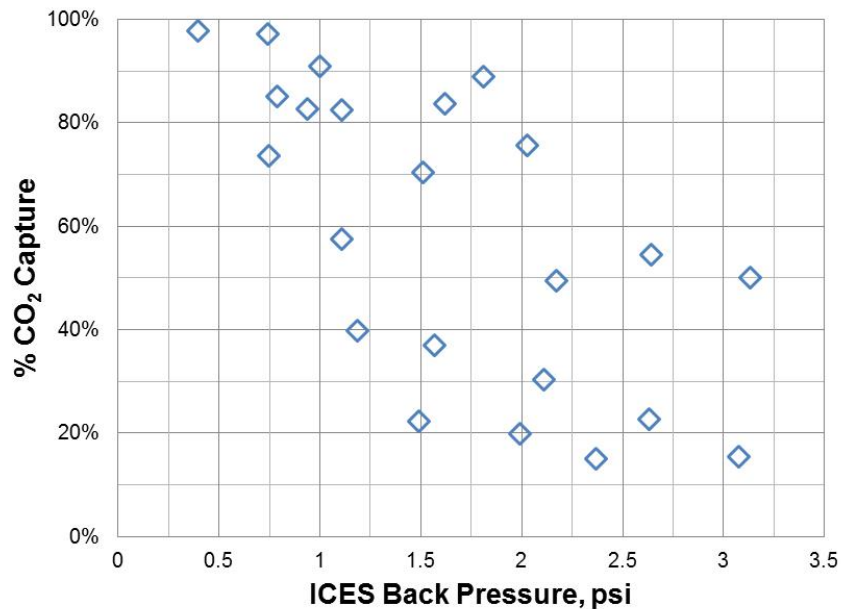
Figure 43 Bench Scale Test Results – percent CO 2 captured as a function of the back pressure.
