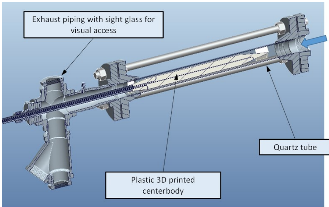
Figure 69: Subsonic ICES Test Article Assembly Key Components
