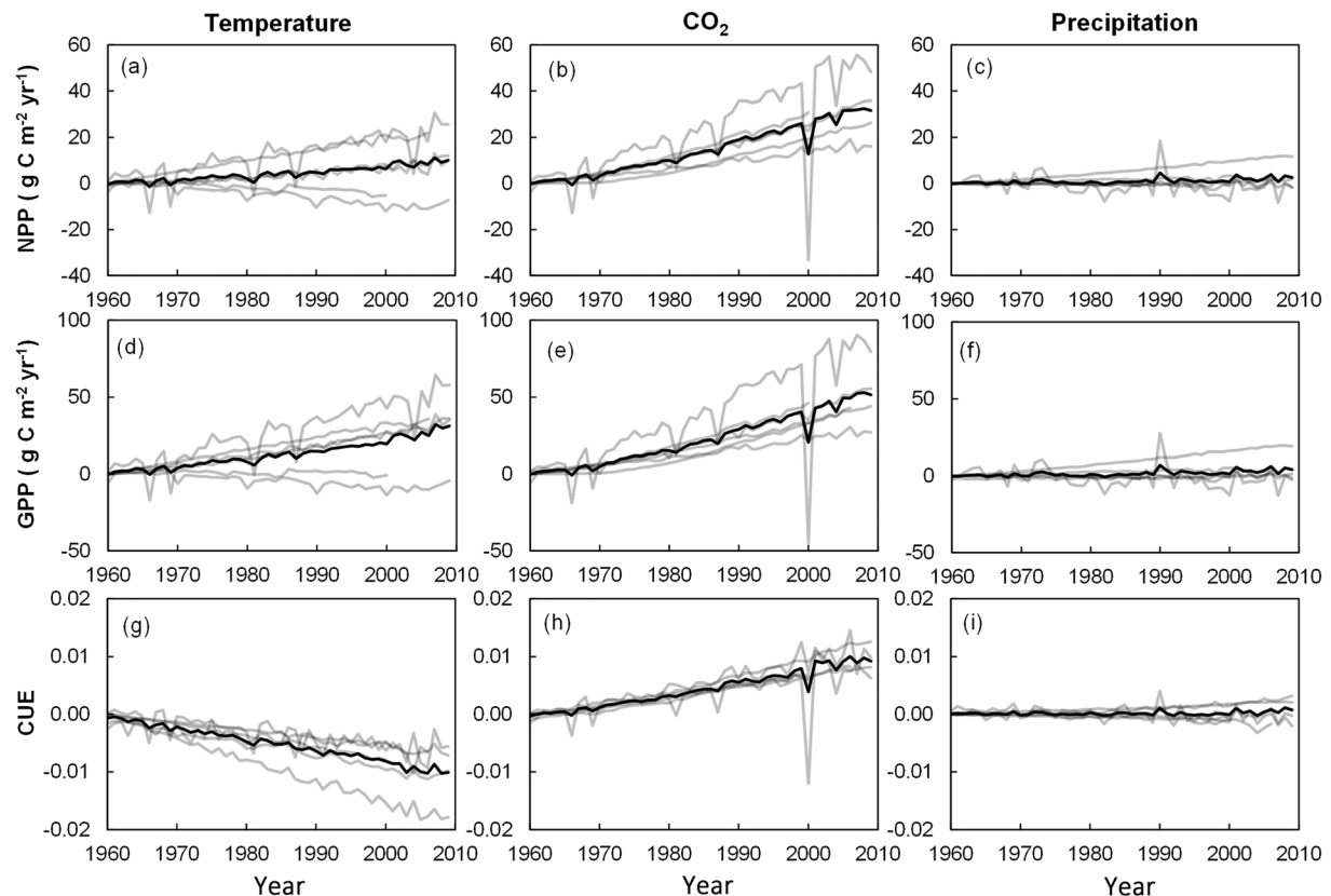
Figure 7. The impacts of air temperature, atmospheric \text{CO}_2 , and precipitation on (a–c) NPP, (d–f) GPP, and (g–i) CUE over 1960–2009. The gray lines are individual model results (note that only 6 out of the 10 models have done the R02–R04 simulations; Table 1) and the bold black line is the ensemble model mean.
