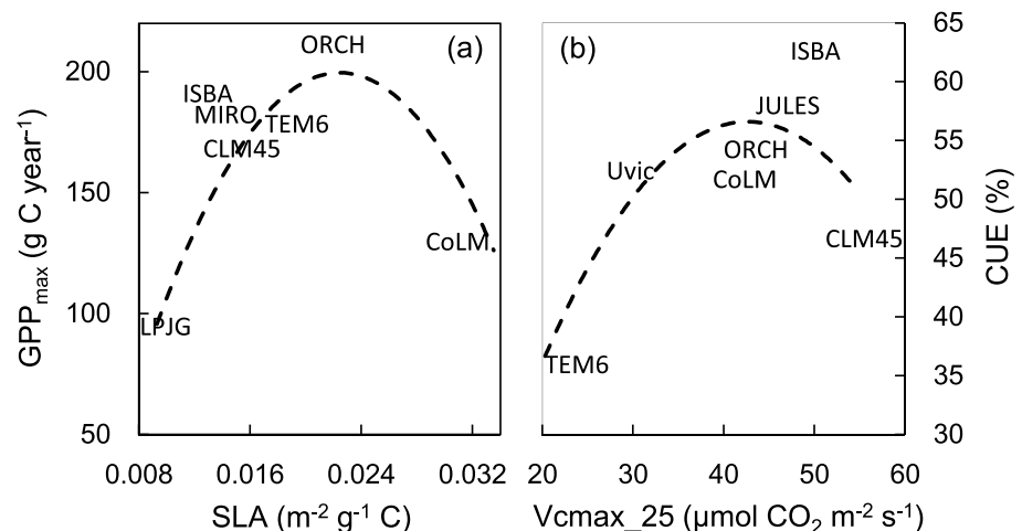
Figure 4. Dependences of (a) \text{GPP}_{\text{max}} on SLA and (b) CUE on V_{\text{cmax\_25}} among models. Note that the medians of SLA and V_{\text{cmax\_25}} across the permafrost region in each model were used in the regression analyses ( \text{GPP}_{\text{max}} = -568678\text{SLA}^2 + 25760\text{SLA} - 92 ; \text{CUE} = -0.04V_{\text{cmax\_25}}^2 + 3.39V_{\text{cmax\_25}} - 15.80 ).
