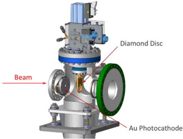
Figure 9: Cross section of IM2 for windowless front end.
