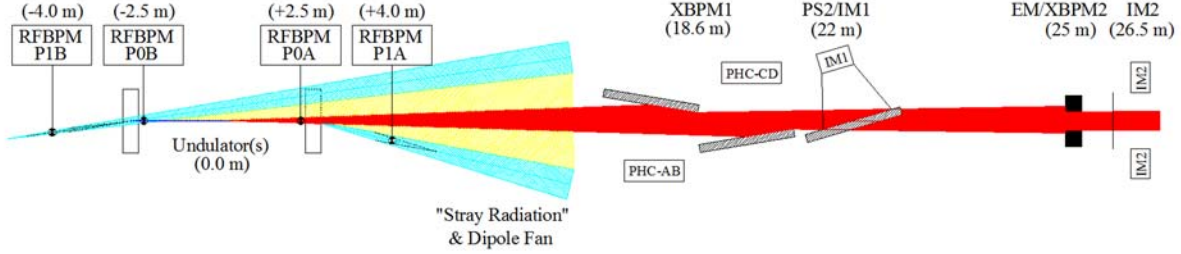
Figure 1: APS 27-ID RFBPM and XBPM system components for orbit controls.
