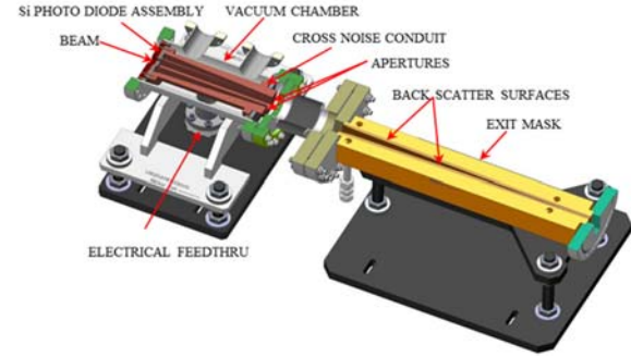
Figure 3: The second XBPM uses the XRF from the Exit Mask to monitor positions of the x-ray beam before it enters the beamline.
