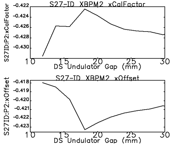
Figure 5: XBPM2 horizontal calibration constant (upper panel) and offset (lower panel) as functions of undulator gap.
