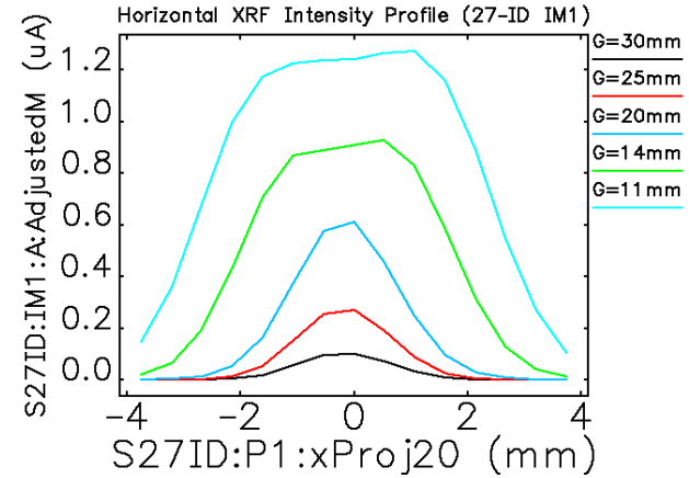
Figure 8: IM1 signal as functions of horizontal beam positions for selected undulator gaps.
