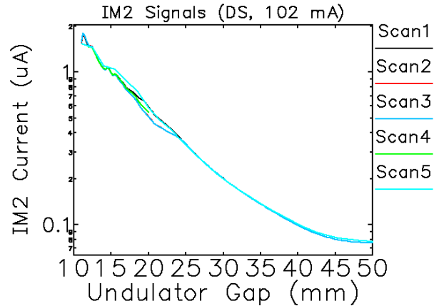
Figure 12: IM2 current as functions of undulator gap for five different small deviations in orbit angles.
