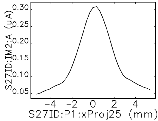
Figure 11: The normalized IM2 currents as functions of horizontal beam position for undulator gap of 25 mm.
