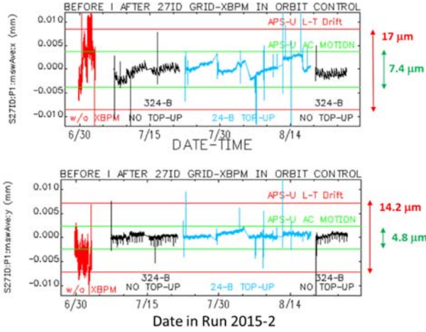
Figure 2: S27-ID GRID-XBPM data taken in 60-days of user operations: The upper panel is for the horizontal x-ray beam positions at 18.6 m from the undulator source and the lower panel is for the vertical beam positions.
