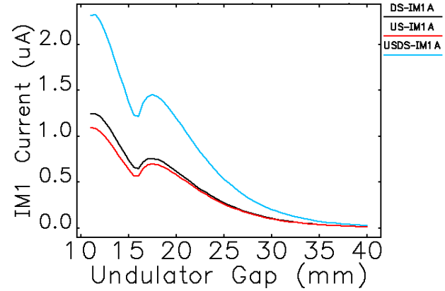
Figure 7: IM1 signal current as functions of the undulator gap for upstream (US), downstream (DS) and both undulators (USDS), respectively.
