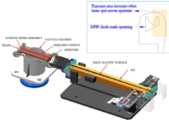
Figure 6: The first intensity monitor uses the XRF photons from the photon shutter (PS2) to monitors the beam intensity at the shutter.
