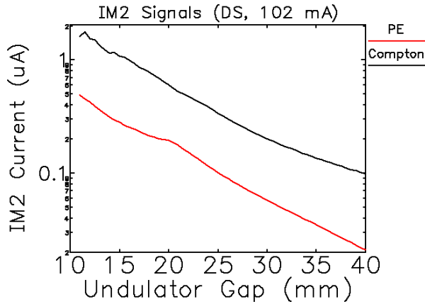
Figure 10: Absolute value of the IM2 current as functions of undulator gap for Compton and photoemission mode, respectively.
