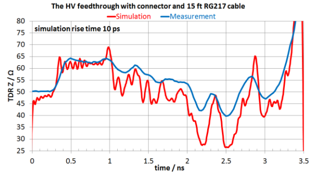
Figure 6: TDR comparison between the measurement and simulation of the HV feedthrough with the connector and RG217 cable.
