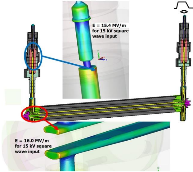
Figure 9: Simulated high electric fields and their locations in the prototype kicker assembly.
