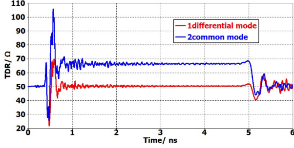
Figure 4: The differential and common-mode TDR simulation in prototype kicker.
