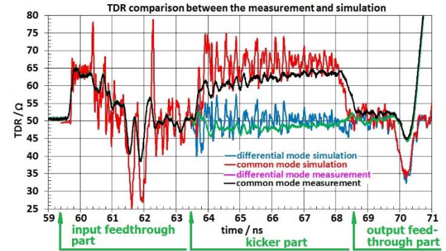
Figure 7: TDR comparison between the measurement and simulation of the MBA prototype kicker assembly.
