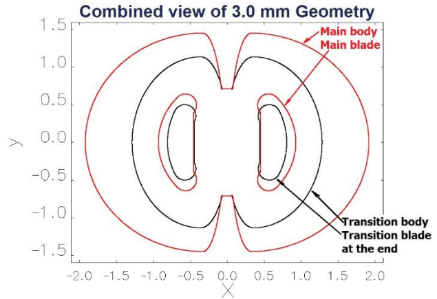
Figure 2: 2D modelling result geometry.
