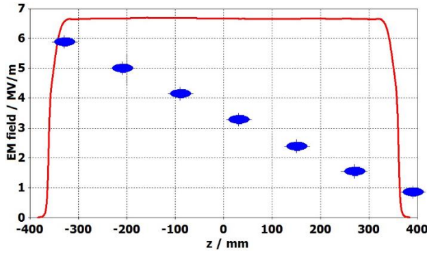
Figure 8: Calculated electromagnetic fields along the beam path and the bunch trace. Red: EM field amplitude. Blue: Gaussian bunch trace.
