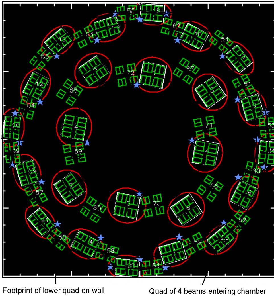
Figure 1: Projection of the top half of the NIF target chamber showing the top beam quads entering through the FOA apertures in the first wall and the 1w unconverted light footprint from the bottom quads incident on the first wall.
