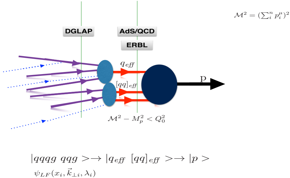
Figure 9: A. A model for evolution starting with a nonperturbative hadronic LFWF. B. Hadronization and evolution ending with a hadronic LFWF. The intermediate quark and gluon states are off the P^- energy shell and thus off-the-invariant mass shell \mathcal{M}^2 > m_H^2 . In the off-shell domain \mathcal{M}^2 - M_H^2 > \kappa^2 , the intermediate quarks and gluons obey the DGLAP and ERBL QCD evolution. If a cluster of quarks and antiquarks satisfies \mathcal{M}^2 - M_H^2 < \kappa^2 , the intermediate state sees the color confinement interaction. The meson LFWF connects the intermediate q\bar{q} state, which is off of the P^- energy shell and thus off-the-invariant mass shell \mathcal{M}^2 > m_H^2 to the physical meson state with \mathcal{M}^2 = m_H^2 . The LF angular momentum J^z is conserved at every vertex [43]
