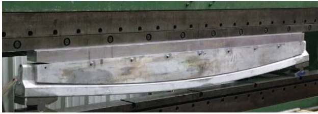
Figure 2: Bending of an L-bend chamber extrusion.
