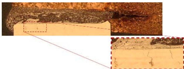
Figure 5: Stress fracturing in electron beam welds.
