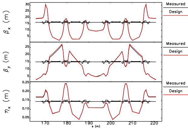
Figure 2: Comparison between the designed and measured optics functions in sectors 7 and 8.
