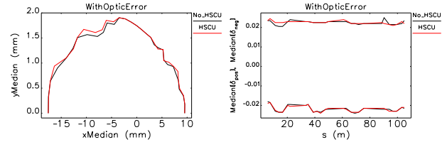
Figure 6: Comparison of dynamic aperture with (red) and without (black) HSCU (left) and local momentum aperture (right).
