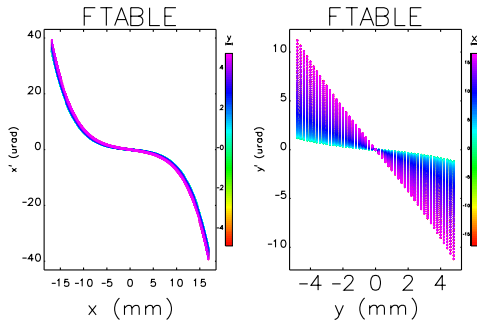
Figure 4: Calculated detailed kick map for HSCU. Color code is the other coordinate (for example, y for the left plot)
