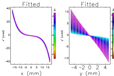
Figure 5: Kick map from fitted multipole components. [8] S. Kim. NIMA , 584:266 (2008).
