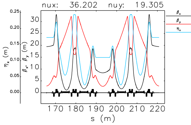
Figure 1: Twiss parameters of the modified sector 7 and 8. ID straight section is in the middle of the plot.
