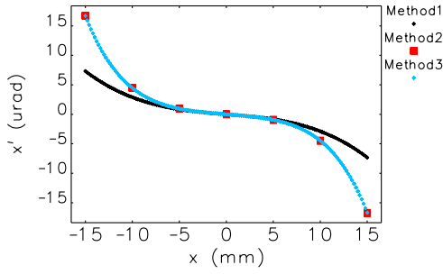
Figure 3: Calculated kick map for HSCU using field from (2). Method 1 is P. Elleaume integration, methods 2 and 3 are direct numerical integration and FTABLE.
