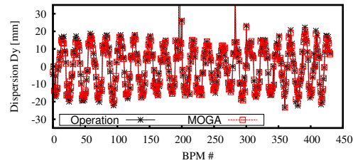
Figure 9: Comparison of measured vertical dispersion.
