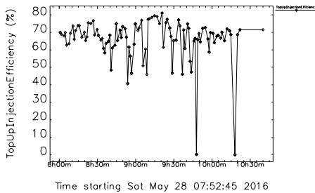
Figure 7: Top up injection efficiency during optimization.
