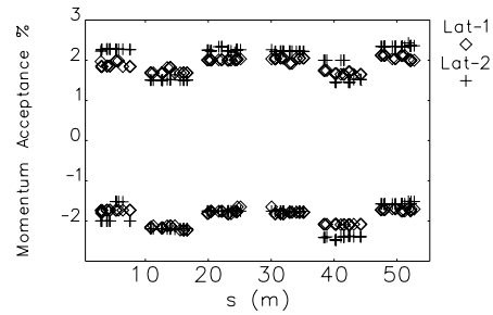
Figure 8: Comparison of simulated local momentum acceptance between the operation lattice (Lat-1) and one of the online optimized lattice (Lat-2).
