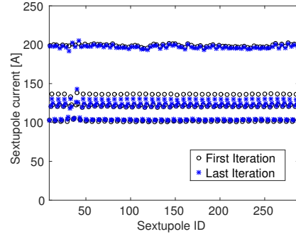
Figure 6: Topup mode, sextupole magnets strength for the first and last iteration, a total of 280 sextupoles in 40 sectors (21 families in total). Starting point is optimized sextupoles from MOGA simulation [7] on the medium chromaticity lattice ( \xi = 6 ).
