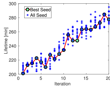
Figure 2: Lifetime (calculated using DCCT current measurements) at each iteration. A total of 20 iterations (finished in 25 minutes), and 10 seeds for each iteration. Starting point is optimized sextupoles from MOGA simulation [7] [15] on the high chromaticity lattice ( \xi = 11 ).
