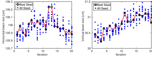
Figure 3: Horizontal and vertical beam size (at sector 35 pinhole location) for each iteration. A total of 20 iterations, and 10 seeds for each iteration. Starting point is optimized sextupoles from MOGA simulation [7, 15] on the high chromaticity lattice ( \xi = 11 ).
