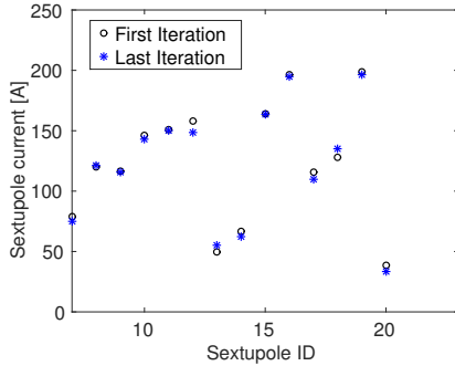
Figure 4: Sector 4 and 5 sextupole magnets strength for the first and last iteration (a total of 14 sextupoles). Starting point is optimized sextupoles from MOGA simulation [7, 15] on the high chromaticity lattice ( \xi = 11 ).
