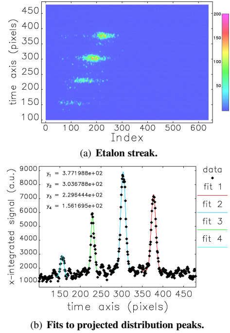
Figure 2: (a) An example of a streak image with multiple peaks from the etalon test and (b) Gaussian fits on Range 1 using a 36.4-ps spacing between peaks (527 nm).
