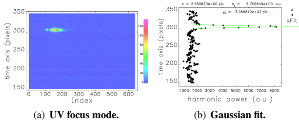
Figure 3: UV focus mode image and Gaussian profile fit.
