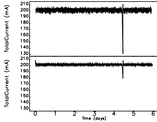
Figure 4: Total current vs time for the first week of simulated operation for 48-bunch (top) and 324-bunch (bottom) modes with round beams and existing rf systems.
