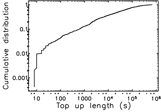
Figure 3: Cumulative distribution of continuous top-up duration for APS all runs from 2004 to present.
