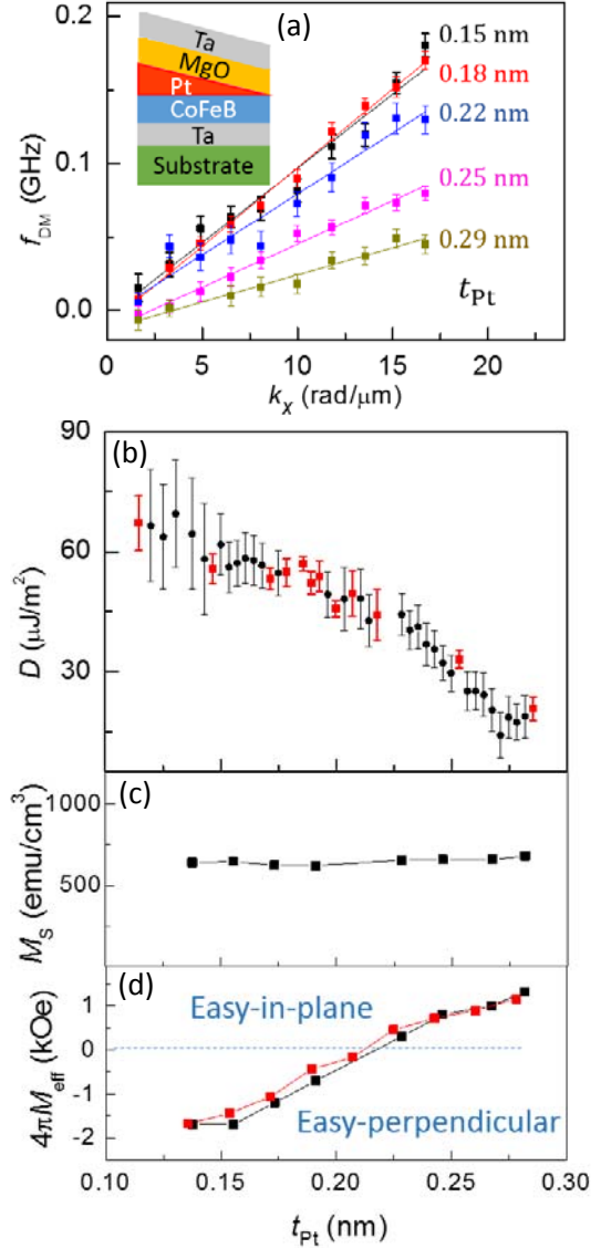
Fig. 3. (a) The linear dependences of f_{DM} on k_x for a Pt wedge layer with a thickness gradient, where the inset illustrates the multilayer structure. The solid lines show the least square fits. (b) The interfacial DMI constant D as a function of the Pt layer thickness t_{Pt} . The red squares are derived from the linear fits on the k_x dependences of f_{DM} with different t_{Pt} using Equation 2. The black circles are obtained through f_{DM}/k_x at fixed k_x = 16.7 \text{ rad}/\mu\text{m} by varying t_{Pt} in a smaller step size. (c) M_s and (d) 4\pi M_{eff} as functions of t_{Pt} . The red (black) dots in (d) are obtained from the field dependence BLS (VSM) measurements, respectively.
