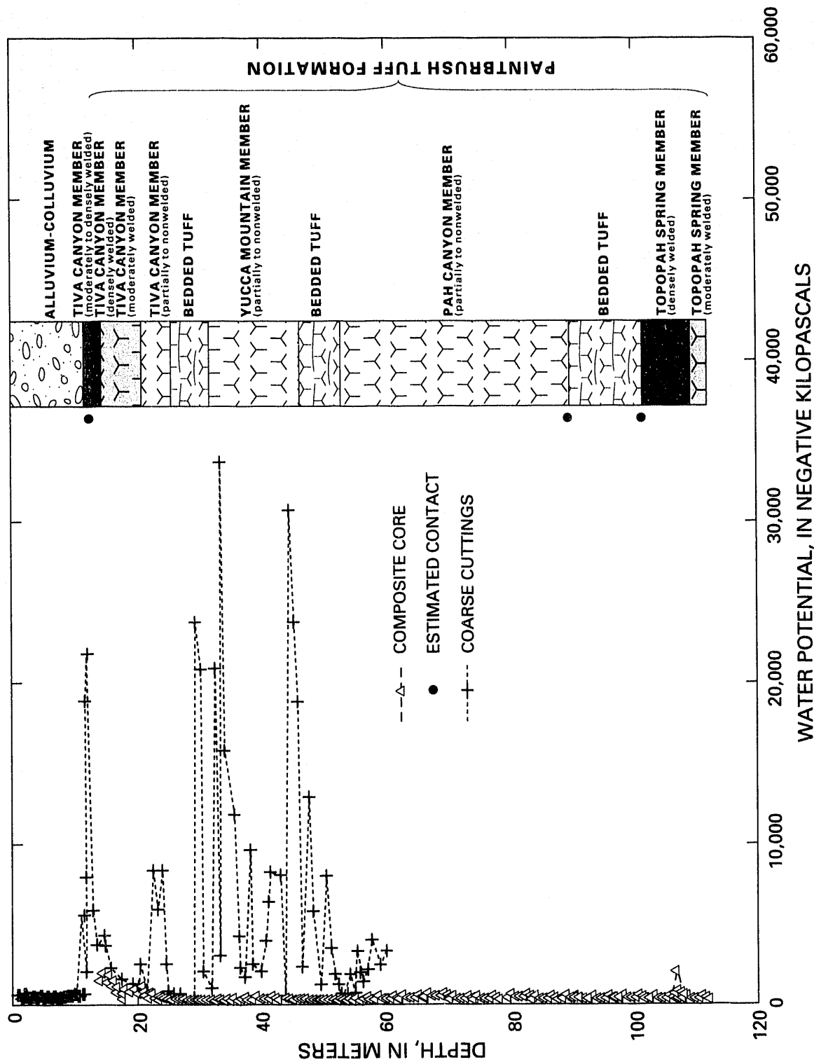
Figure 5.--Water-potential measurements of core and cuttings from test hole UE-25 UZ #4.
