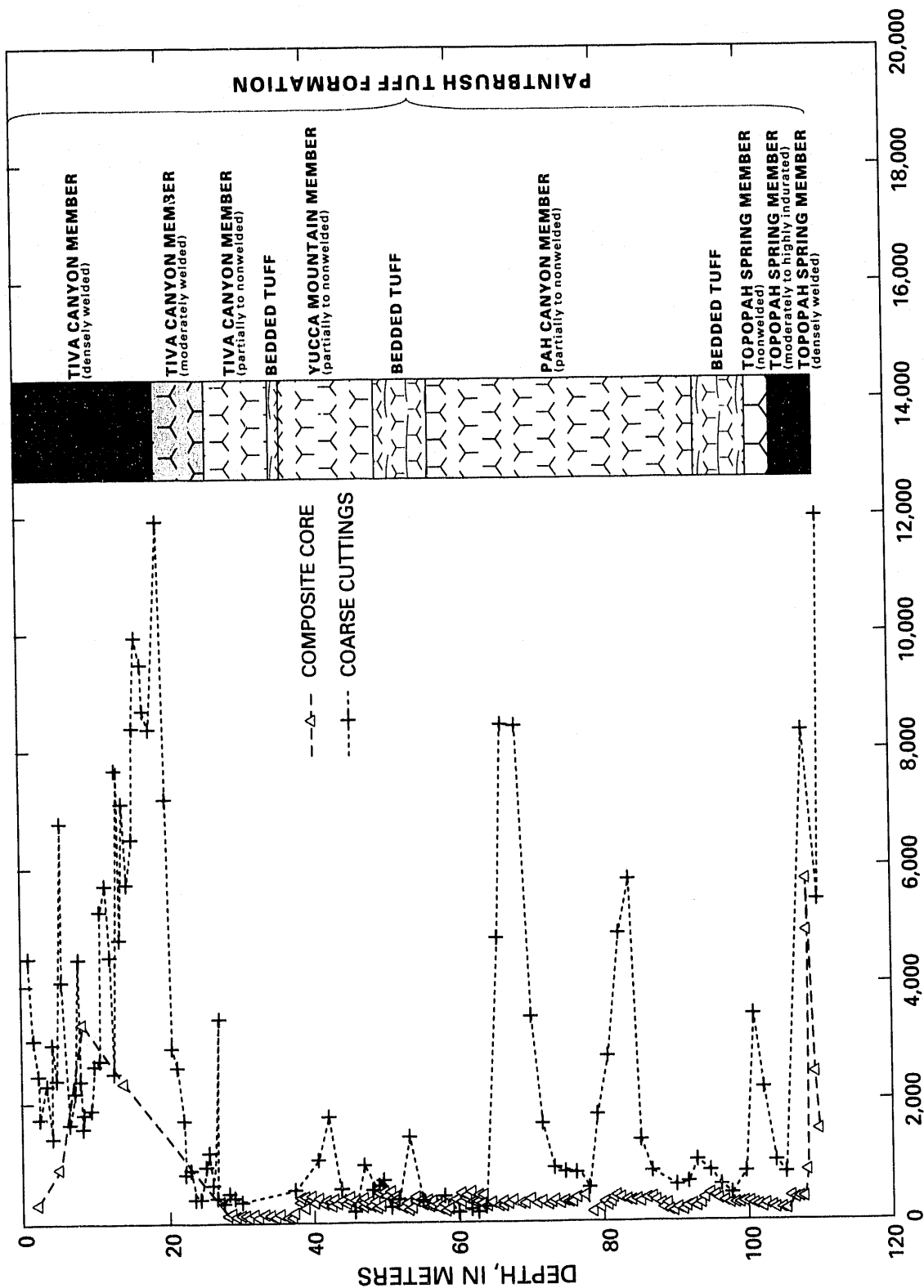
Figure 6.--Water-potential measurements of core and cuttings from test hole UE-25 UZ #5.
