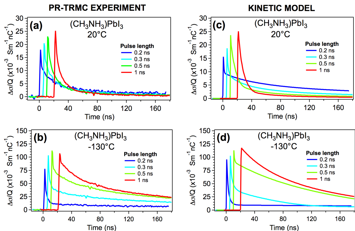
Figure 3. Experimental (a,b) and kinetic model fit (c,d) Pulse length dependence of \text{CH}_3\text{NH}_3\text{PbI}_3 at room (top) and lower (bottom) temperatures
