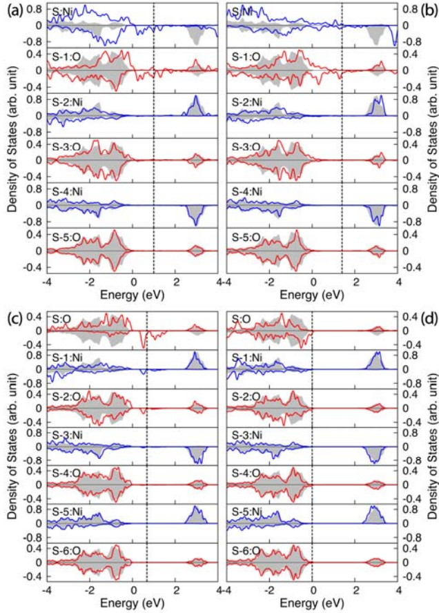
FIG. 3. Layer-resolved PDOS comparison between bulk NiO and (a) 1\times 1 _Ni, (b) 1\times 1 _Ni-H, (c) 1\times 1 _O, (d) 1\times 1 _O-H surface structures. VBM of bulk NiO is set to 0, Fermi levels of different reconstructed surfaces are shown in dashed line. The Ni-3d and O-2p PDOS are represented by blue and red lines, and the bulk NiO PDOS is shown in solid grey.
