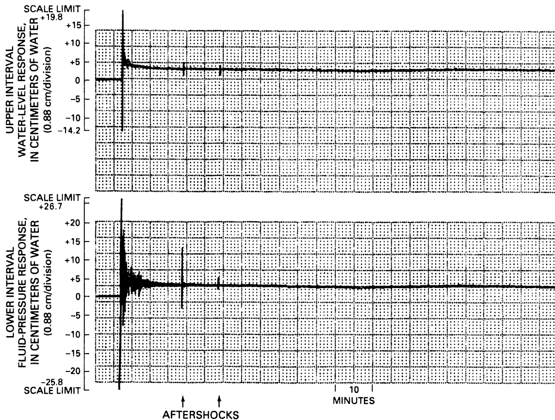
Figure 4. Well USW H-5 response to earthquake at Little Skull Mountain, Nevada, occurring at 10:14:22 UTC, on June 29, 1992.
