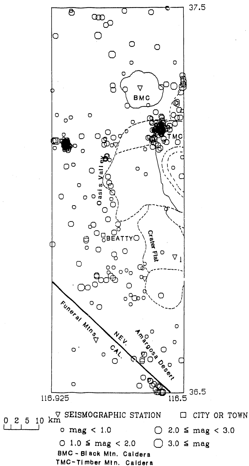
Figure 7.- Earthquake epicenters in the Oasis Valley region west of the Black Mountain and Timber Mountain calderas and east of Sarcobatus Flat, for the period 1979 through 1989. Caldera boundaries are shown as solid curves or dashed curves (written communication, Will Carr, 1990). An inner limit and an outer limit for the resurgent dome of Timber Mountain are partially shown as dashed rings.
