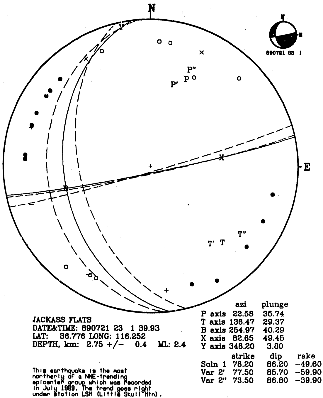
Figure D36. Oblique normal-slip or strike-slip focal mechanism solutions for an earthquake at Little Skull Mountain, Nevada Test Site, on July 21, 1989, 23:01:40 UTC.
