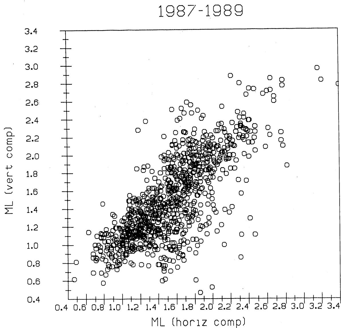
Figure 3.— Comparison of horizontal-component instrument-determined local magnitudes, M_L^H , with vertical-component instrument-determined local magnitudes, M_L^V , for a subset of the 1987 through 1989 SGBSN hypocenter data.
