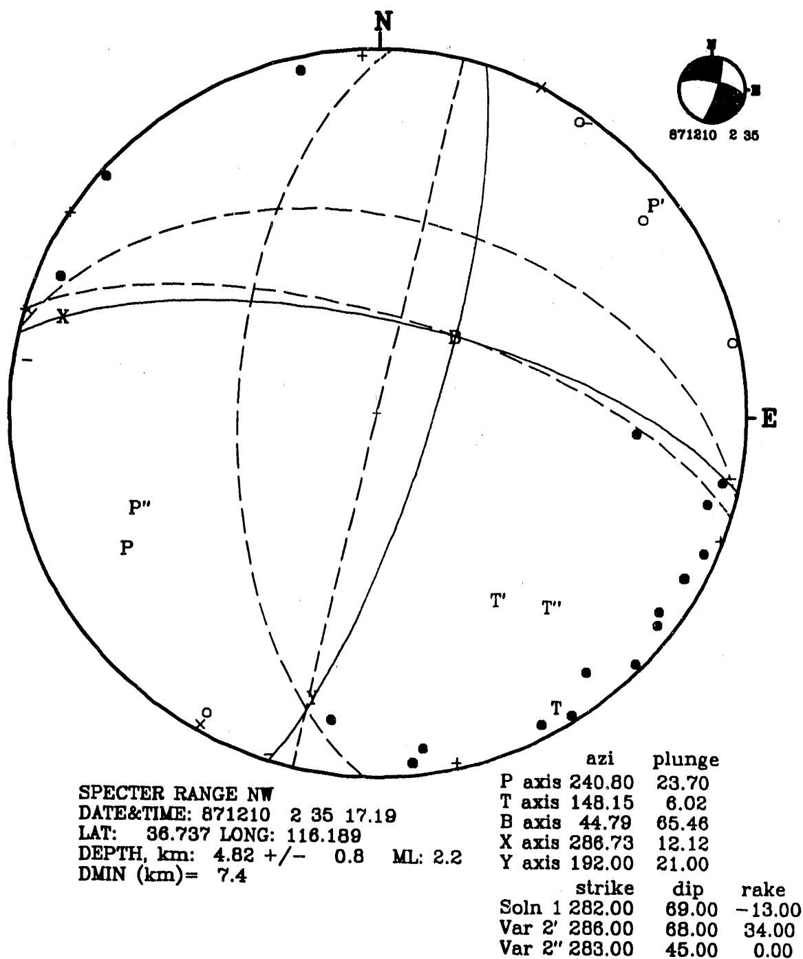
Figure D15. A set of predominantly strike-slip focal mechanism solutions for an earthquake of December 10, 1987, 2:35:17 UTC, in the Specter Range, southern Nevada Test Site.
