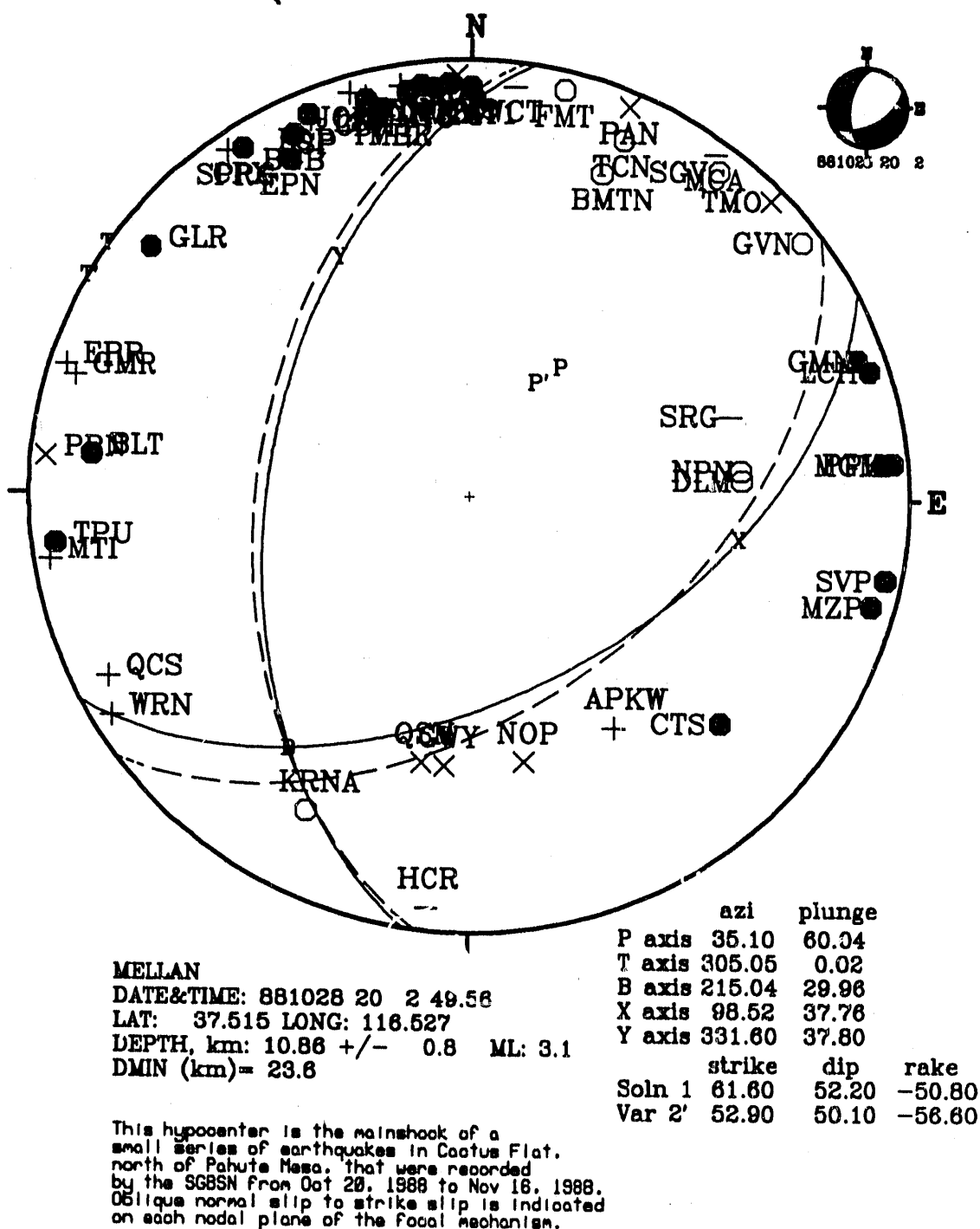
Figure D26. Oblique normal-slip focal mechanism solutions for a M_L = 3.1 earthquake at Cactus Flat, Nevada (Mellan quadrangle) on October 28, 1988, 20:02:50 UTC. That earthquake was the mainshock of a series that lasted nearly one month.
