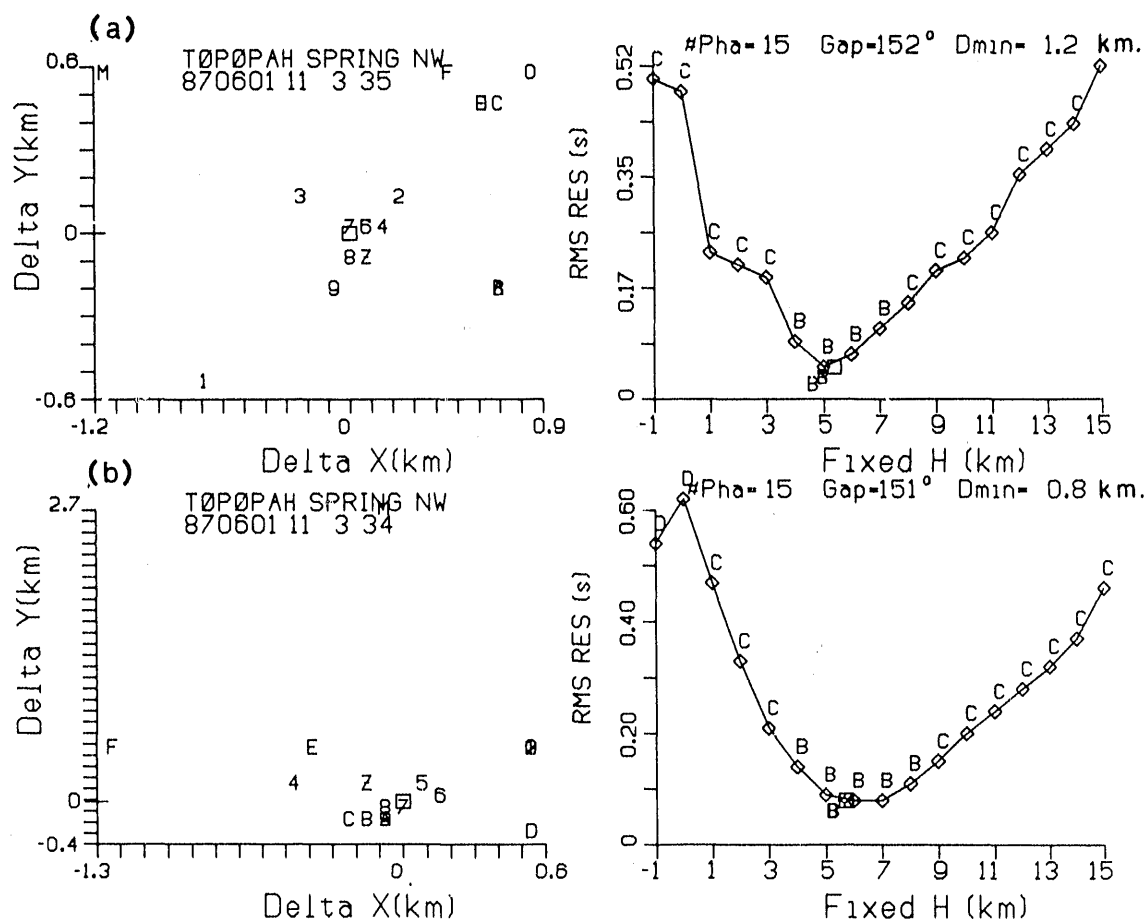
Figure 10.—(a) Left side , the distribution of epicenters for various fixed-depth hypocenter solutions for the Yucca Mountain earthquake of June 1, 1987, 11:03:35 UTC, where all hypocenters are determined using the standard SGB velocity model (Appendix F, Figure F1(a)). The epicenter symbols are M, 0, 1, 2, ..., A, B, C, D, E, F, corresponding to depth-constrained hypocenters having z = -1, 0, 1, 2, \dots, 10, 11, 12, 13, 14, 15 km, respectively. The open square symbol at (0,0) is for a free-depth solution, with starting iterate depth 7 km, and the symbol "Z" is for a free-depth solution with starting iterate depth 0 km (at sea level). Right side , the variation in RMS travel time residual for various fixed-depth and free-depth hypocenters for that earthquake and velocity model. (b) The same distribution of epicenters ( left side ) and variation in RMS travel time residual ( right side ) as in Figure 10(a), except that here, the Yucca Mountain velocity model (Appendix F, Figure F1(b)) is used in hypocenter determinations.
