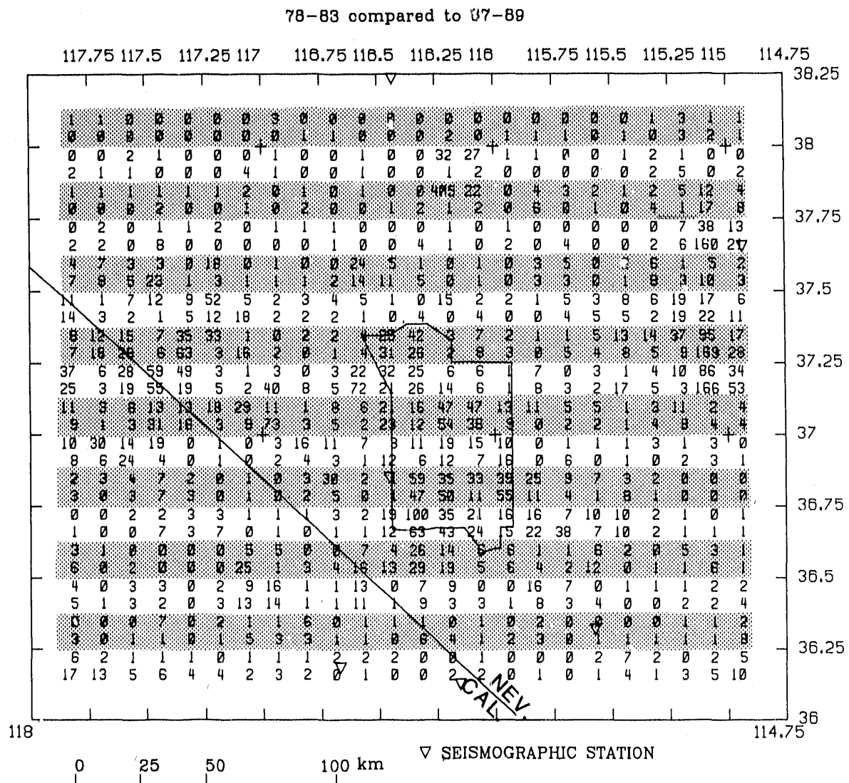
Figure 9.- Map of SGB region showing, on a 7\frac{1}{2}' quadrangle scale, the number of earthquakes recorded by the SGBSN in 1987 through 1989 (top number in each 7\frac{1}{2}' quadrangle) compared to number of earthquakes recorded by the SGBSN in the period, August, 1978 through December, 1983 (bottom number in each quadrangle). Alternate rows are shaded to aid in visual separation of information in adjacent quadrangles.
