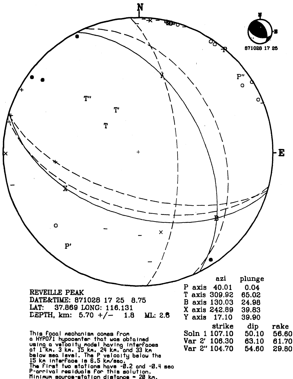
Figure D14. An oblique reverse-slip focal mechanism solution for the same earthquake as in Figure D13, in which the depth of focus is assumed to be 5.7 km below sea level. A velocity discontinuity at 15 km below sea level (shifted from the 12 km discontinuity in the model used in Figure D13) was used for ray tracing when computing this preliminary hypocenter.
