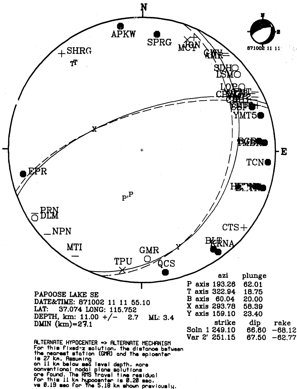
Figure D12. An alternate predominantly normal-slip focal mechanism solution for the same earthquake as in Figure D11, in which the previously shallow-dipping nodal plane now dips at about 30 degrees, when the depth of focus is assumed to be 11 km below sea level.
