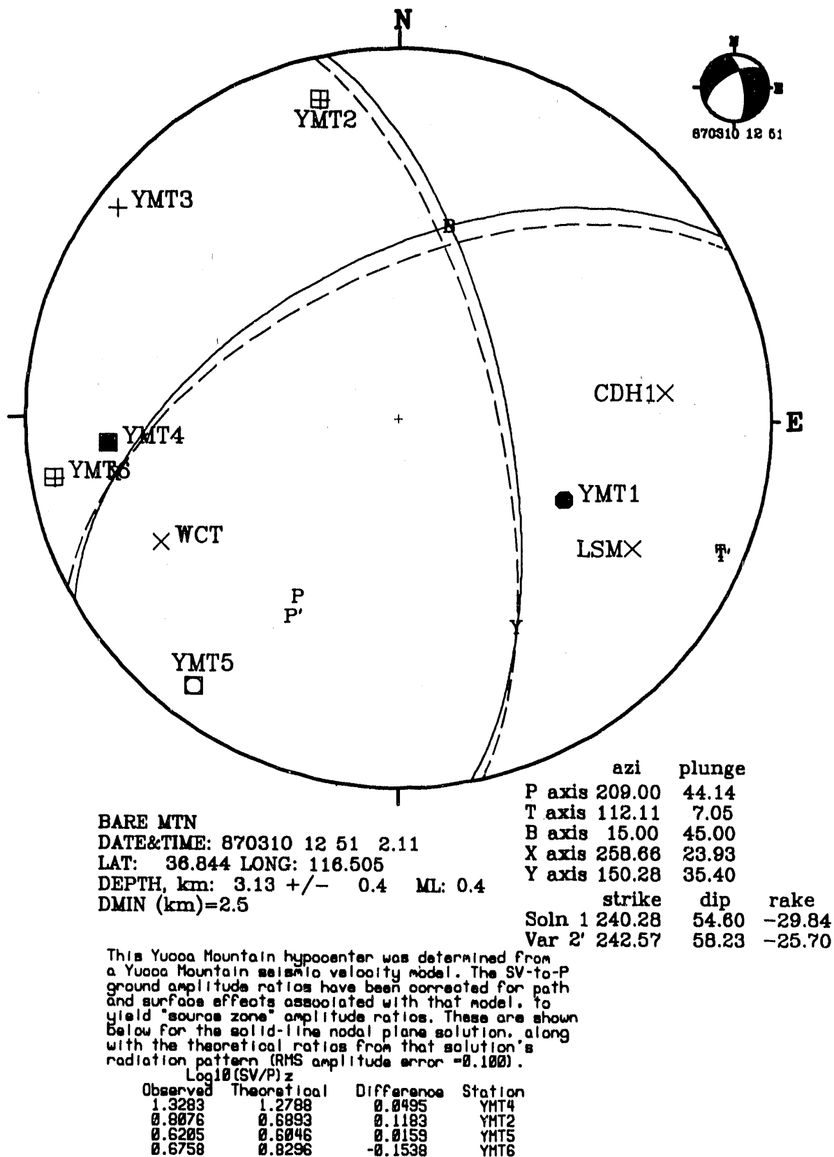
Figure D3. Predominantly strike-slip focal mechanism for a very small earthquake of March 10, 1987, at Yucca Mountain, Nevada, constrained by several SV/P z amplitude ratios.
