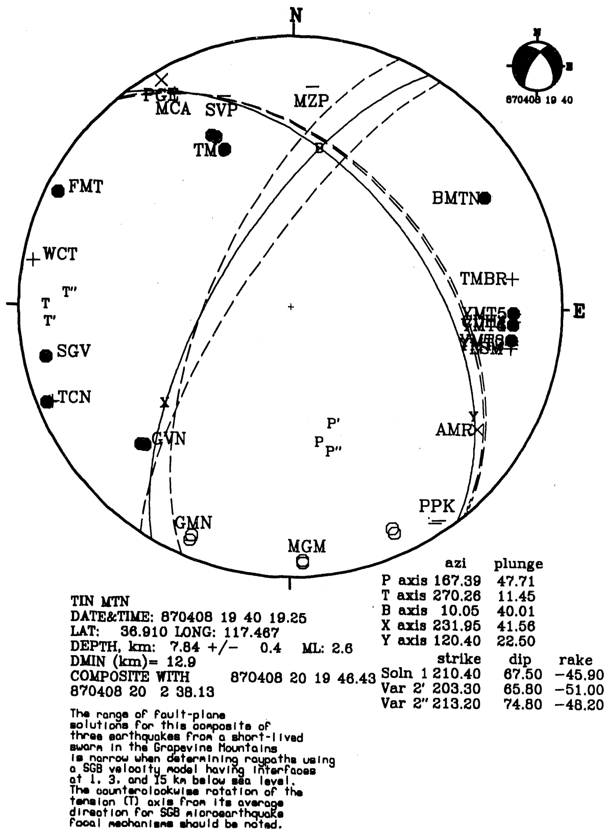
Figure D4. A composite, oblique, normal-slip set of focal mechanism solutions for earthquakes of April 8, 1987, in the Grapevine Mountains, California.
