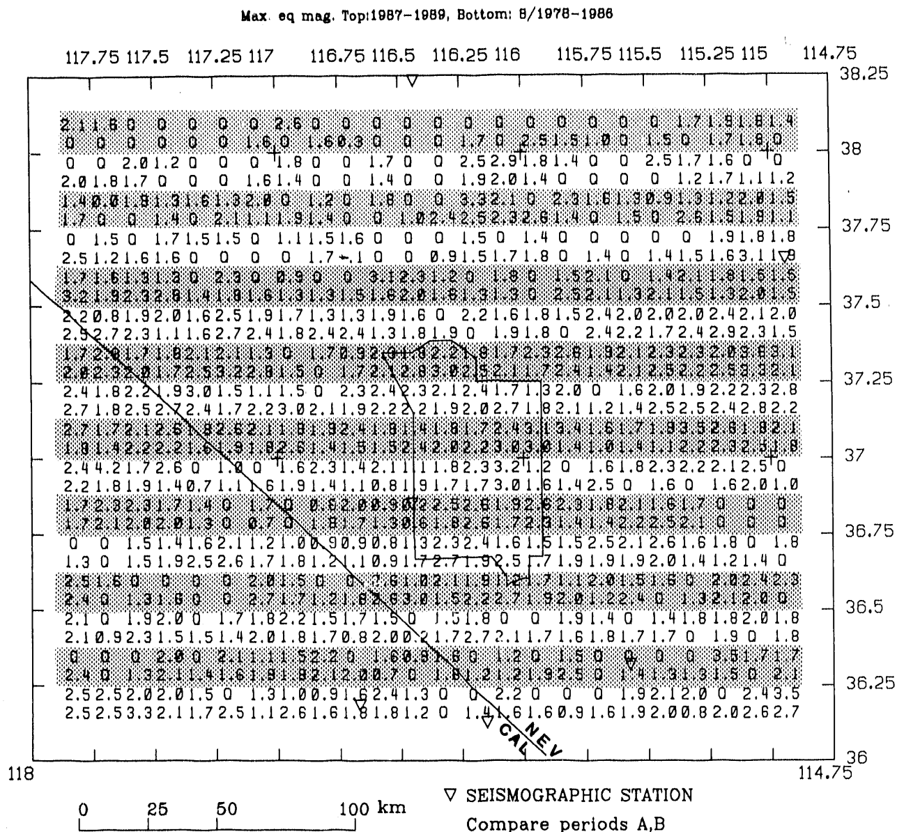
Figure A5.- Map tabulating maximum earthquake magnitude ( M_L where available, otherwise M_D or M_{ca} ) in each 7\frac{1}{2}^\circ quadrangle within the ranges 114.875^\circ\text{W} to 117.875^\circ\text{W} and 36.125^\circ\text{N} to 38.125^\circ\text{N} recorded by the SGBSN. The top number is the maximum magnitude in the period 1987 through 1989, and the bottom number is the maximum magnitude in the period August, 1978 through December 1986. The letter "Q" (quiet) within a quadrangle means no earthquakes were monitored during that period by the SGBSN. The NTS boundary and part of the California-Nevada state border are shown. Alternate rows are shaded to aid in visual separation of information in adjacent quadrangles.
