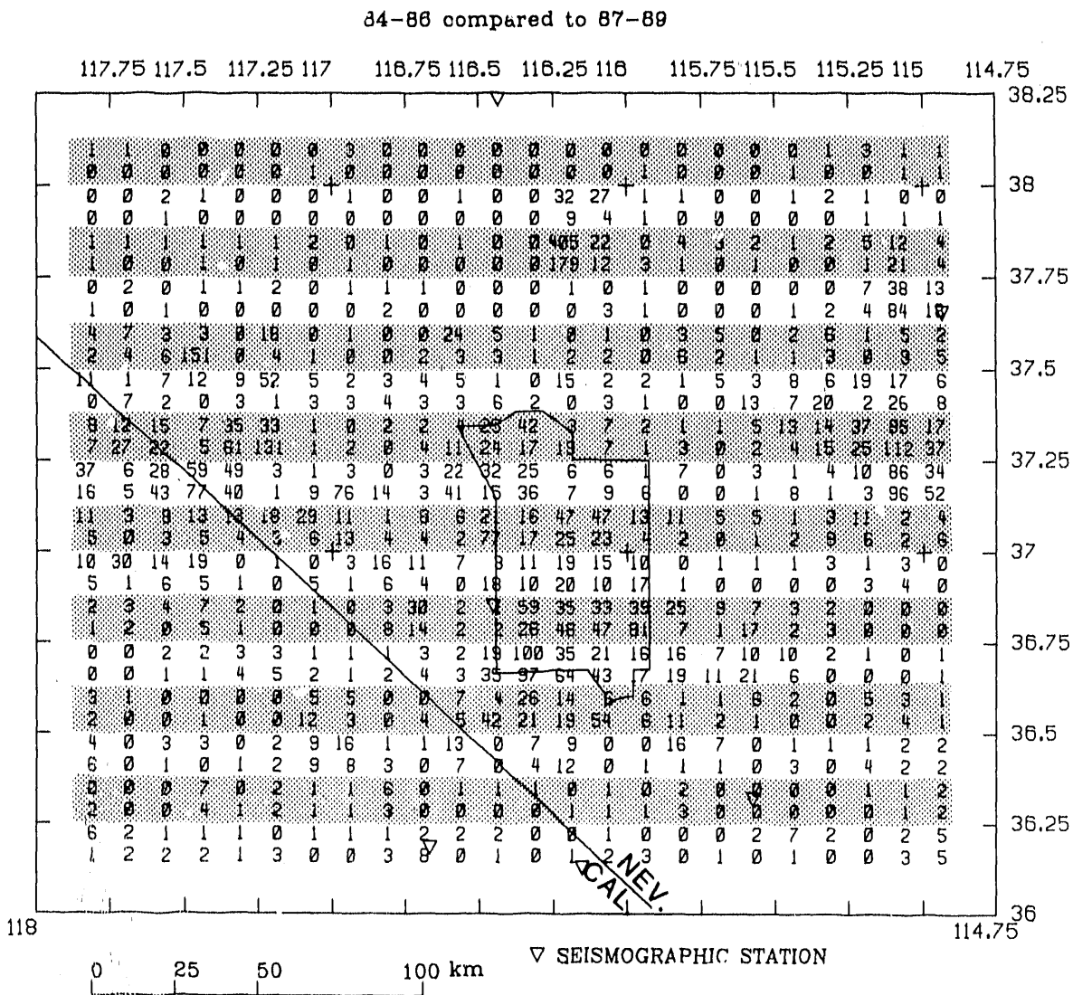
Figure 8.-- Map of SGB region showing, on a 7\frac{1}{2}' quadrangle scale, the number of earthquakes recorded by the SGBSN in the three-year period, 1987 through 1989 ( top number in each 7\frac{1}{2}' quadrangle) compared to number of earthquakes recorded by the SGBSN in the previous three-year period, 1984 through 1986 ( bottom number in each quadrangle). Alternate rows are shaded to aid in visual separation of information in adjacent quadrangles.
