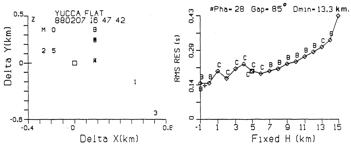
Figure 14.— Left side: epicentral scatter for various fixed depth and free depth HYPO71 hypocenters for a Yucca Flat earthquake of February 7, 1988, 16:47 UTC. The symbols correspond to the fixed depth hypocenters: M,0,1,2, ..., A,B,C,D,E, and F for depths = -1,0,1,2, ...,10,11,12,13,14, and 15 km below sea level. The open square is for the free depth solution, with starting iterate depth 7 km, and the Z is for the free depth solution with starting iterate depth 0 km (at sea level). Right side: The RMS travel time residual for the various fixed depth and free depth solutions for the same event. The letters above the fixed depth solutions, and below the free depth solutions, are HYPO71 "grades" assigned during the process of hypocenter determination. This plot shows a small variation in RMS for many shallow depth estimates, a pattern that is often present for SGB data sets where the nearest station is relatively distant from the epicenter.
