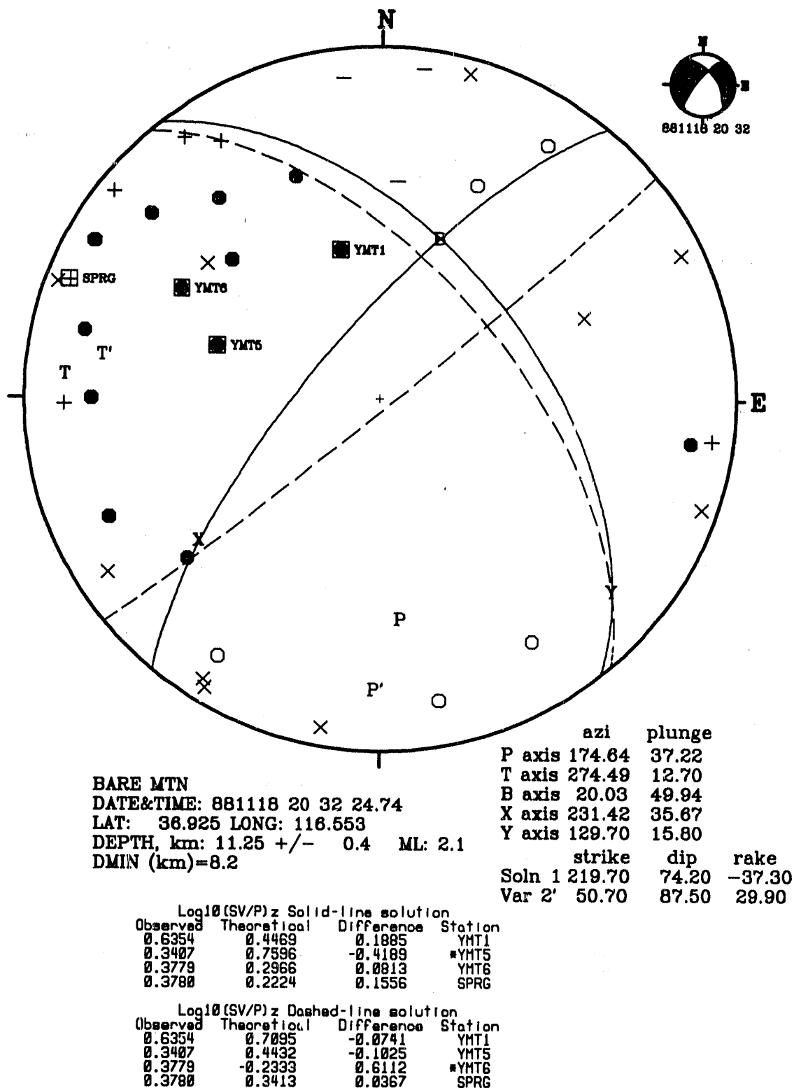
Figure D28. Predominantly strike-slip focal mechanism solutions for the M_L = 2.1 mainshock of a short-lived series of microearthquakes at a northwest boundary of Yucca Mountain, Nevada (Bare Mountain quadrangle) on November 18, 1988, 20:32:25 UTC. To provide additional constraint on the focal mechanisms, SV/P_s amplitude ratios were included from a foreshock (the mainshock clipped nearby station seismograms).
