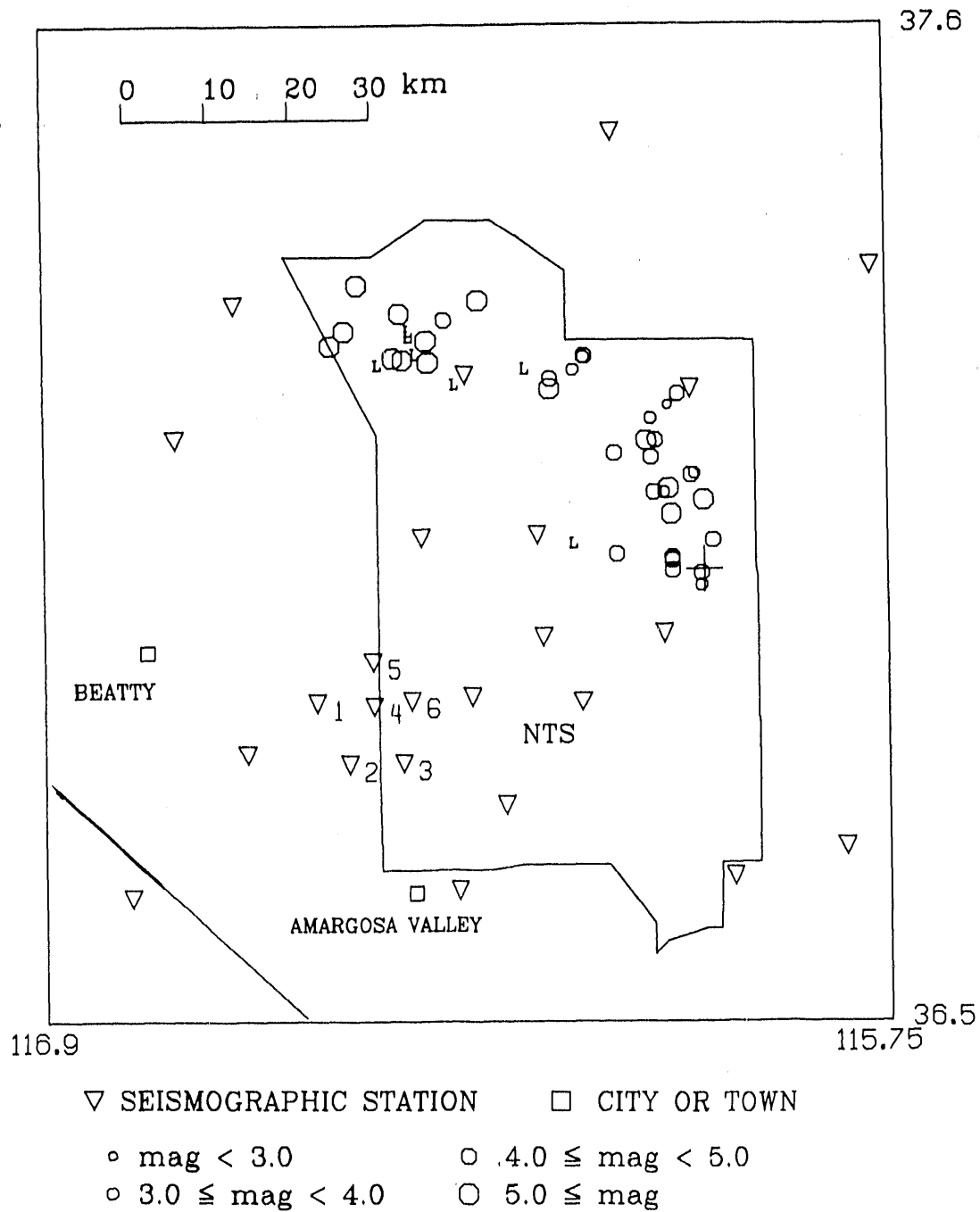
Figure C1. Map of announced NTS nuclear device detonation epicenters for the period 1987 through 1989 (test epicenters are octagons), and of epicenters of a small subset of the low-coda frequency activity (aftershocks?, collapses?) that followed those UNEs (designated by "L" symbols).
