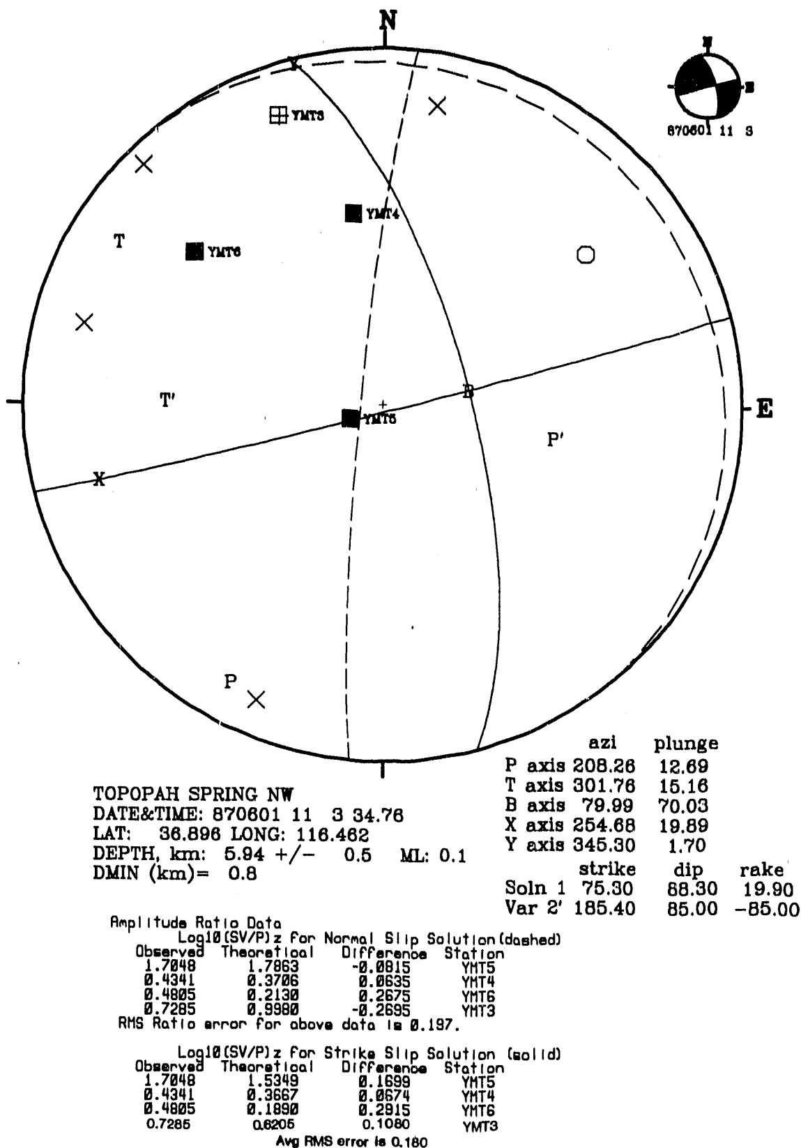
Figure D7. A very different pair of focal mechanism solutions for a very small earthquake of June 1, 1987, at Yucca Mountain, Nevada, both of which are constrained by several SV/P_z amplitude ratios.
