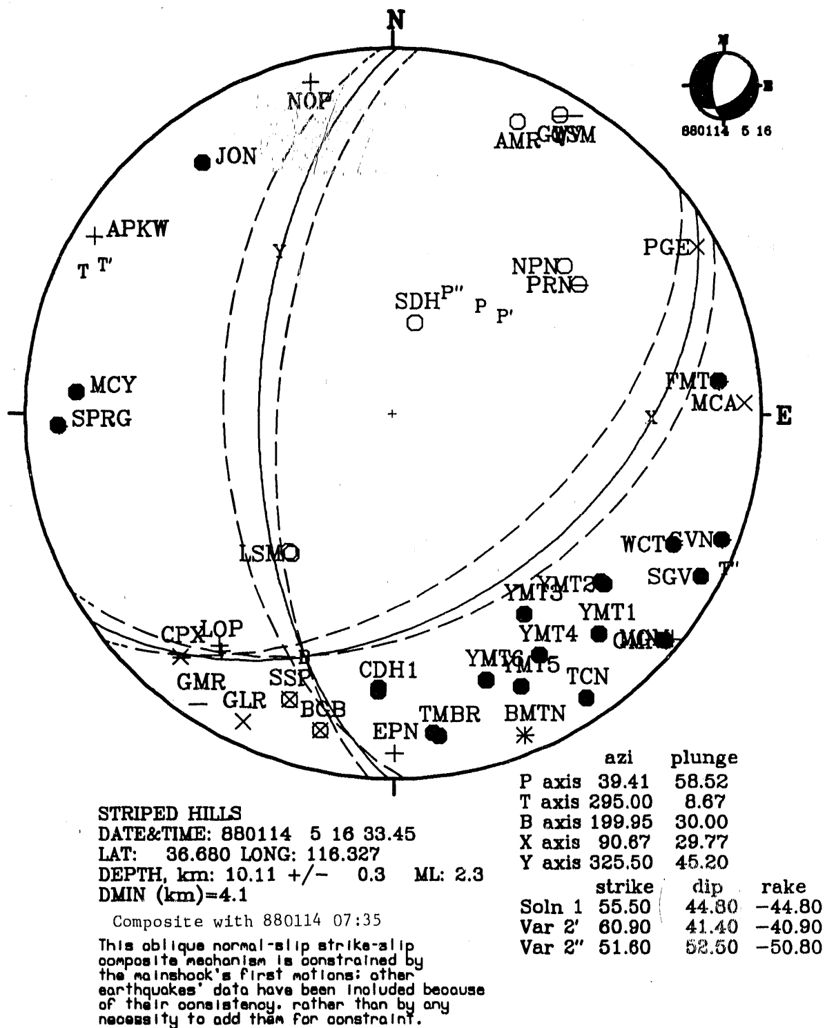
Figure D16. A composite oblique normal-slip set of focal mechanism solutions for a pair of earthquakes on January 14, 1988, in the Striped Hills, about 20 km south of Yucca Mountain, Nevada.
