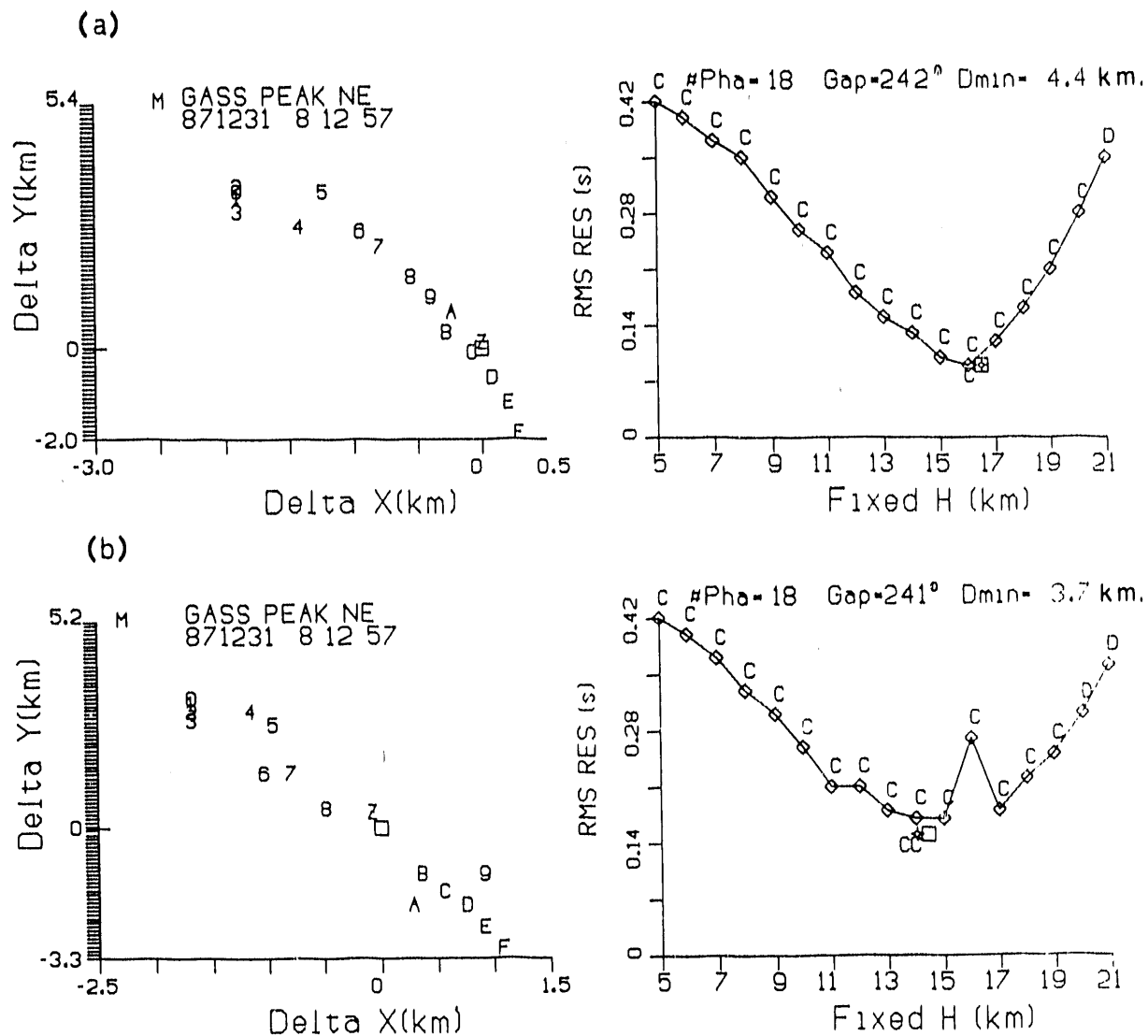
Figure 20.- Left side , epicentral scatter and right side , behavior of RMS as a function of fixed-depth and free-depth HYPO71 solutions, with symbols having same meanings as in Figures 10 and 14, for an earthquake north of Las Vegas, Nevada, on December 31, 1987 8:12 UTC having probable depth of focus near the brittle-ductile transition. (a) Hypocenters derived using a model with no interface at 15 km below sea level, V_p = 6.15 km/sec between 3 and 24 km below sea level, (b) Hypocenters derived using a model with an interface at 15 km below sea level, V_p = 6.5 km/sec below that interface (see Figure F1(a) for the velocity model). This figure shows that in some instances, the 15 km interface, or the relatively high velocity below that interface, is not well supported by arrival time data.
