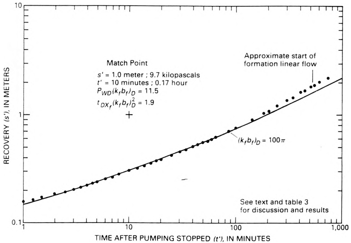
Figure 18.--Analysis of recovery test 4, depth interval from 704 to 1,219 meters, vertical-fracture model, curve-match method.
