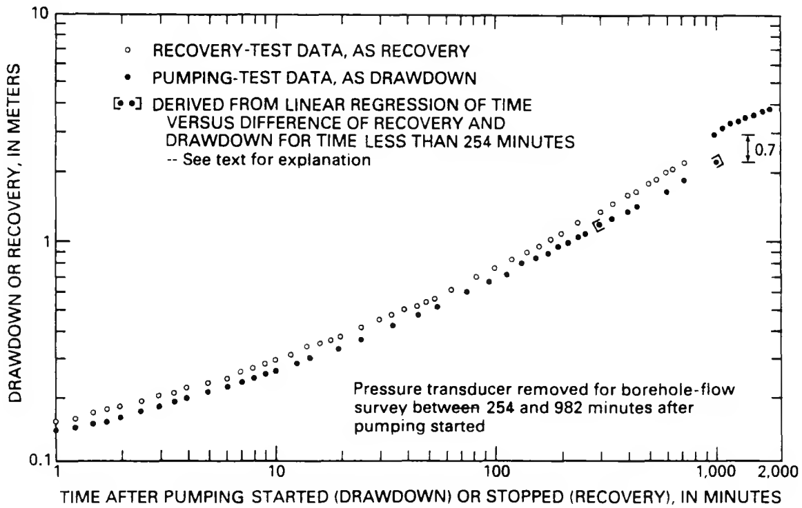
Figure 11.--Data for pumping and recovery tests 4, depth interval from 704 to 1,219 meters.
