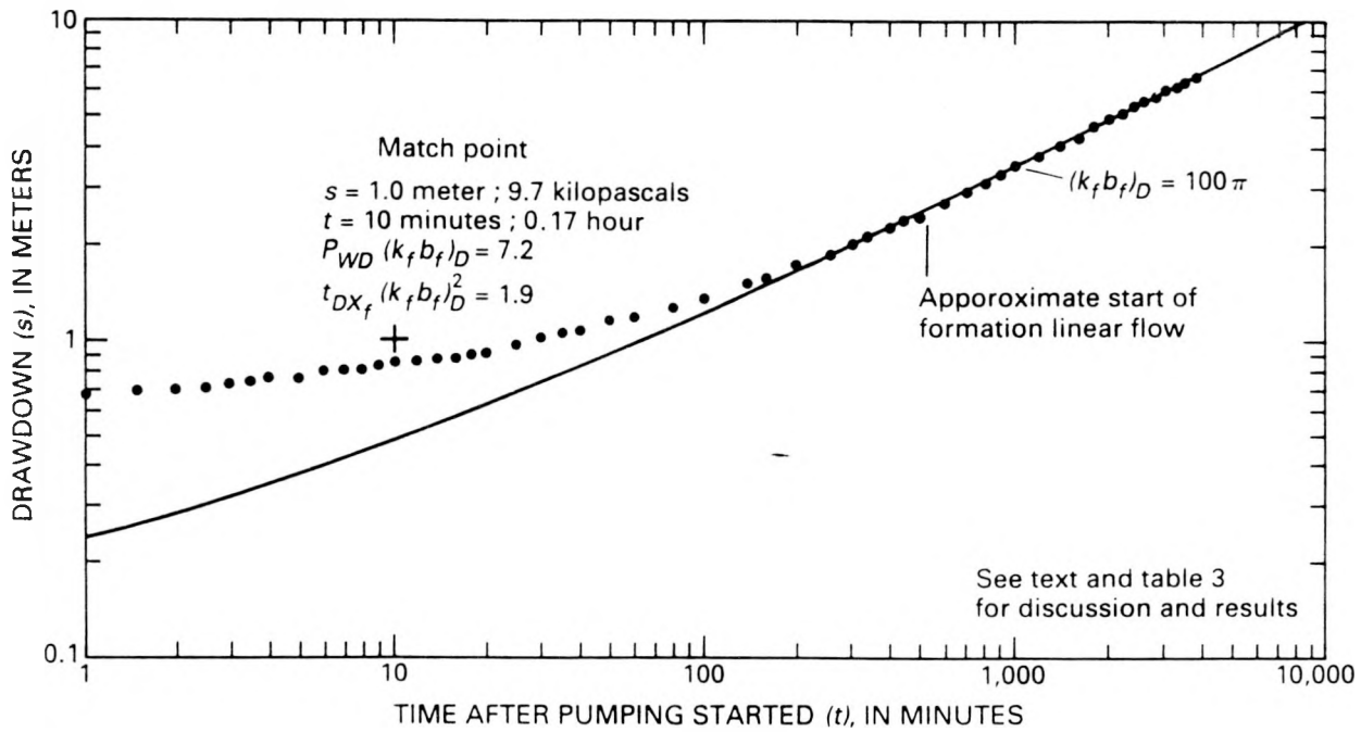
Figure 16.--Analysis of pumping test 3, depth interval from 704 to 1,219 meters, vertical-fracture model, curve-match method.
