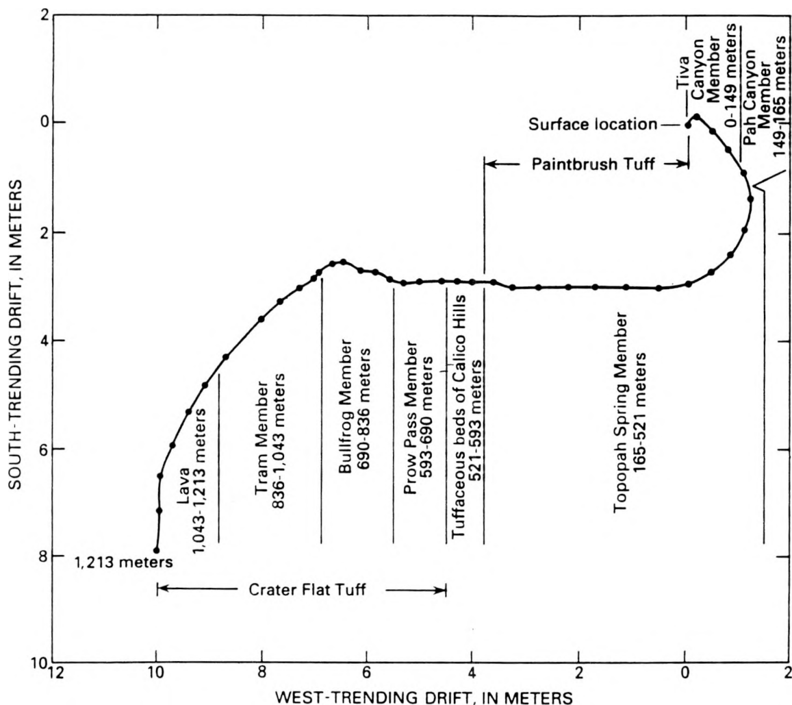
Figure 3.--Subsurface survey of borehole showing horizontal drift from surface location.
