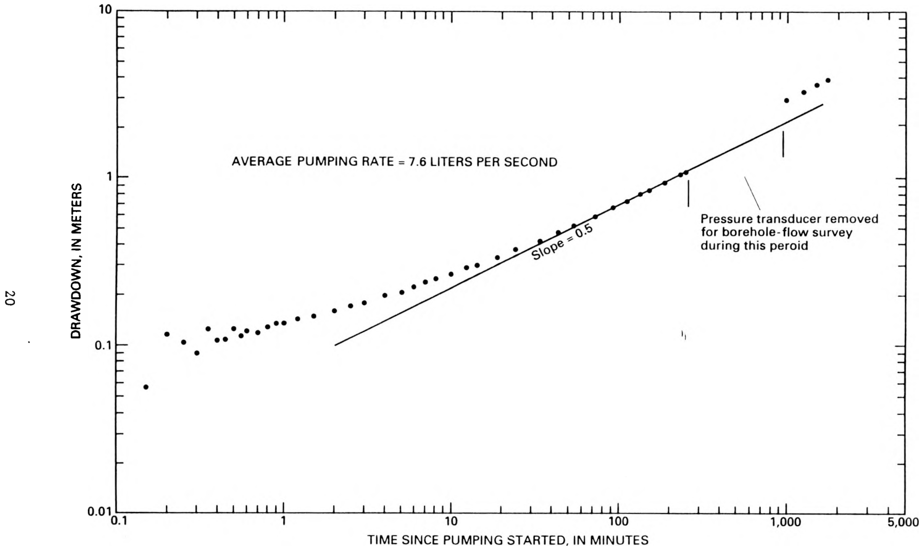
Figure 10.--Water-level drawdown, pumping test 4, depth interval from 704 to 1,219 meters.
