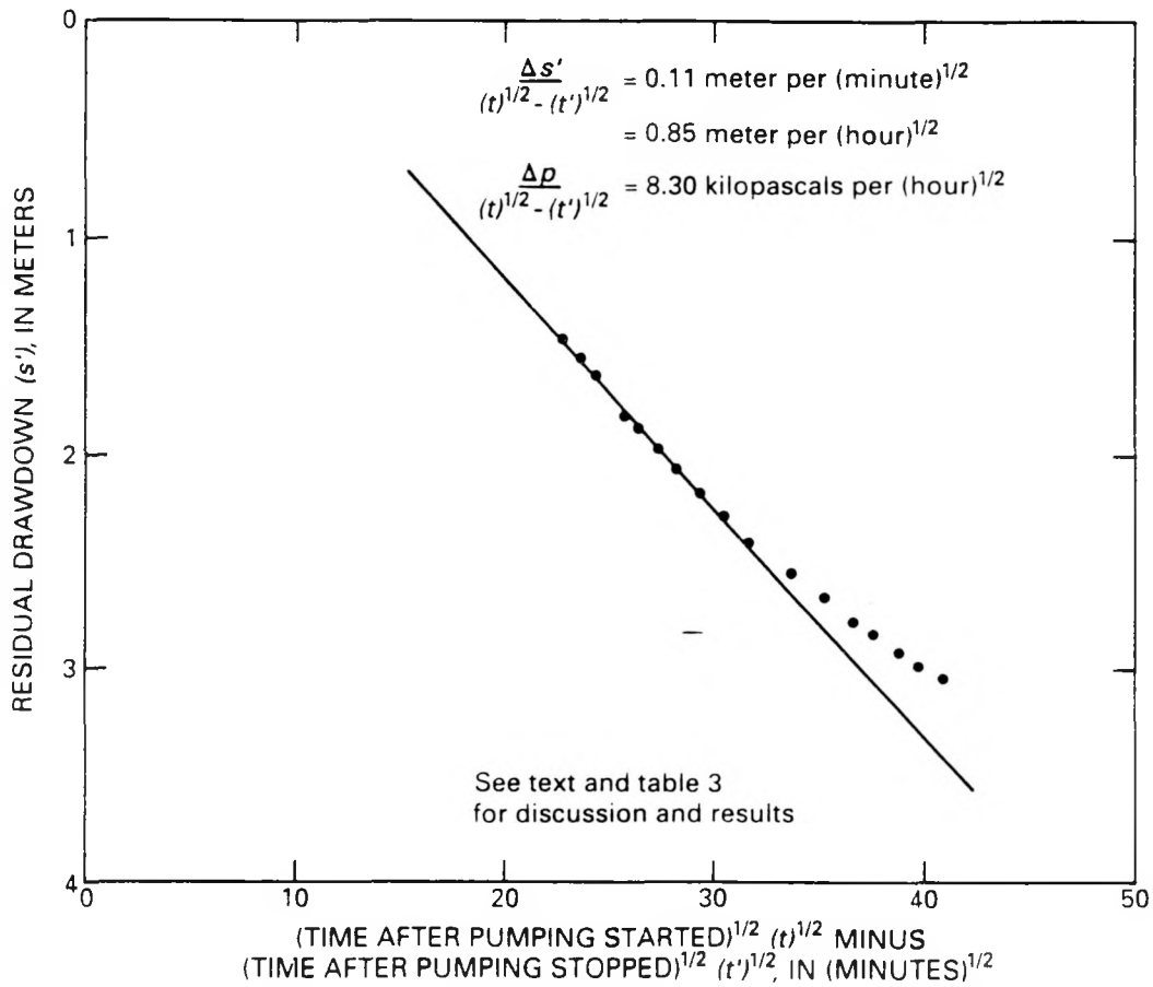
Figure 24.--Analysis of recovery test 4, depth interval from 704 to 1,219 meters, vertical-fracture model, linear-flow method.
