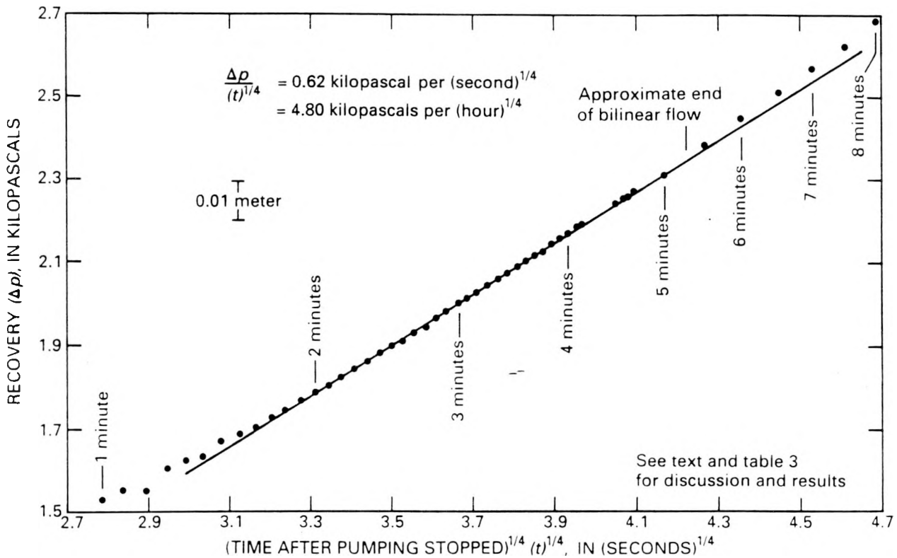
Figure 20.--Analysis of recovery test 4, depth interval from 704 to 1,219 meters, vertical-fracture model, bilinear-flow method.
