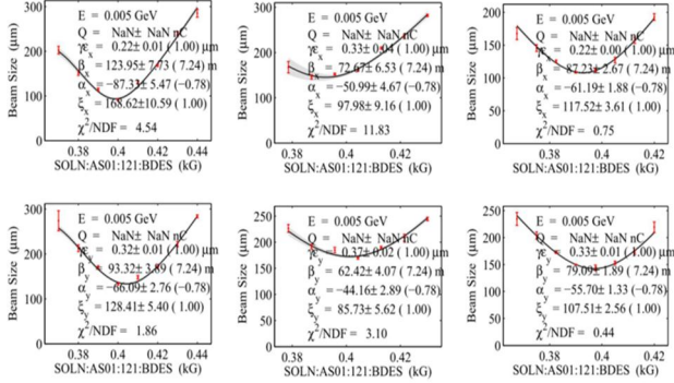
Figure 6: Intrinsic emittance 0.22-μm (x)/0.32-μm (y) before laser cleaning (left), 0.33-μm (x)/0.37-μm (y) immediately after laser cleaning (middle), and 0.22-μm (x) /0.33 -μm (y) on the second day after laser cleaning (right).
