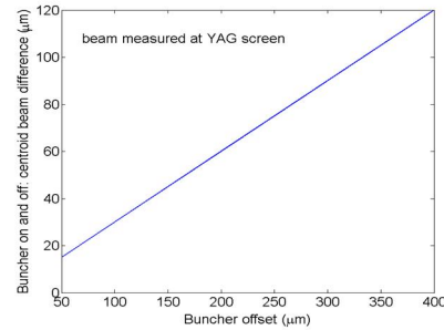
Figure 4: Transverse beam displacement difference between buncher on/off vs. buncher offset.
