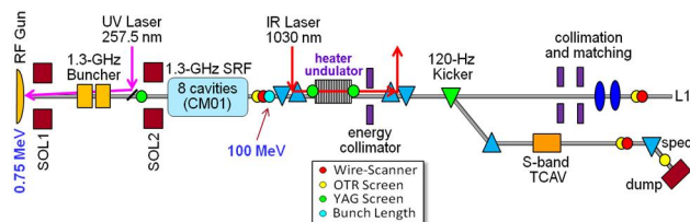
Figure 1: Schematic of the full LCLS-II injector.
