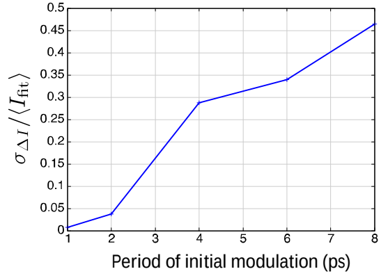
Figure 3: density modulation at the undulator entrance vs. photocathode laser modulation period with fixed \pm 5\% of amplitude change [2].
