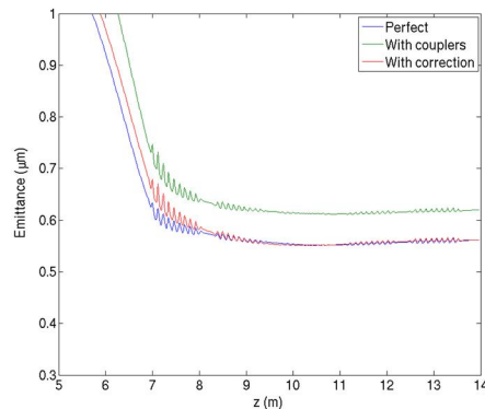
Figure 2: LCLS-II injector emittance with perfect RF field, with RF couplers field and correction using a quadrupole for 300 pC [1].
