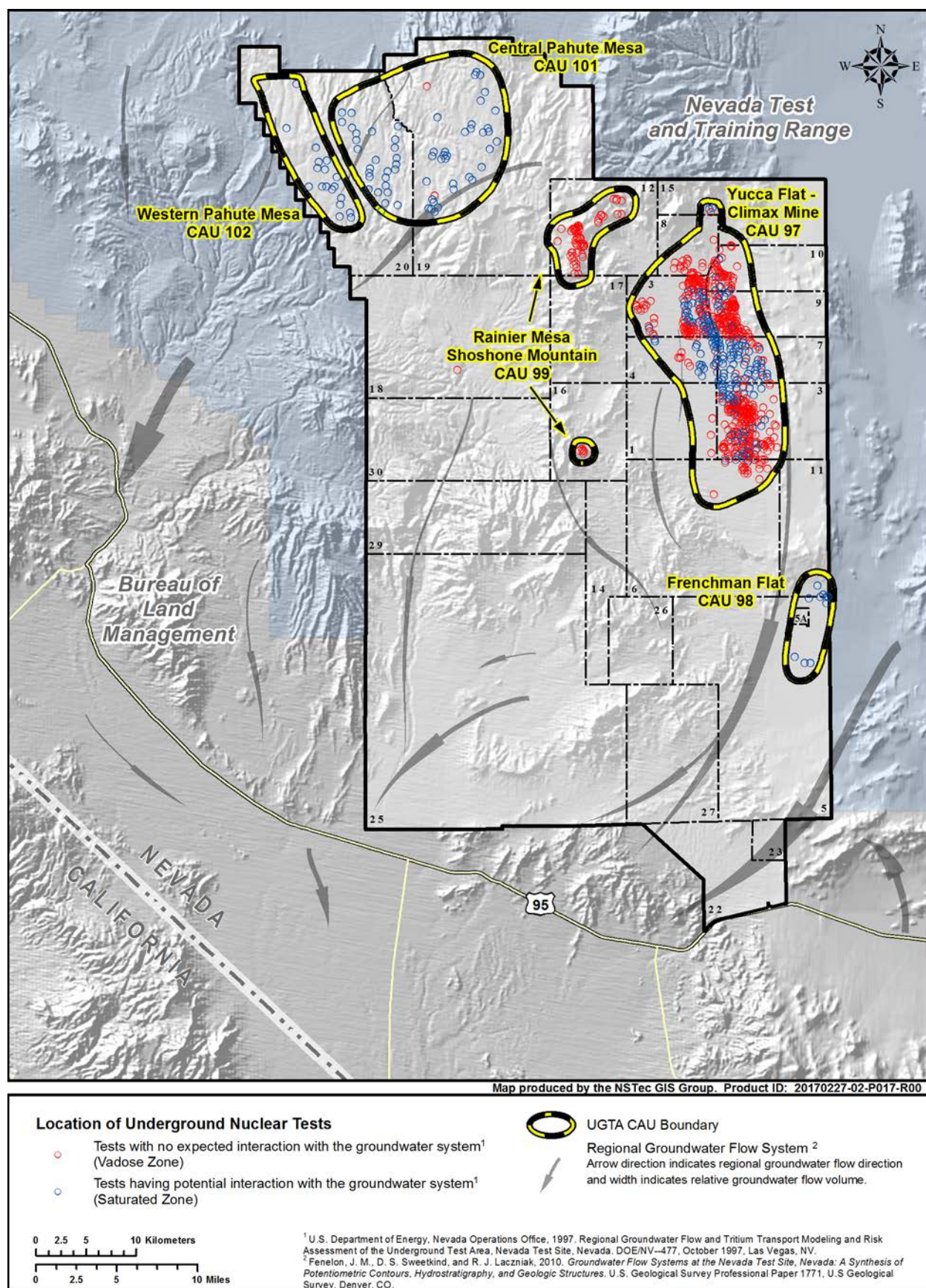
Figure A-7. Location of UGTA corrective action units (CAUs) and historical underground nuclear tests on the NNSS
