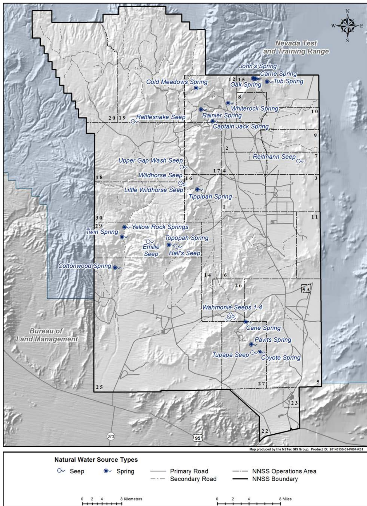
Figure A-4. Natural springs and seeps on the NNSS (adapted from Hall et al. 2017)
