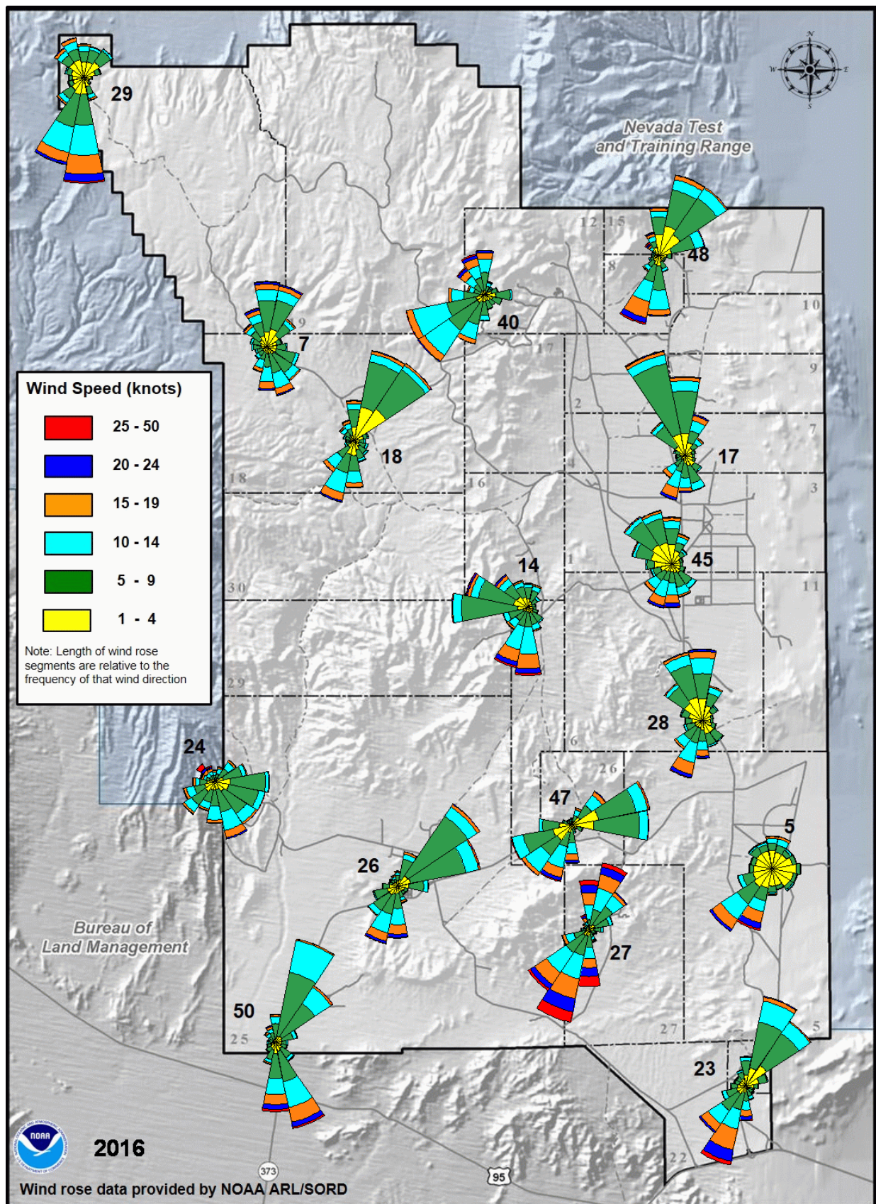
Figure A-18. Wind rose climatology for the NNSS (2005-2016)
