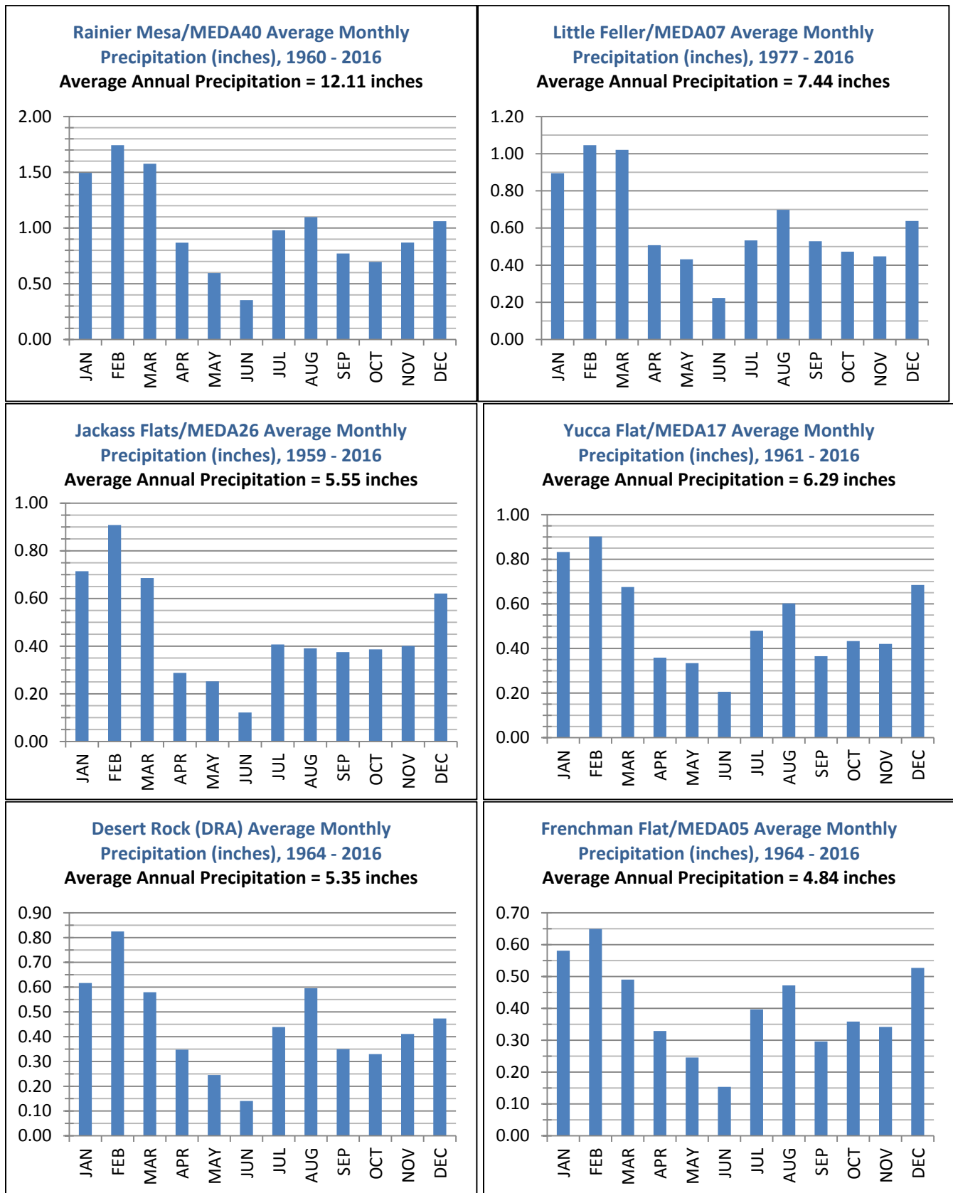
Figure A-16. Mean monthly precipitation at six NNSS rain gauge stations (location of numbered stations are shown in Figure A-14)
