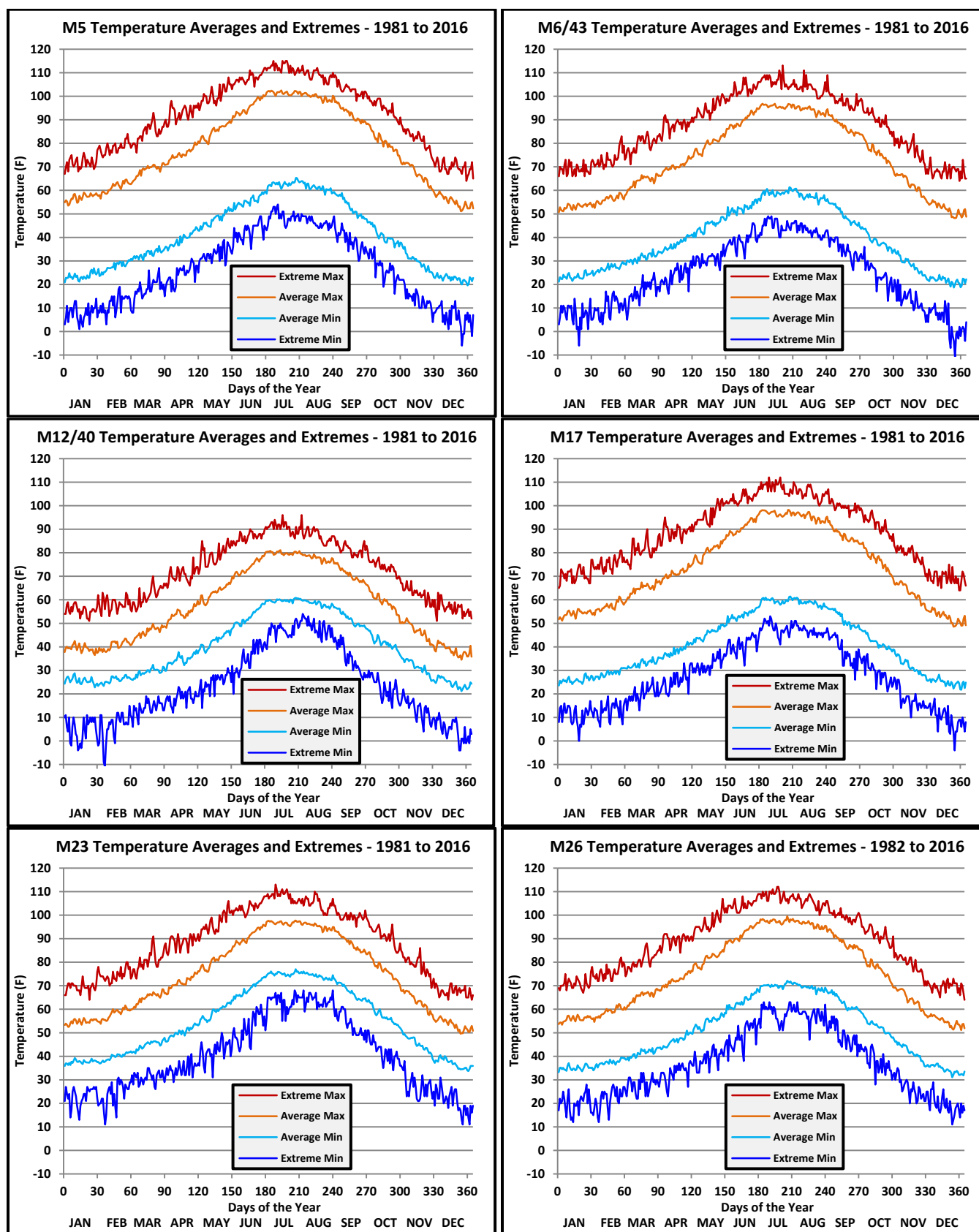
Figure A-17. Temperature extremes and average maximums and minimums at six NNSS MEDA stations (location of numbered stations are shown in Figure A-14)
