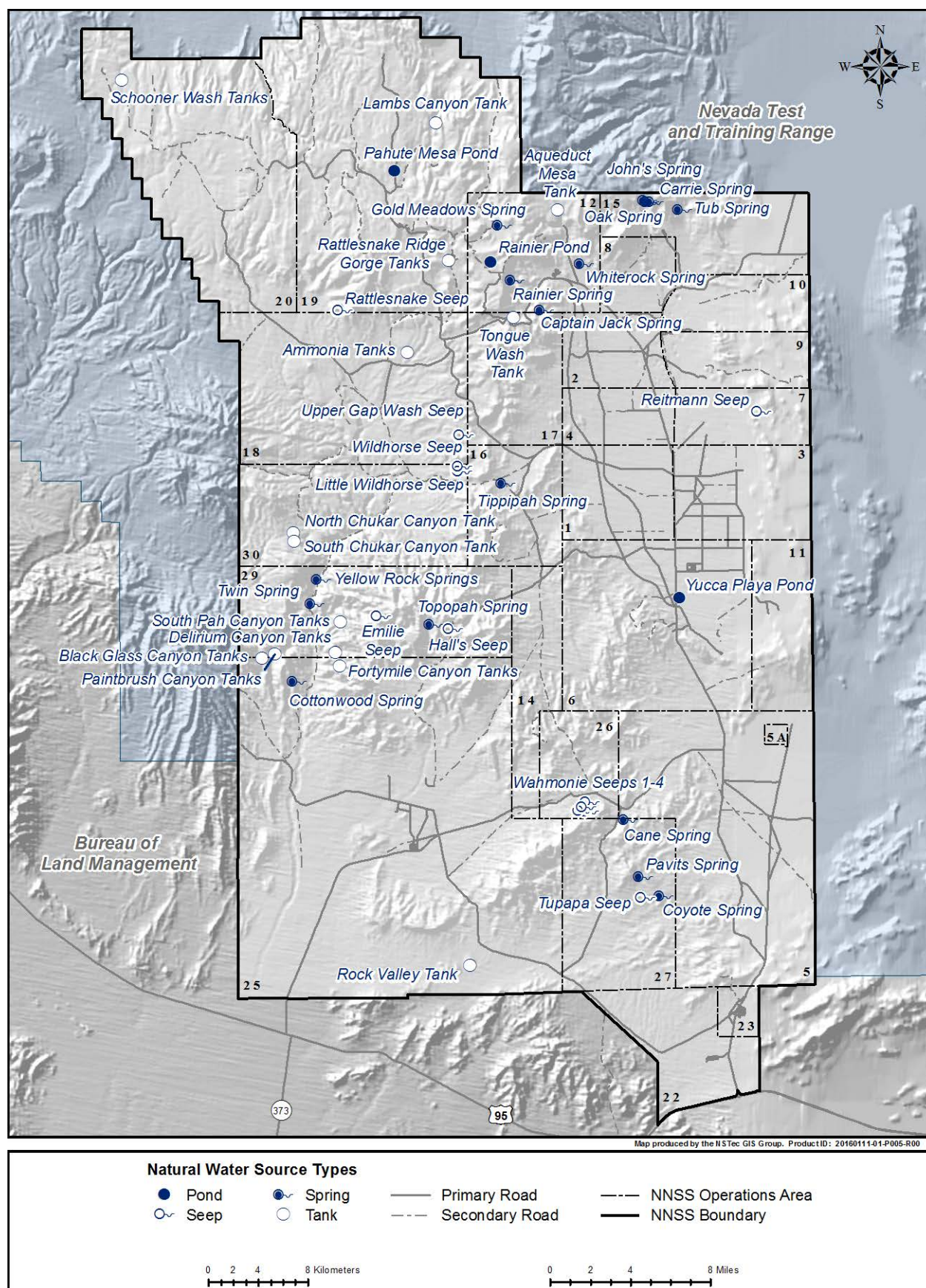
Figure A-21. Natural water sources on the NNSS (from Hall et al. 2017)
