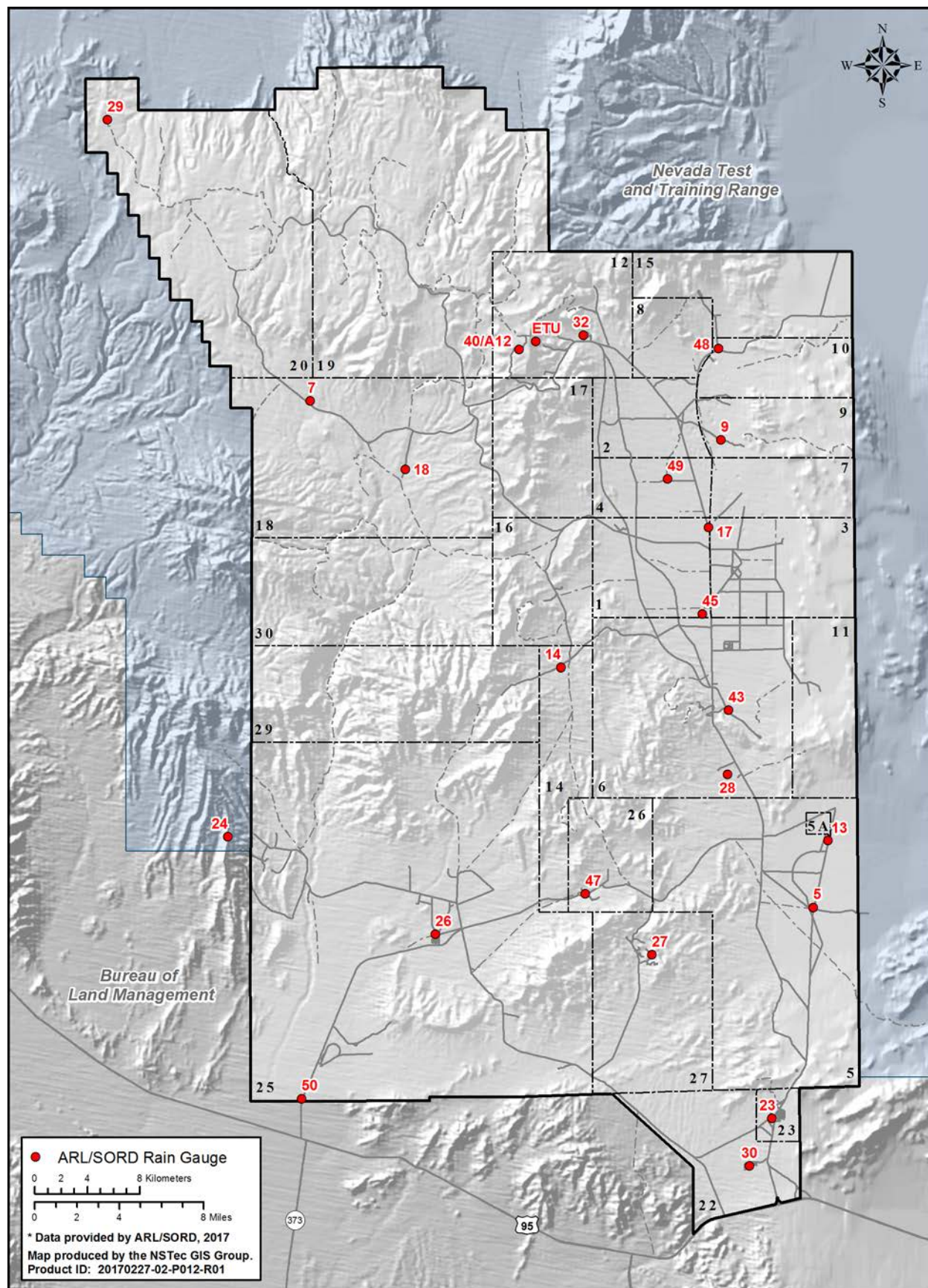
Figure A-15. 2016 climatological rain gauge network on the NNSS
