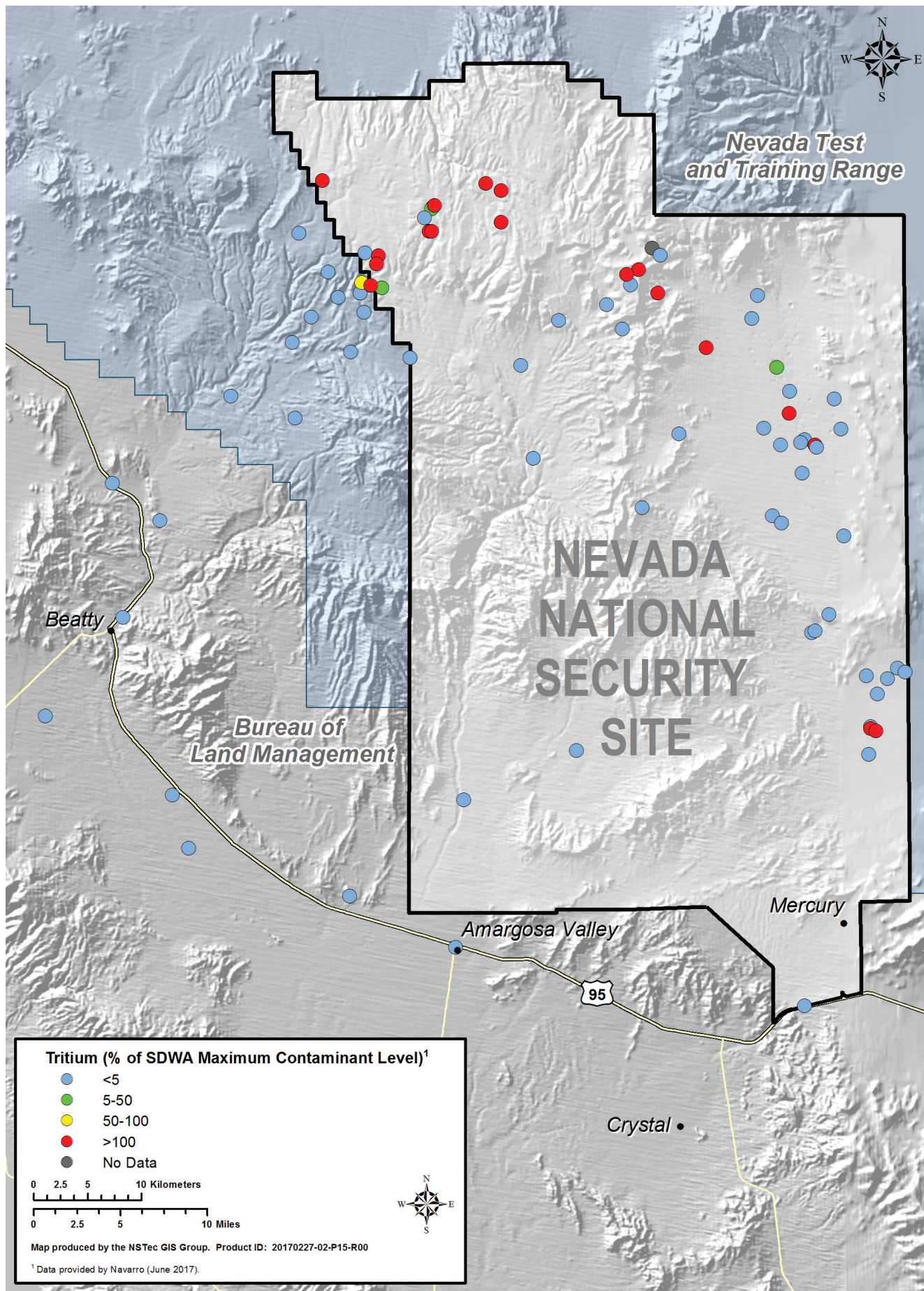
Tritium in NNSA/NFO Groundwater Monitoring Wells
