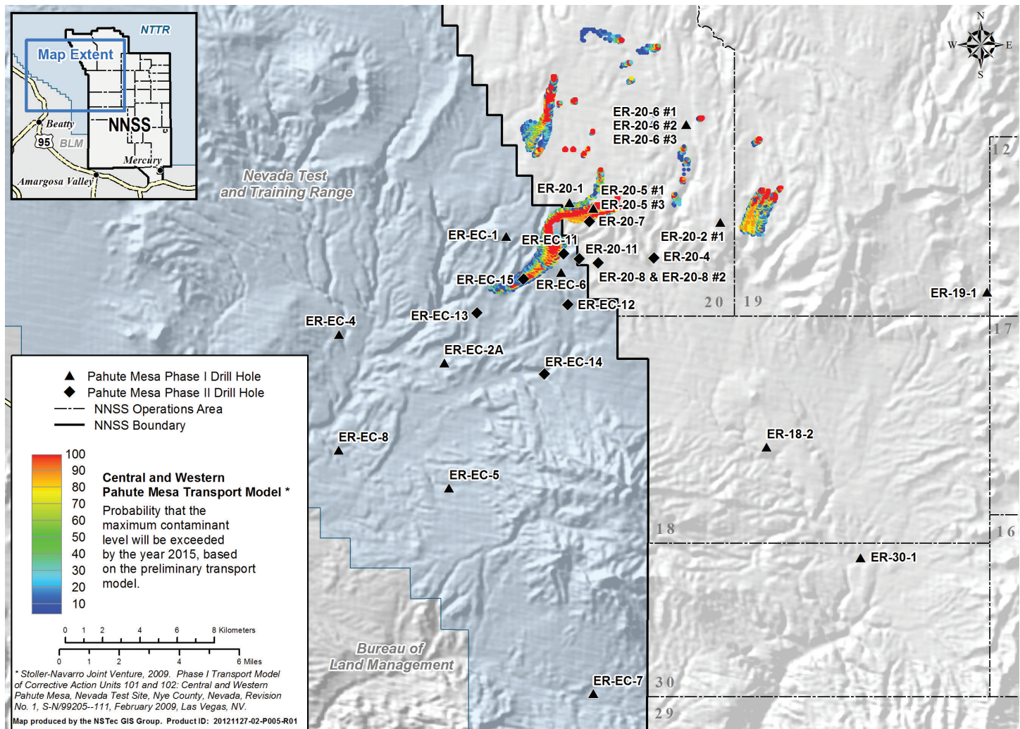
Results of 2009 Phase I Central and Western Pahute Mesa Transport Modeling
