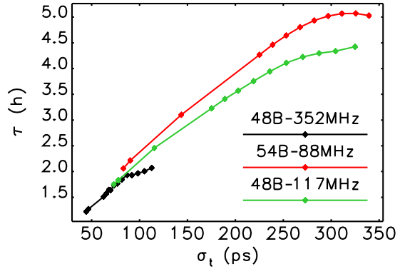
Figure 6: 10 th -percentile beam lifetime as a function of rms bunch length for various fundamental rf frequency choices. A gas-scattering lifetime of 60 h is included [21].
