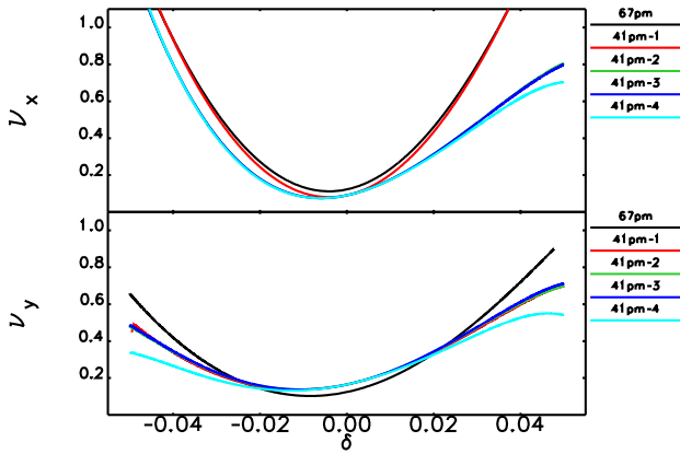
Figure 2: Momentum tune footprints for several variants of the 41-pm lattice compared to the 67-pm lattice.
