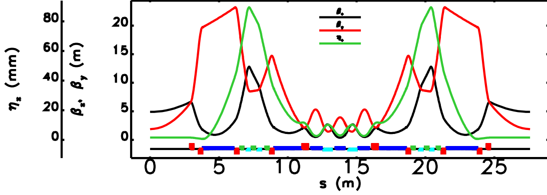
Figure 1: Lattice functions for the 41-pm lattice with reverse bends. Dipoles are blue (normal) and cyan (reverse), quadrupoles are red, and sextupoles are green.
