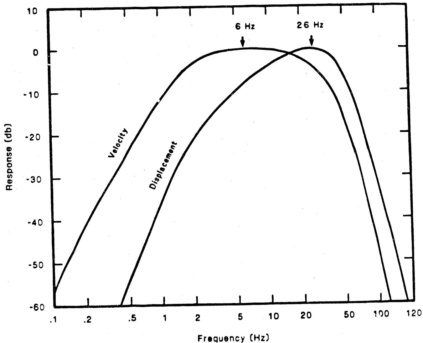
Figure 1.9. Theoretical Transfer-function curves for the USGS short-period seismic refraction system (both recorder and digitizer). Solid lines are the displacement and velocity normalized amplitude. (From Dawson and Stauber, 1986)
