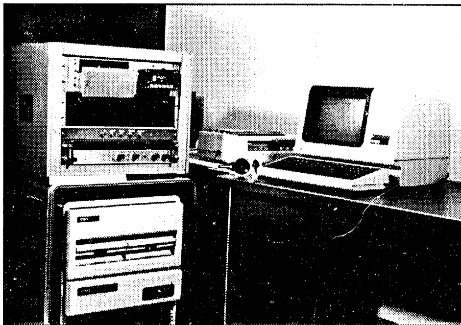
Figure 1.4. Digitizing unit.
