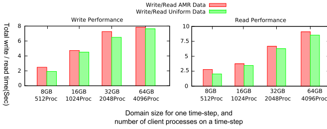
Fig. 9. Results of boxes write/read performance testing for AMRZone over real AMR datasets, with comparisons on synthetic uniform data, totally 10 time-steps. In the worst case, AMR data related task demands more than 36% additional execution time, in the best case it is 2% more. In 5 cases (out of 8), AMR data coupled write/read needs less than 10% more time. Note these are not weak scaling testings.
