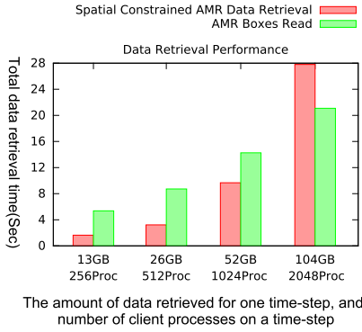
Fig. 12. Results of spatially constrained data retrieval performance testing for AMRZone over AMR datasets, with comparisons of AMR boxes read, totally 10 time-steps. Note these are not weak scaling testings.
