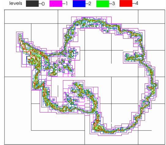
Fig. 1. The visualization graph of a 1GB block-structured AMR dataset generated by BISICLES [11]. The coarsest (or lowest) level (level 0) covers the entire global data domain. A finer (or higher) level is generated by refining a set of boxes on the adjacent coarser level, only covering some sub-regions of interest with higher resolution which is defined by a refinement ratio. The boxes at the finer levels represent spatial regions of more interest.
