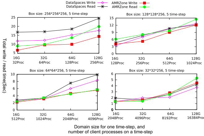
Fig. 7. Results of weak scalability comparison experiments between AMRZone and DataSpaces, over 5 time-steps. AMRZone generally performs better compared to DataSpaces (22 out of 32 cases). In the best case, it could achieve about 46% performance improvement, in the worst case there is about 35% performance reduction.
