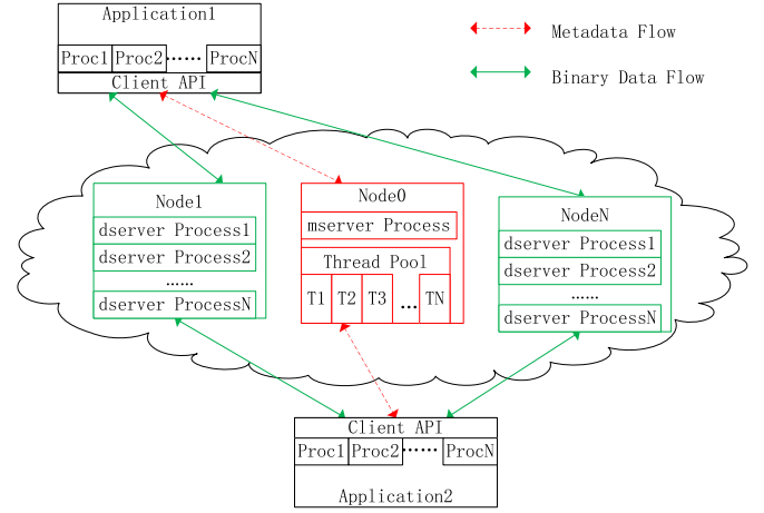
Fig. 3. The client-server architecture of AMRZone consists of two types of server processes: (1) mservers that only manage metadata, recording how AMR boxes are distributed across dservers and constructing spatial index; and (2) dservers that only manage the binary data. Note that Application1 and Application2 could be simulations or other data analytics programs. Also note that AMRzone does not limit the number of applications that can connect to the server side.
