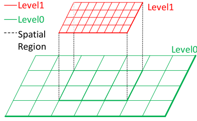
Fig. 4. A spatial query over AMR data. Typically, boxes are retrieved in multiple levels, rather than a single level. The boxes at level 1 are refined from bigger boxes at level 0.
