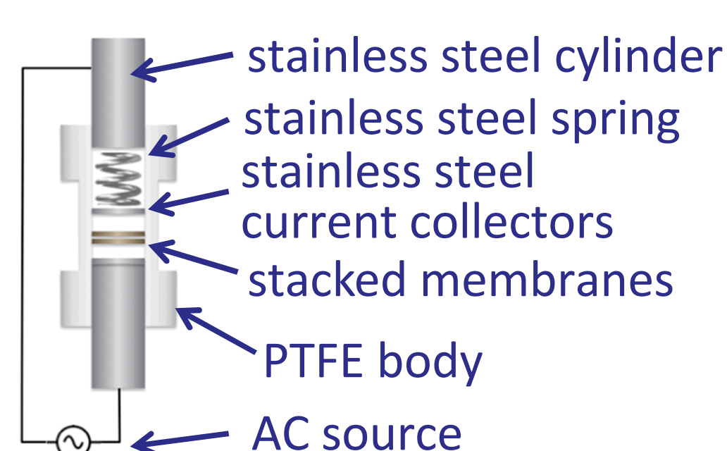
Membrane Conductivity Cell
