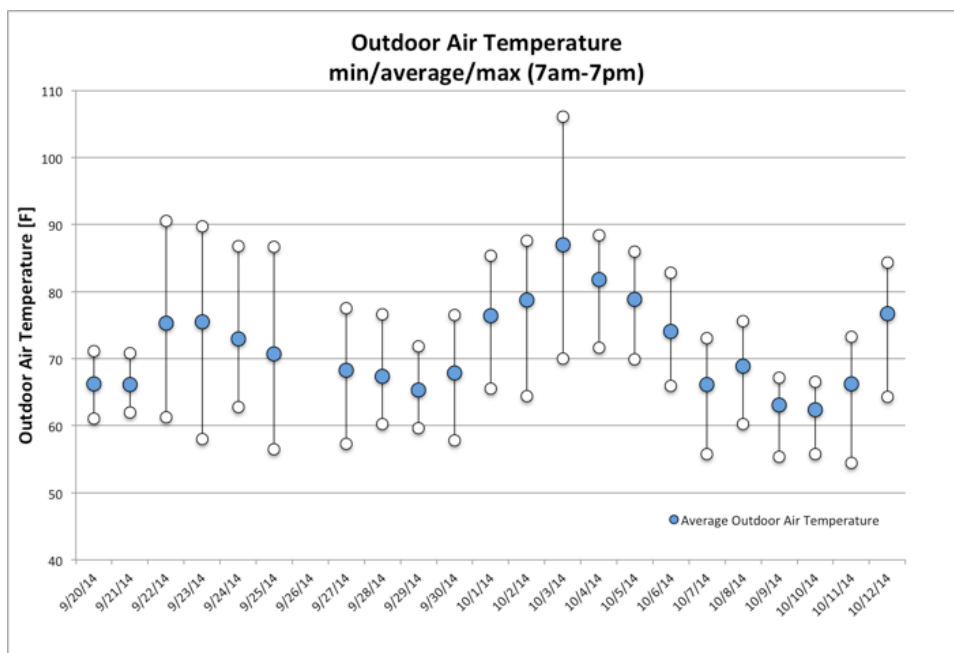
Figure 8.7 – Daily outdoor air temperature, min,avg,max (7am-7pm)
