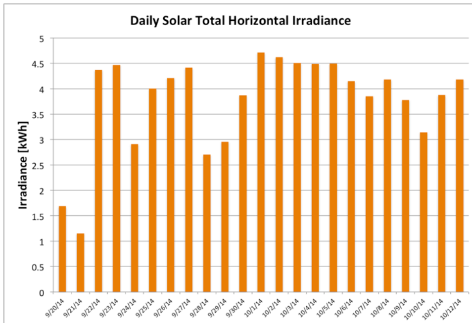
Figure 8.6 – Daily solar total global horizontal irradiance (7am-7pm)
