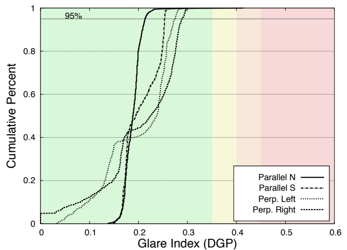
Figure 8.27 - Glare class ratings for views of the the east facade between October 4 and 10.
