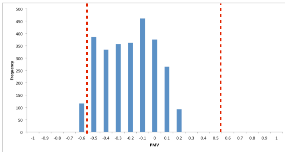
Figure 8.16 - Predicted Mean Vote histogram for the west façade – 42" from glass, September 22 nd – 25 th
