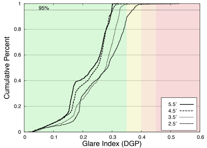
Figure 8.30 - Visual comfort rating at each camera position for the west facade (table above). Cumulative distribution chart for each camera position (right).
