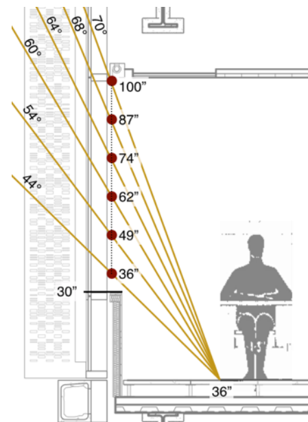
Figure 7.10 - Section detail illustrating the proposed shade stops. The lowest stop is 36" above the floor, 6" above the sill. Seated eye height is typically 44-48 inches above the floor.
