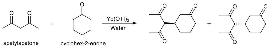
Figure 13. Michael addition of acetylacetone with cyclohex-2-enone in water catalyzed by a ytterbium(III) triflate Lewis acid catalyst. [46]
