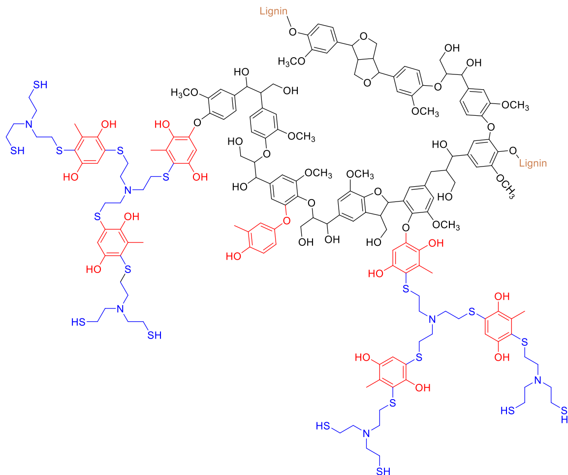
Figure 88. Proposed structure of lignin-core hyperbranched copolymers.
