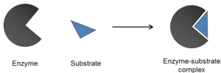
Figure 23. “Lock-and-key” model of enzyme-substrate interaction.
