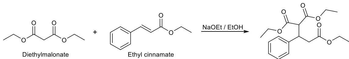
Figure 3. Michael addition of diethylmalonate with ethyl cinnamate. [24]
