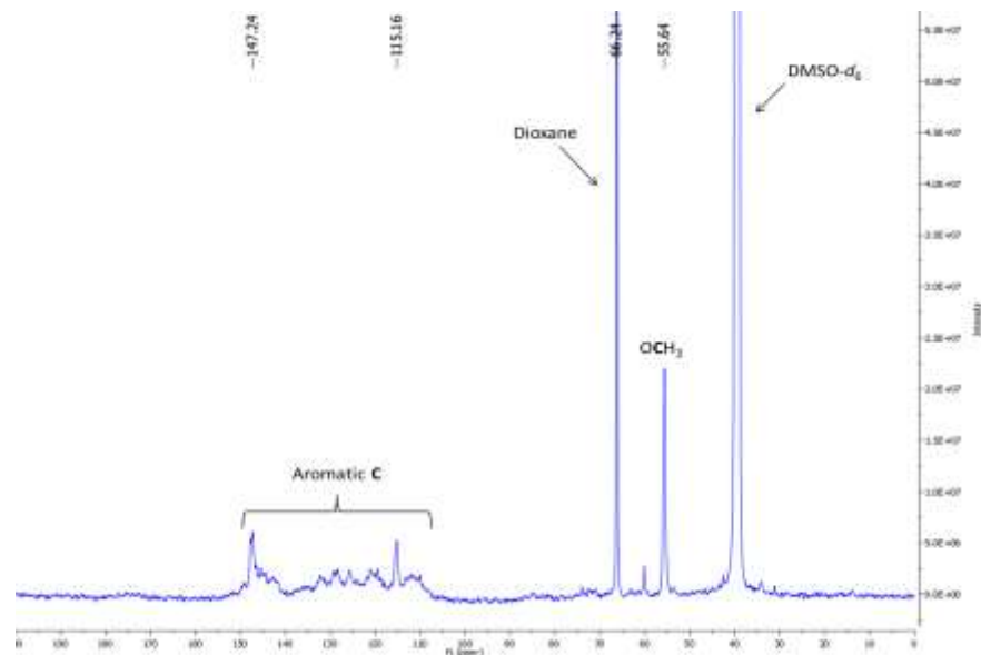
Figure 82. a) ^1\text{H} NMR spectrum and b) ^{13}\text{C} NMR spectrum of purified kraft lignin.
