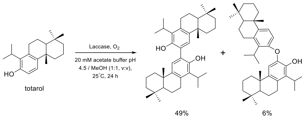
Figure 39. Laccase-catalyzed dimerization of totarol. [156]
