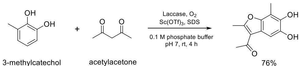
Figure 43. Laccase-catalyzed coupling of 3-methylcatechol with a 1,3-dicarbonyl. [183]
