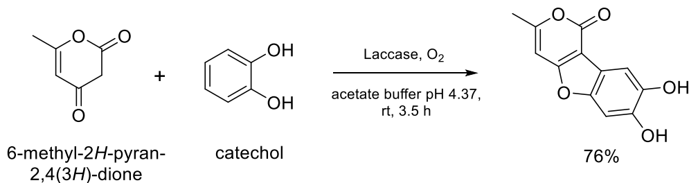
Figure 42. Laccase-catalyzed coupling of catechol with a heterocyclic 1,3-dicarbonyl. [181]
