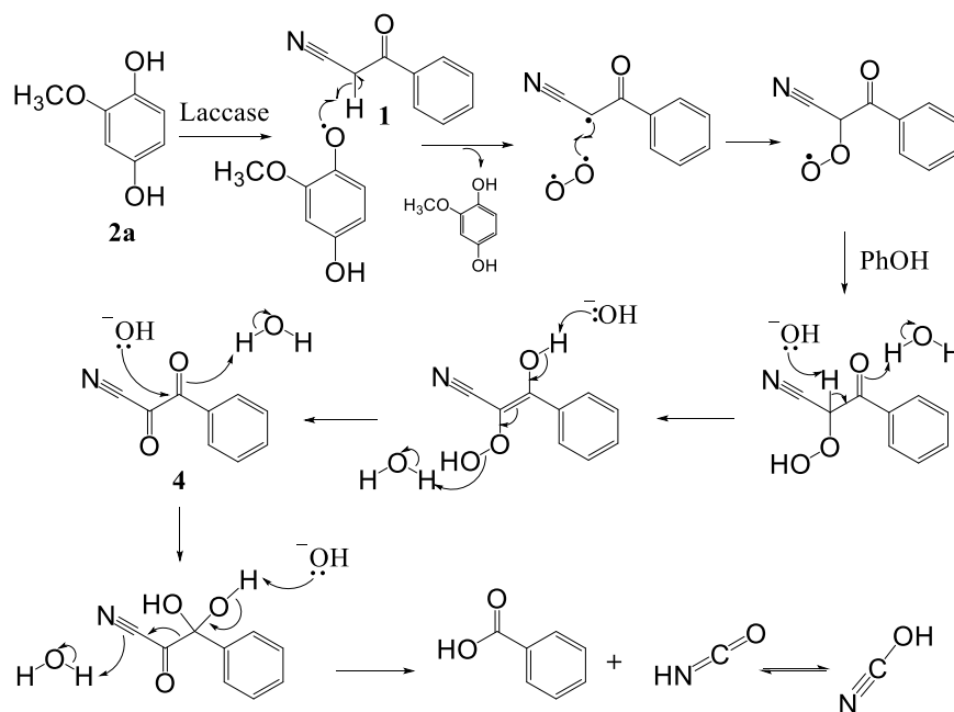
Figure 66. Proposed mechanism for the oxidative degradation of 1 to form benzoic acid and isocyanic/cyanic acid via 1,2-dicarbonyl intermediate 4 .
