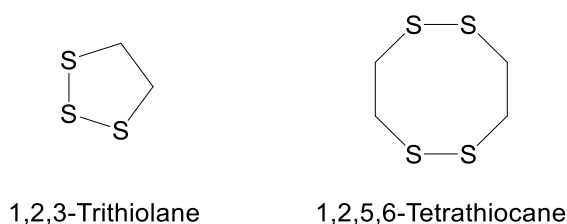
Figure 74. Side products of the laccase-catalyzed reaction of 1,2-ethanedithiol ( 9 ) with substituted hydroquinones ( 2 ).
