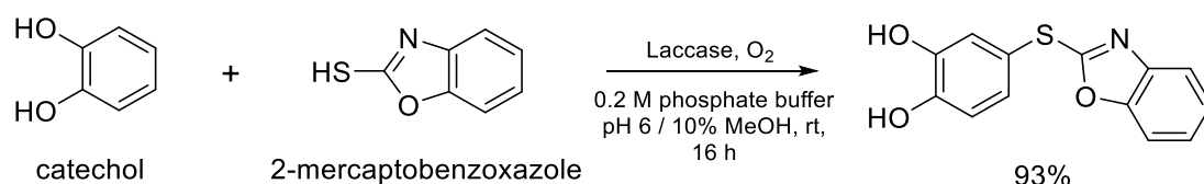
Figure 50. Laccase-catalyzed coupling of catechol with 2-mercaptobenzoxazole. [221]
