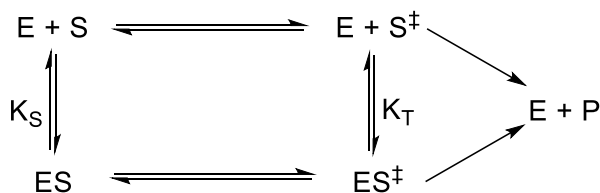
Figure 25. Thermodynamic cycle illustrating transition-state stabilization in enzymatic catalysis. [70]
