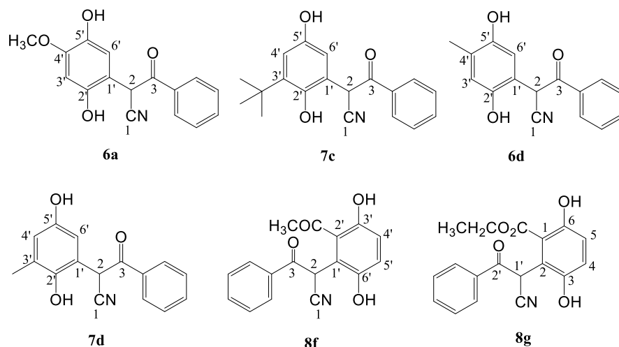
Figure 68. Structures of the products formed by the laccase-catalyzed reaction of benzoylacetoneitrile (1) with substituted hydroquinones (2).
