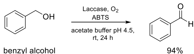
Figure 52. LMS ABTS oxidation of benzyl alcohol to benzaldehyde. [140]
