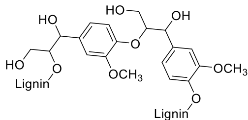
Figure 57. The \beta -O-4 linkage in softwood lignin.
