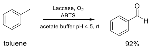
Figure 53. LMS ABTS oxidation of toluene to benzaldehyde. [139]
