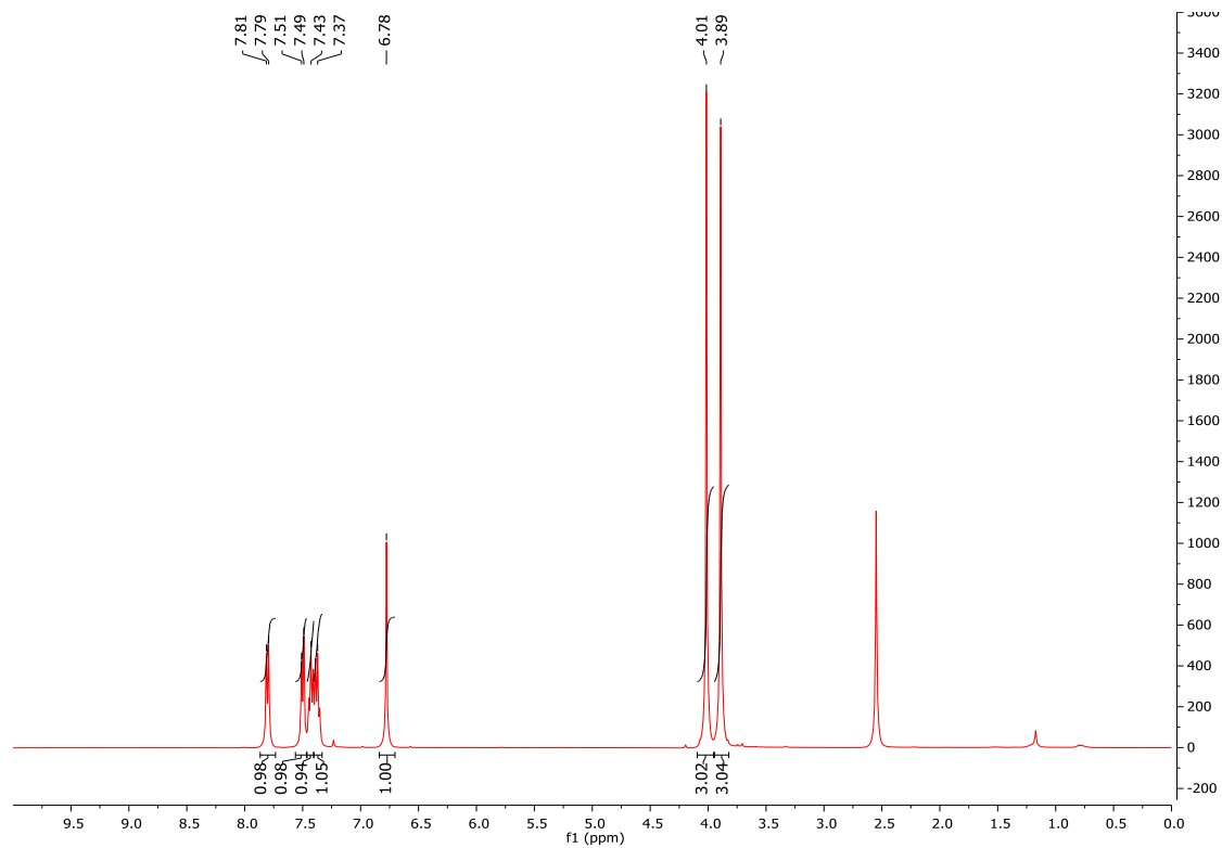
Figure A28. ^1\text{H} NMR spectrum of compound 15c.
