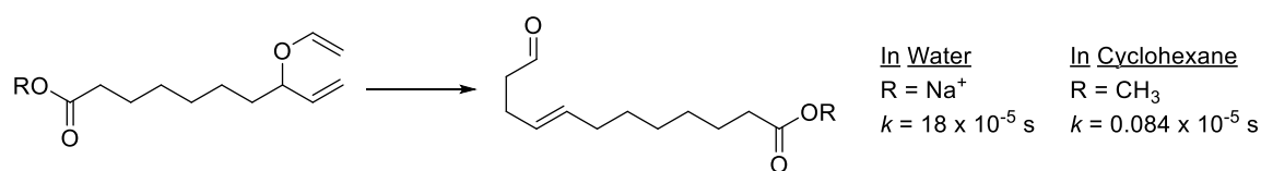
Figure 6. Claisen rearrangement of an allyl vinyl ether. [30]
