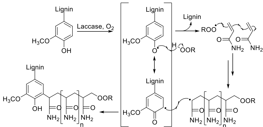
Figure 61. Reaction mechanism for the laccase-initiated copolymerization of lignin with acrylamide (adapted from Mai et al. 1999). [248, 269]
