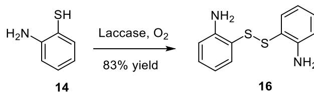
Figure 77. Laccase-catalyzed dimerization of 2-aminothiophenol ( 14 ). Reaction conditions: 0.50 mmol 14 , 50 U laccase, 6 mL 0.10 M sodium acetate buffer pH 5.0, rt, 4 h.
