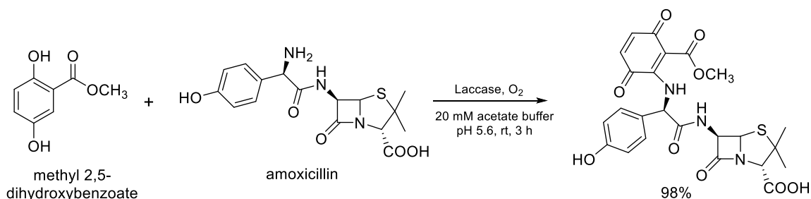
Figure 47. Laccase-catalyzed coupling of methyl 2,5-dihydroxybenzoate with amoxicillin. 208
