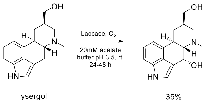
Figure 54. Laccase-mediated stereoselective C-4 hydroxylation of lysergol. [245]
