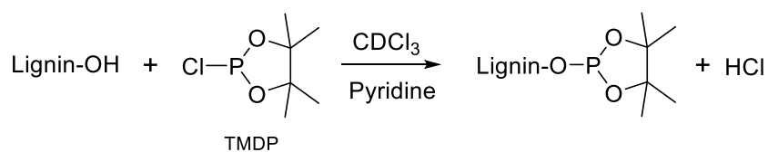
Figure 84. Phosphitylation of lignin with TMDP.
