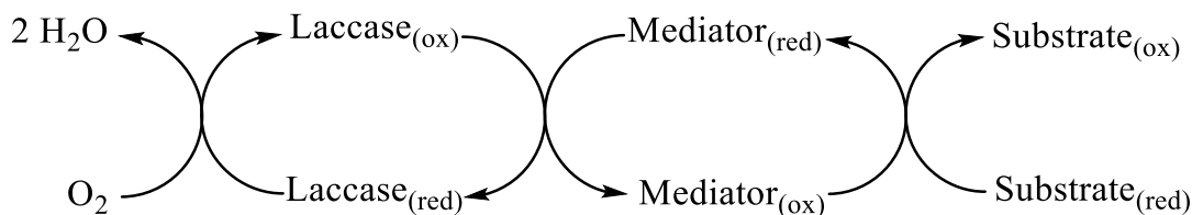
Figure 34. Laccase-mediator system (LMS). [94]
