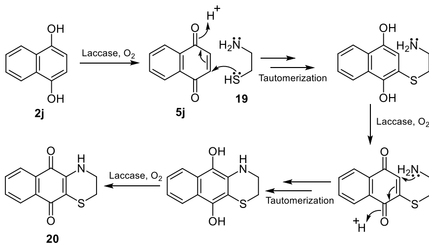
Figure 81. Reaction mechanism for the laccase-catalyzed coupling of naphthohydroquinone ( 2j ) with cysteamine ( 19 ).
