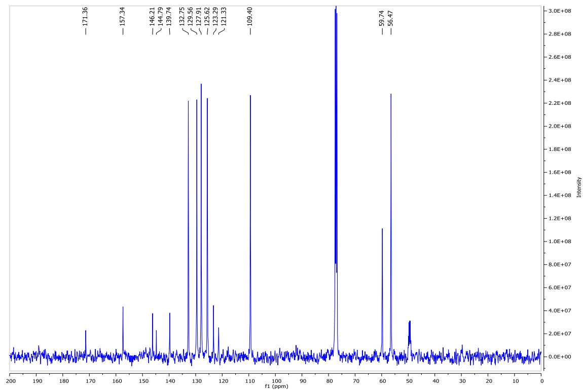
Figure A29. ^{13}\text{C} NMR spectrum of compound 15c.
