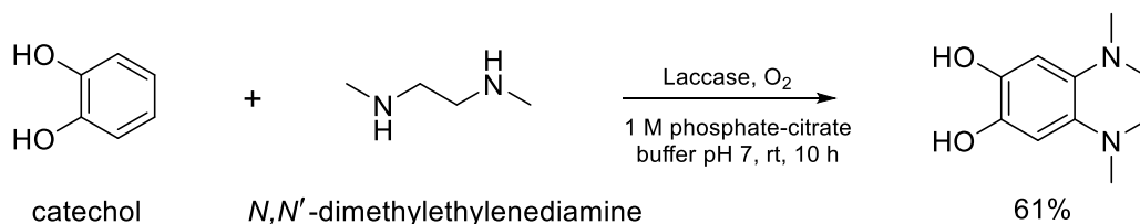
Figure 48. Laccase-catalyzed coupling of catechol with N,N' -dimethylethylenediamine. [218]
