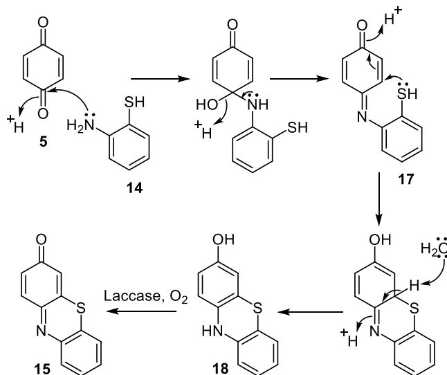
Figure 79. Reaction mechanism for the laccase-facilitated synthesis of phenothiazones.
