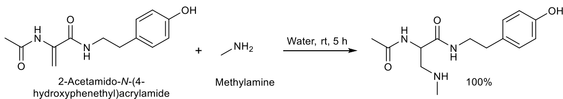
Figure 8. Michael addition of methylamine to a dehydroalanine amide in water. [32]
