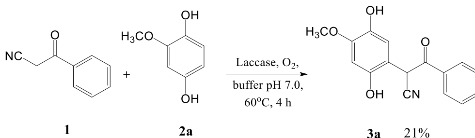
Figure 65. Initial reaction of benzoylacetone nitrile ( 1 ), 1 mmol, with methoxyhydroquinone ( 2a ), 0.25 mmol.
