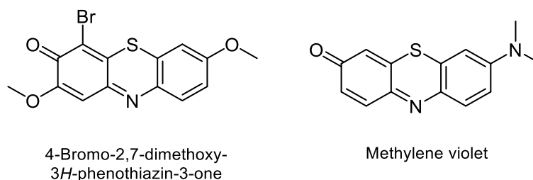
Figure 75. Representative structures of phenothiazones.
