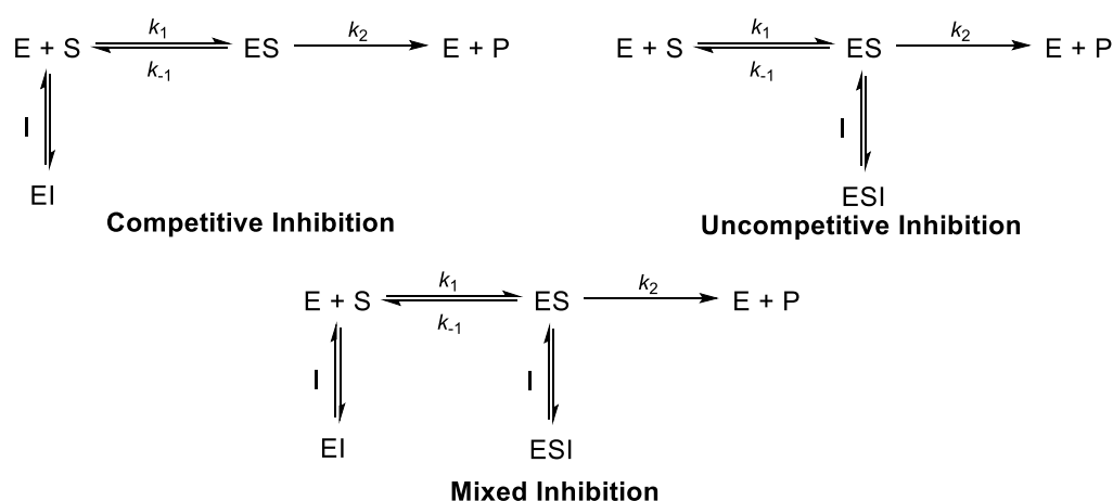
Figure 27. Reaction models of enzyme inhibition modes. [57]
