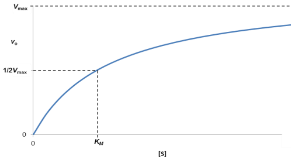
Figure 26. A generic Michaelis-Menten plot. [57]
