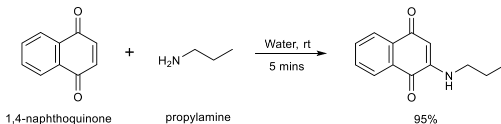
Figure 22. Michael addition of propylamine with 1,4-naphthoquinone in water. [62]
