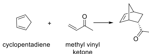
Figure 5. Diels-Alder cycloaddition of cyclopentadiene with methyl vinyl ketone. [28]
