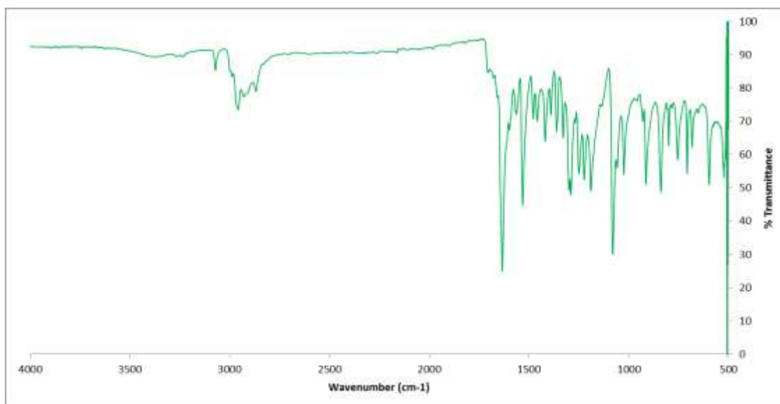
Figure A22. FTIR spectrum of compound 10c.
