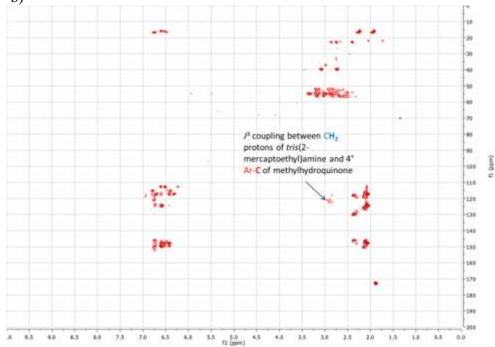
Figure 93. ^1\text{H} - ^{13}\text{C} HMBC spectrum of a) lignin-core hyperbranched copolymers, and b) product from the reaction of methyl-1,4-quinone with tris (2-mercaptoethyl)amine.
