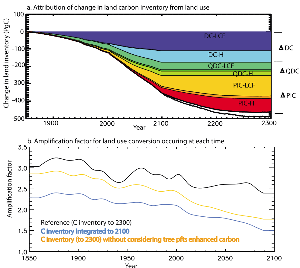
Figure 4. (a) Time series plots from 1850 to 2300 for global difference in land carbon stock from the fully coupled simulations with and without land use (e.g., difference between red solid and red dotted lines in Figure 2; blue arrow). Using equations (1–3), the relative attribution of the difference between direct carbon (DC), quasi-direct carbon (QDC), and potential indirect carbon (PIC) changes, as defined in Figure 1, is shown for three different types of processes: land conversion of forests (LCF), land conversion of nonforests (LCNF; unlabeled smaller sections between others), and harvesting (H). The colors represent, in order from top to bottom: DC-LCF (dark blue), DC-LCNF (blue, unlabeled small sliver), DC-H (cyan), QDC-LCF (green), QDC-LCNF (light green, unlabeled small sliver), QDC-H (chartreuse), PIC-LCF (orange), PIC-LCNF (dark orange unlabeled sliver), and PIC-H (red). The difference between the bottom black line (with LULCC minus without LUCC) and the colored regions represents the error in the estimation method (Table 4 at 2300). (b) Time series plots from 1850 to 2100 for global estimates of the amplification factor, AF, which represents the ratio of the sum of indirect and direct carbon loss relative to the direct carbon loss for clearing at a given time step when integrated to either 2100 (blue) or 2300 (black) (equation (5)), for tree pfts where time represents the time at which land conversion took place for reference case (equation (5): reference case; black), case where tree pfts are not considered to have more carbon relative to other pfts (orange), and the case where only indirect effects through 2100 were considered (inventory integrated to 2100; blue). This panel only extends to 2100 because the simulation stops converting land at 2100. Units of Pg C.
