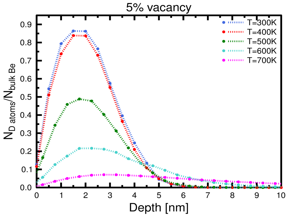
Fig. 2 Final D distribution in Be at 5% vacancy concentration to set-up MD initial structures at different surface temperatures.
