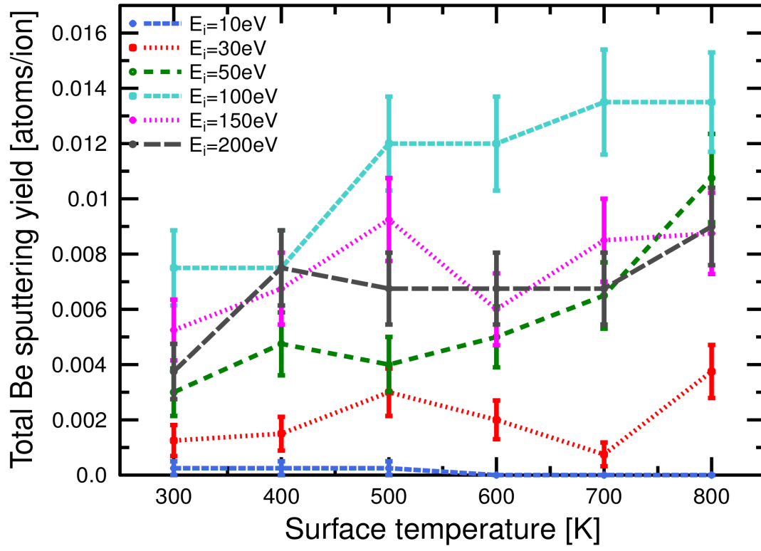
Fig. 3 Total Be sputtering yield by D irradiation as a function of temperature for different impact energies.
