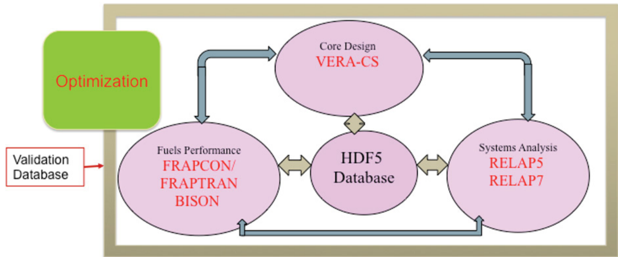
Figure 41. Schematic Illustration of Core Design Optimization Development for LOTUS.
