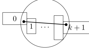
Figure 7: Boxes intersected by a line segment within a circumsphere.
