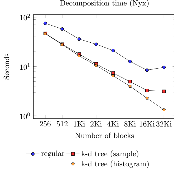
Figure 4: Decomposition time for regular vs k-d tree domain decomposition of 2048^3 points from a late-stage cosmological simulation.
