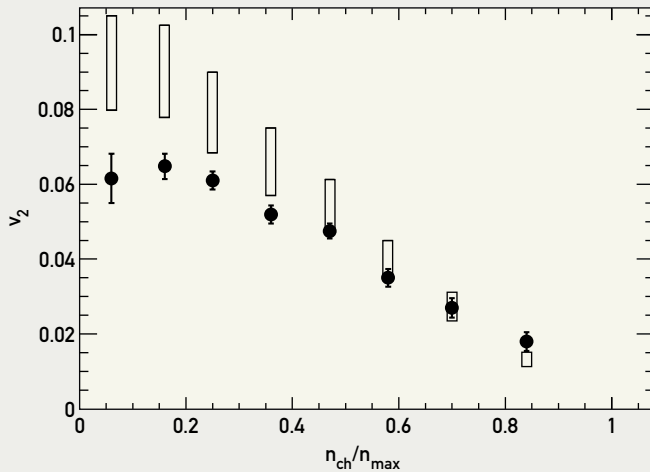
Nuclear flow. The figure plots elliptic flow v_2 (solid points) as a function of centrality, defined as n_{ch}/n_{max} , as measured by the STAR detector. The open rectangles show a range of values expected for v_2 in the hydrodynamic limit, scaled from \epsilon , the initial space eccentricity of the overlap region. The lower edges correspond to 0.19\epsilon and the upper edges to 0.25\epsilon . The startling feature of these data is that, for central events ( n_{ch}/n_{max} > 0.5 ), the flow signal appears to be as strong as allowed by hydrodynamics, implying an early equilibration of the system.
