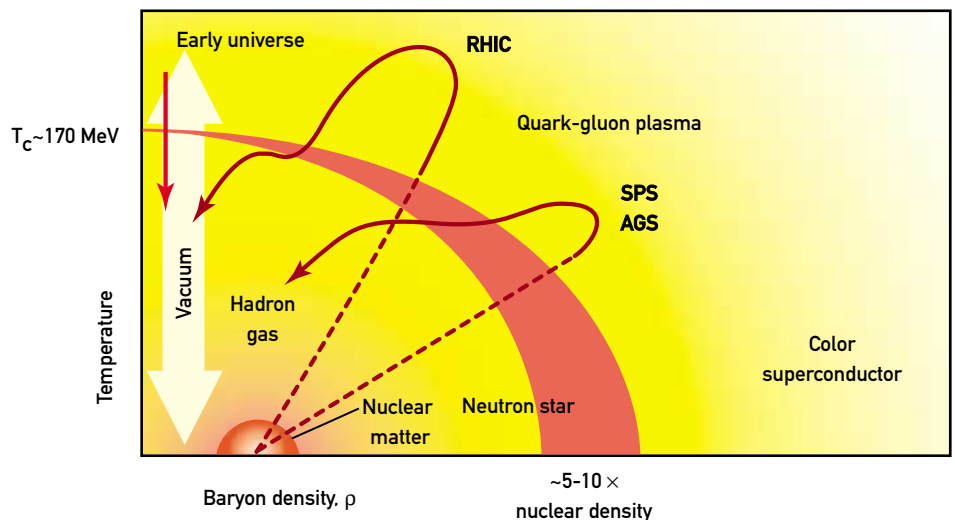
Figure 2.14. The phases of QCD. The QCD phase diagram, with baryon density as the abscissa and temperature as the ordinate. The red band indicates the range of temperatures and baryon densities at which phase transitions (both chiral and deconfinement) are thought to occur. The vacuum is the region near the y -axis, with a net baryon density near zero. Trajectories are also shown for systems created at the AGS and SPS, with center-of-mass energies of approximately 4–20 GeV per nucleon pair, and at RHIC, with a center-of-mass energy of 200 GeV per nucleon pair. The region of cold, high-density color-superconducting matter is shown to the far right.
