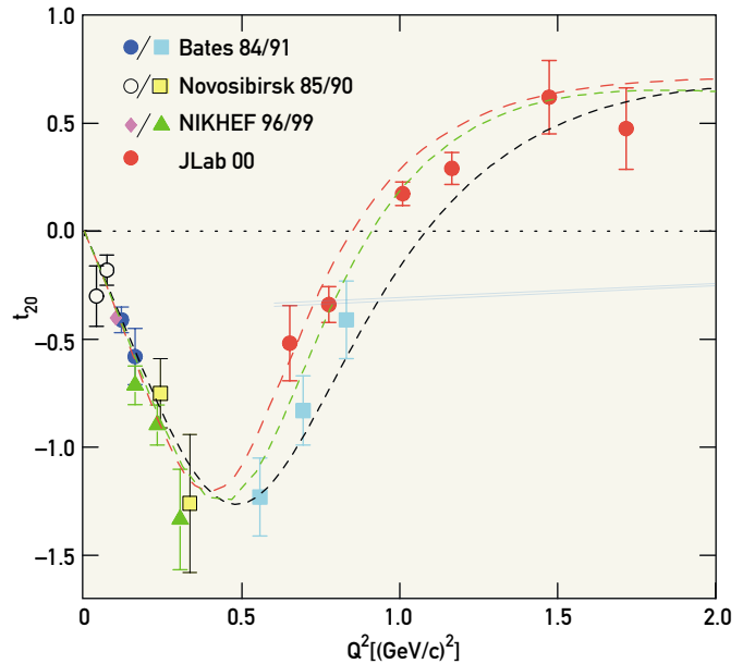
Figure 2.9. New t_{20} data from Jefferson Lab. Calculations using the traditional meson-exchange picture (the dashed curves) agree best with the new data, even at distance scales where the neutron and proton overlap significantly (at and above Q^2 \sim 1 ), whereas the perturbative QCD calculation (double solid line) does not describe the data at all.
