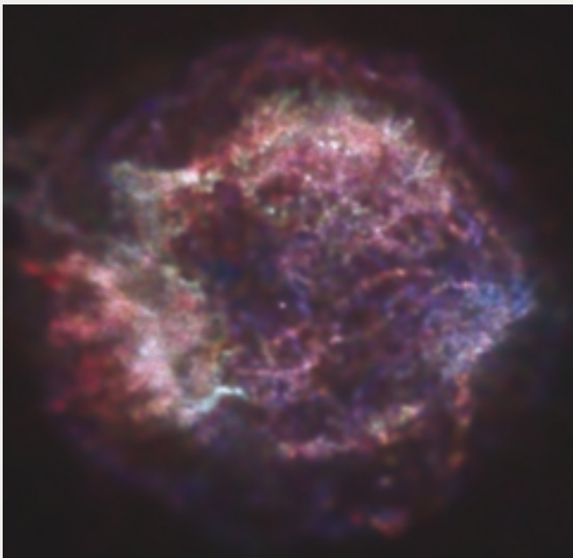
Remnants of Cas A. Supernova explosions such as this, which is 10,000 light-years distant, contain the elements that make up people and planets. This Chandra X-ray Observatory image of the supernova remnant Cassiopeia A shows in unprecedented detail where the intensities of low-, medium-, and high-energy x-rays are greatest (red, green, and blue, respectively). The red material on the left outer edge is enriched in iron, whereas the bright greenish white region on the lower left is enriched in silicon and sulfur. In the blue region on the right edge, low- and medium-energy x-rays have been filtered out by a cloud of dust and gas in the remnant. The iron-rich features synthesized deepest in the star are near the outer edge of the remnant, surprisingly suggesting that the explosion turned the star completely inside out. Image courtesy of NASA/CXC/SAO.
