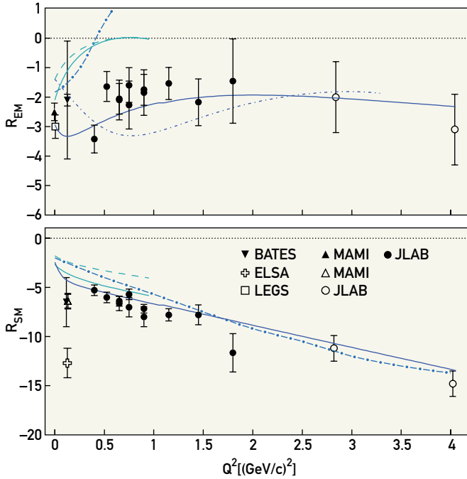
Figure 2.3. Data from LEGS (Brookhaven), MAMI (University of Mainz), ELSA (University of Bonn), MIT-Bates, and Jefferson Lab on the Q^2 dependence of the multipole ratios R_{EM} and R_{SM} for excitation of the delta resonance, the lowest-lying excited state of the proton. Curves show model calculations.
