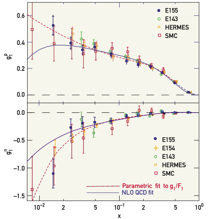
Figure 2.5. Momentum dependence of the spin structure functions for the proton and the neutron, g_1^p and g_1^n , respectively, evaluated at Q^2 = 5 \text{ (GeV/c)}^2 . The data are from experiment SLAC E155 (solid circles), E143 (open circles), and E154 (crosses); CERN SMC (squares); and DESY HERMES (stars). The solid curves correspond to a QCD fit that satisfies Bjorken's sum rule for the difference of the proton and neutron data, and confirm that the quarks carry only about one-fourth of the spin for either proton or neutron individually.
