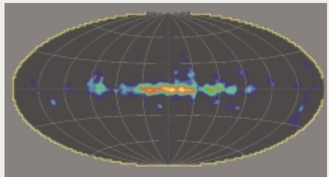
Aluminum in the galaxy. A detailed map made by COMPTEL shows the intensity of 1.8-MeV gamma-ray lines in our galaxy. These photons correspond to the radioactive decay of ^{26}\text{Al} into ^{26}\text{Mg} . The relatively short ( 7.2 \times 10^5 years) half-life of this decay (compared to the galactic age of billions of years) means that the ^{26}\text{Al} was synthesized by nuclear reactions relatively recently. From S. Plüschke et al., AIP Conf. Proc. 510, 35 (2000).
