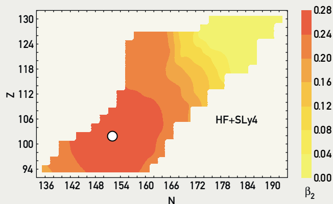
Stability from deformation. The colors in this plot indicate the degree of deformation, as measured by the quadrupole deformation \beta_2 , predicted by a theoretical model labeled as HF + SLy4. The larger the value of \beta_2 , the greater the prolate deformation of the nucleus. The open circle shows the location of ^{254}\text{No} .
