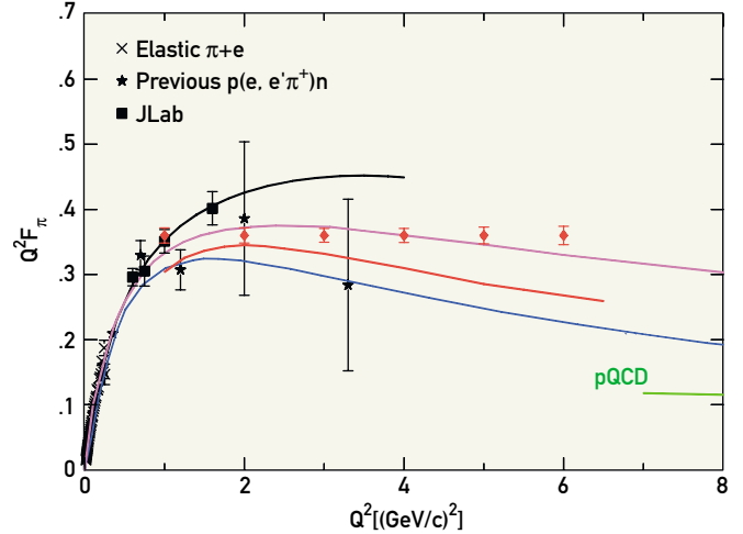
Figure 2.8. Projections for an upgraded CEBAF. The 12-GeV Upgrade will allow measurements of the pion elastic form factor through the expected transition region from confinement-dominated dynamics (at modest Q^2 ) to perturbative-dominated dynamics (at high Q^2 ). The colored symbols depict the expected precision at values of Q^2 \leq 6 . The curves represent model predictions of this transition, while the pQCD result (lower right) is the predicted value at high Q^2 .
