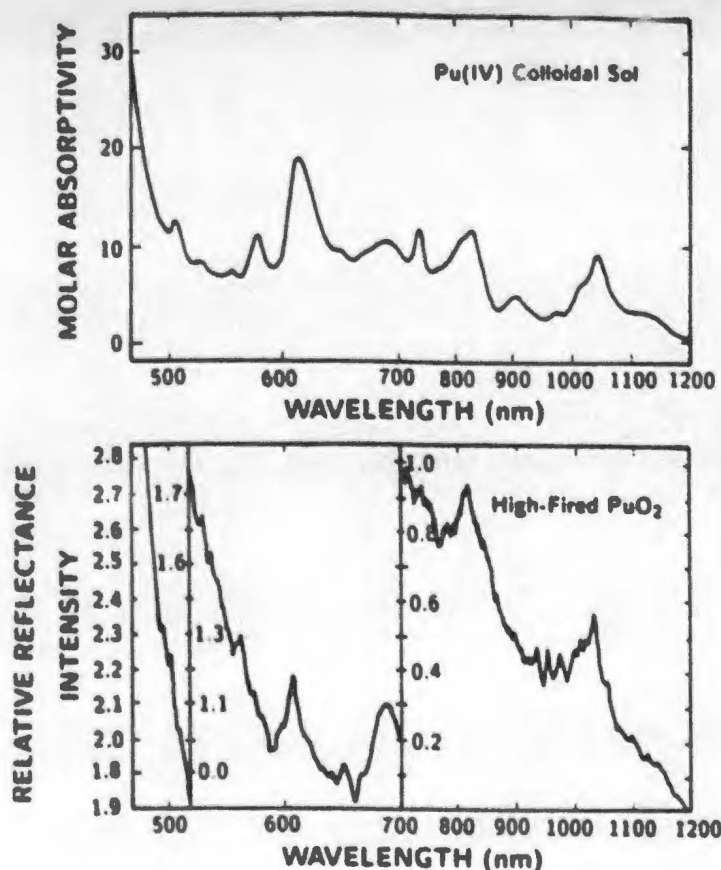
FIGURE 2. ABSORPTION SPECTRUM OF Pu(IV) COLLOIDAL SOL AND DIFFUSE REFLECTANCE SPECTRUM OF HIGH-FIRED PLUTONIUM DIOXIDE.
