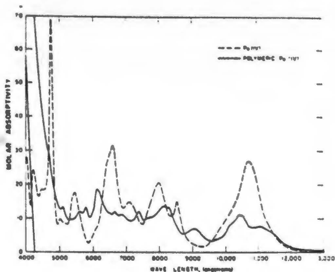
FIGURE 1. ABSORPTION SPECTRA OF AQUO \text{Pu}(\text{IV}) AND \text{Pu}(\text{IV}) COLLOIDAL SOL.
