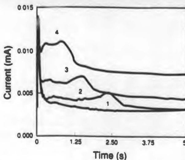
FIGURE 6. CHRONOAMPEROGRAMS FOR THE REDUCTION OF Pu(IV) COLLOID IN DILUTE HYDROCHLORIC ACID AT A MERCURY CATHODE.
