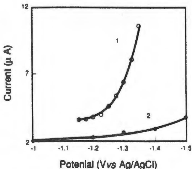
FIGURE 7. CURRENT-VOLTAGE CURVES CONSTRUCTED FROM CHRONOAMPEROMETRIC DATA FOR THE REDUCTION OF Pu(IV) COLLOID IN DILUTE HYDROCHLORIC ACID AT A MERCURY ELECTRODE.
