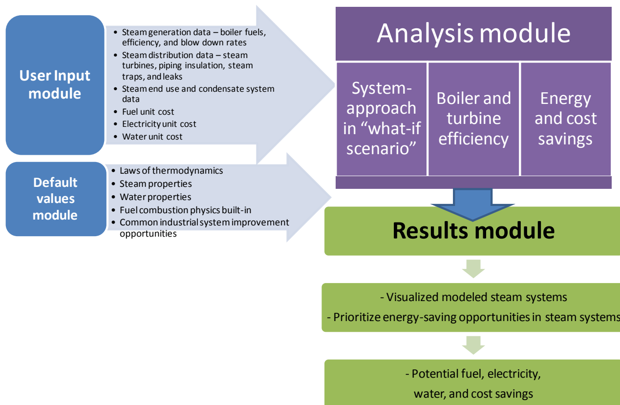
Figure 7 Flow Chart and Structure of the Steam System Assessment Tool
