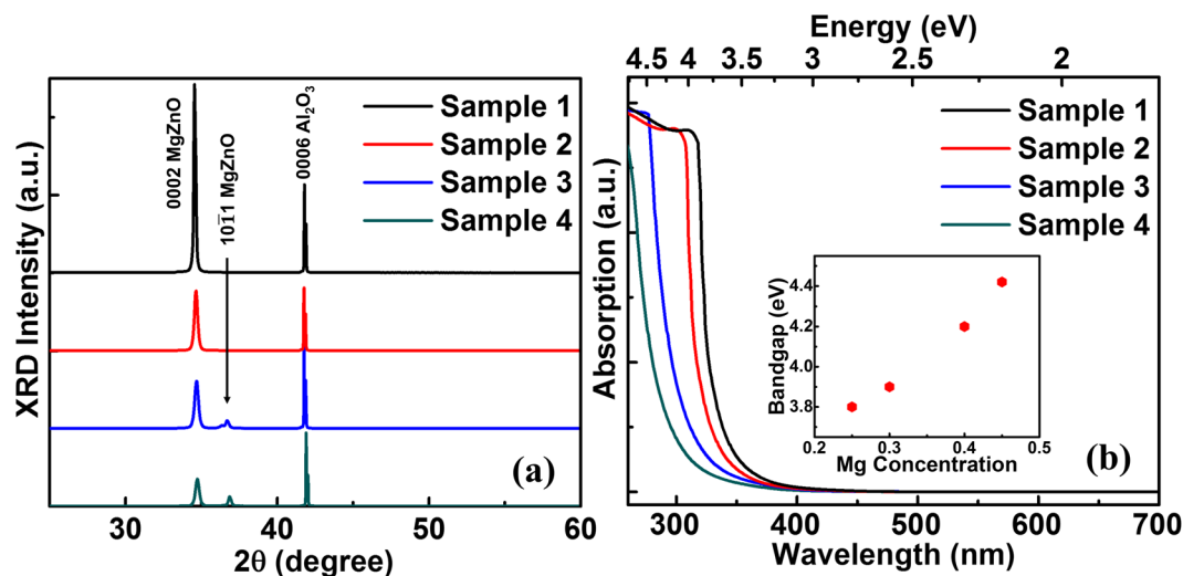
Figure 2. Structural and bandgap properties of MgZnO thin films. (a) XRD spectra of MgZnO thin films (Samples 1–4). (b) Room-temperature absorption spectra of MgZnO thin films (Samples 1–4), inset shows the variation of bandgap with Mg content in the film.
