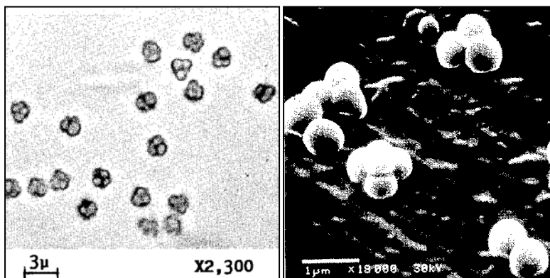
Fig. 13 Multi-lobe latex particles of different sizes:
