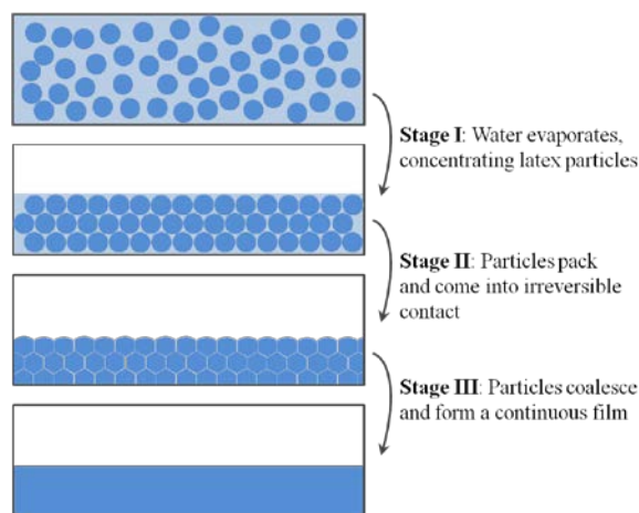
Fig. 10 Stages of the film formation process. 50
