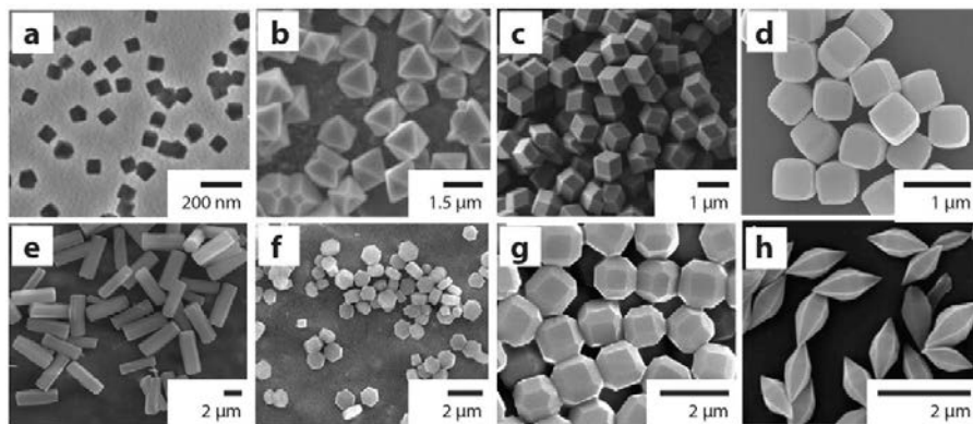
Fig. 2. Examples of polyhedral colloids synthesized from metal-organic frameworks: (a) cubes, (b) octahedra, (c) rhombic dodecahedra, (d) truncated cubes, (e) hexagonal rods, (f) hexagonal discs, (g) truncated rhombic dodecahedra, and (h) bipyramidal hexagonal prisms. Reproduced from ref. 11 with permission from the American Chemical Society, copyright 2014.
