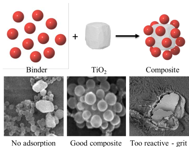
Fig. 18 Process of forming the polymer-pigment composite. 47
