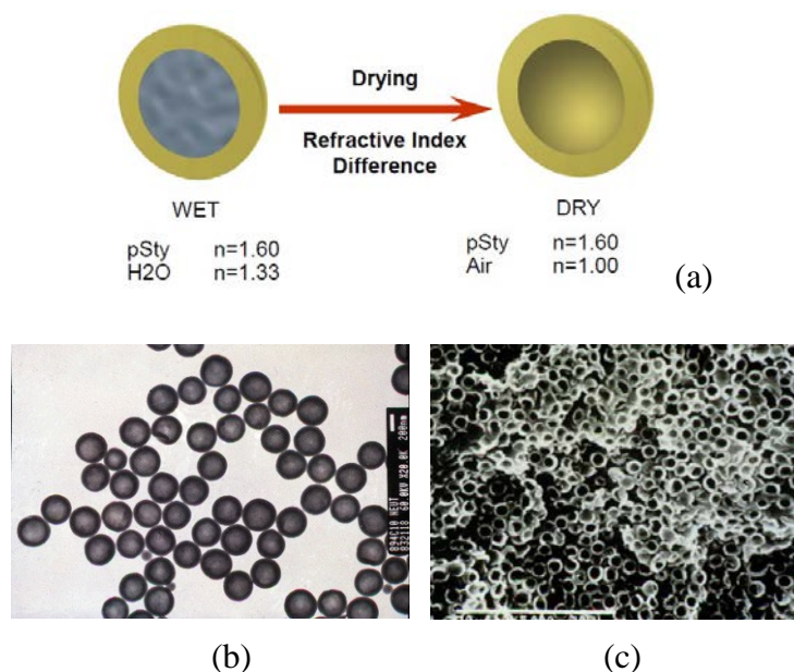
Fig. 16 Opaque polymer images (a) schematic plot; (b) under optical microscope in aqueous solution; (c) cross-section under the electron microscope. 82
