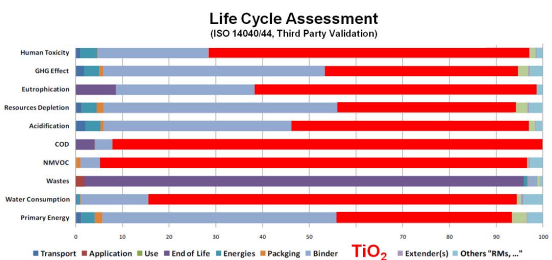
Fig. 15 Life cycle assessment for major coating component: TiO 2 has a large environment footprint. 47
