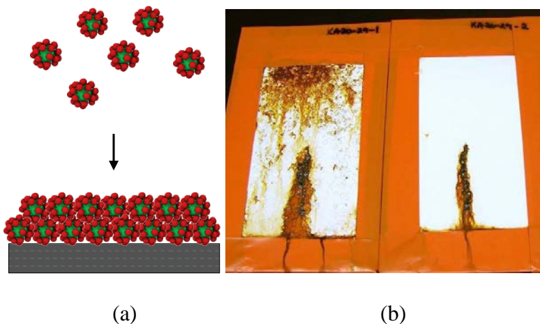
Fig. 21. (a) Schematic plot of film formation from composite polymer (red spheres) and TiO 2 (green spheres); (b) comparison of salt spray resistance of composite polymer versus the conventional binder. 47
