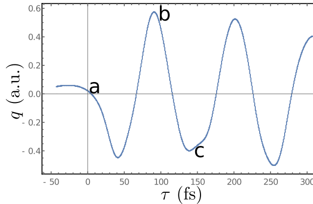
FIG. 4. Bending dynamics following a 30 fs, 5.55 eV pump excitation. Shown is the time dependent average q . The corresponding molecular geometries (a), (b), and (c) of Fig. 1 are marked at three key points.
