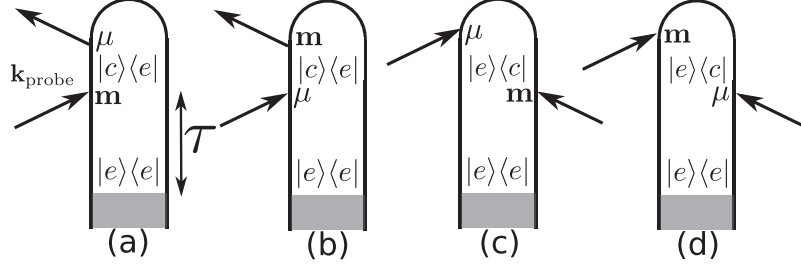
FIG. 3. Loop diagrams 28 contributing to the TRCD signal are defined in Equation (9). One has to consider the interaction with both the \mu \cdot \mathbf{E} or \mathbf{m} \cdot \mathbf{B} parts of the Hamiltonian. The complex conjugates of these diagrams also contribute to the signal. Diagrams (a) and (b) represent stimulated Raman, (c) and (d) represent the excited state absorption. Arrows represent the interactions with the probe. The interaction with the pump is treated implicitly and occurs during the shaded area.
