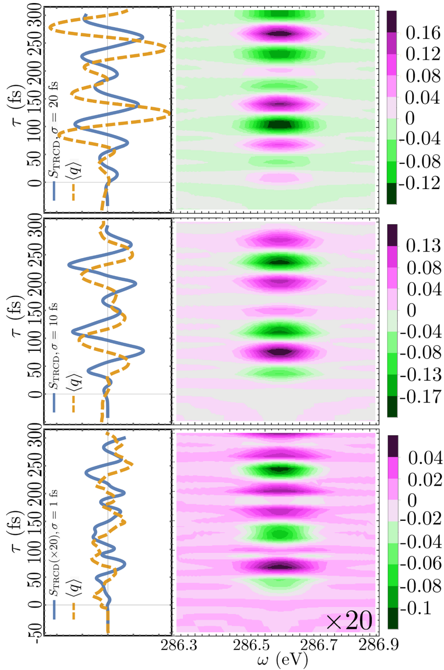
FIG. 9. Left: TRCD signals at the C K-edge (solid, blue, Eq. (16)) and the expectation value of the normal mode coordinate q (dashed, orange) calculated for three pump durations: \sigma_{pu} = 20 , 10, and 1 fs ( \omega_{pu} = 5.85 eV for all). Right: Corresponding frequency and time resolved signals.
