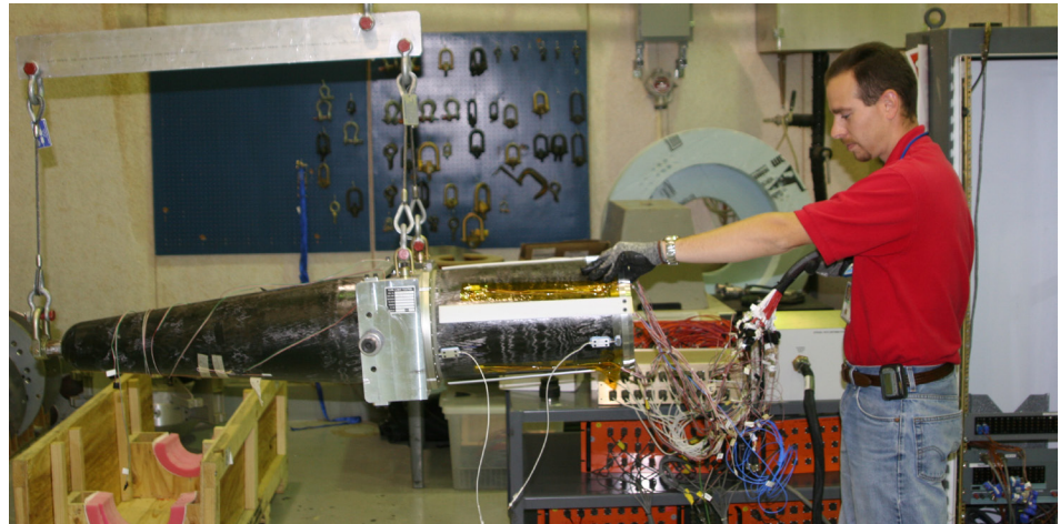
Dynamic shaker testing of a Department of Defense warhead allows engineers to determine if their designs meet the necessary requirements.
