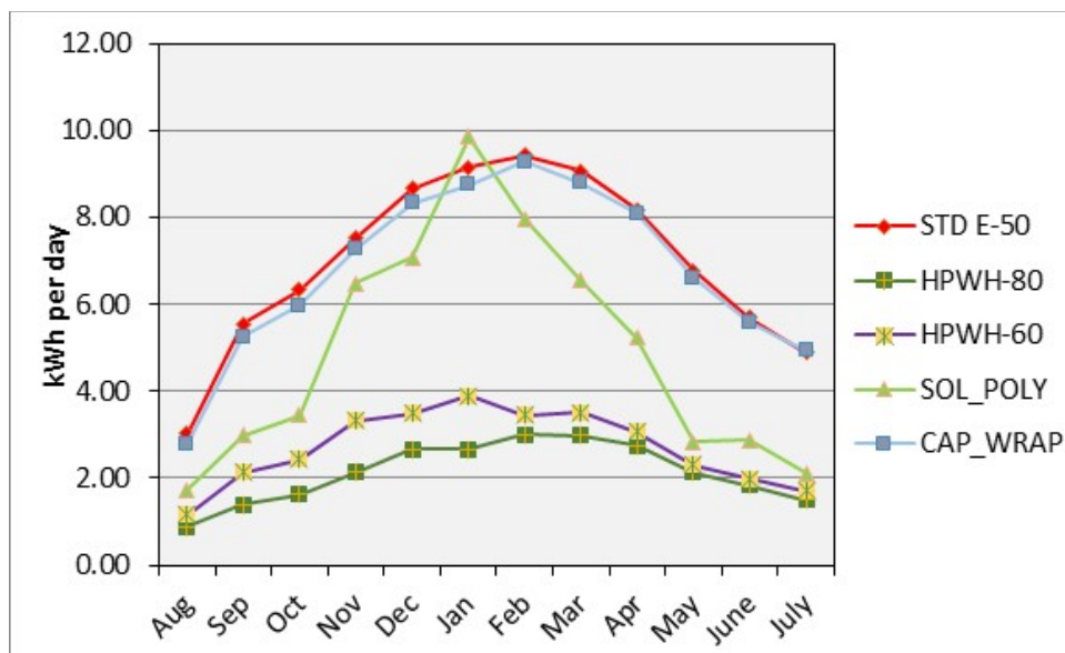
Figure 24. Average HWS daily electricity use for NREL/BA
