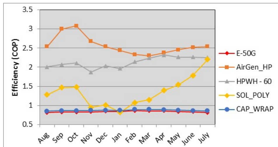
Figure 13. Average monthly efficiency performance for electric water heating systems based on typical NREL/BA hot water draws
