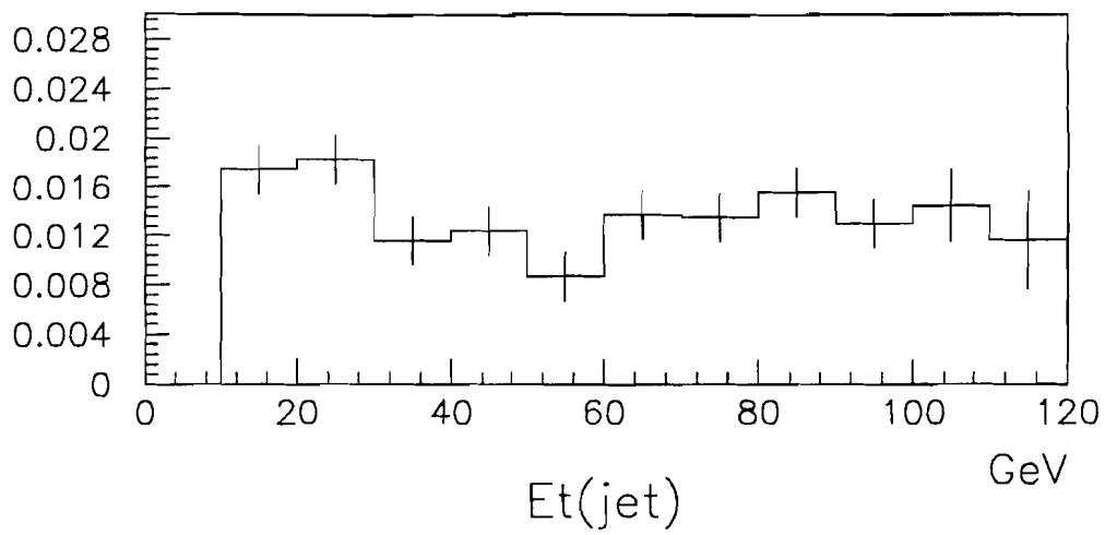
Figure 5.5: Probability for a jet to be associated to an isolated track with P_T > 5 GeV/c as a function of the jet E_T (JET50 sample).
