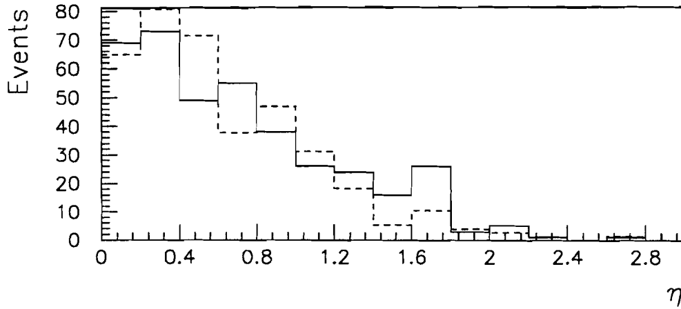
Figure 3.5: Pseudorapidity |\eta| of the two leading jets in top events (Isajet + QFL) where both W's decay leptonically. The solid line corresponds to M_{top} = 170 \text{ GeV}/c^2 while the dashed line to M_{top} = 140 \text{ GeV}/c^2 .
