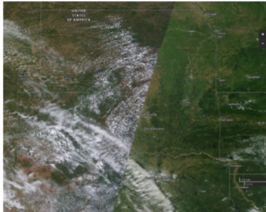
Figure 18. MODIS Terra corrected reflectance for 9-Jun-2015. Acquired from NASA EOSDIS Worldview, http://go.nasa.gov/1PpEM69 .
