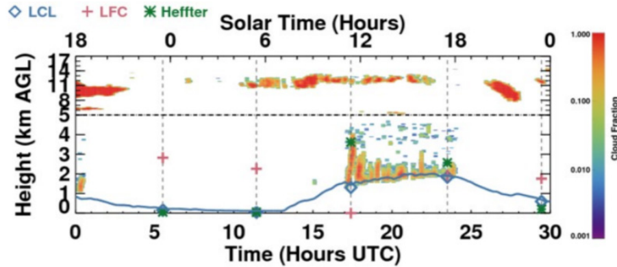
Figure 44. Cloud fraction profiles derived from the KAZR-ARSCL for 1-Aug-2015 at the Central Facility. Note the non-linear vertical axis that emphasizes the lower troposphere. Also indicated are the LCL, LFC, and PBL height based on the Heffter methodology, each of which is calculated from the SONDE product.
