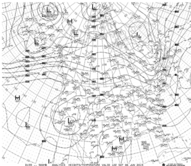
Figure 12. 500 hPa synoptic map for 6-Jun-2015 12 UTC. Acquired from Storm Research and Consulting, http://www.stormresearch.com/ncep/2015/2015_06/2015060612_500.tif .
