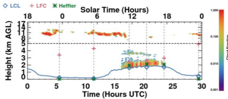
Figure 17. Cloud fraction profiles derived from the KAZR-ARSCL for 6-Jun-2015 at the Central Facility. Note the non-linear vertical axis that emphasizes the lower troposphere. Also indicated are the LCL, LFC, and PBL height based on the Heffter methodology, each of which is calculated from the SONDE product.
