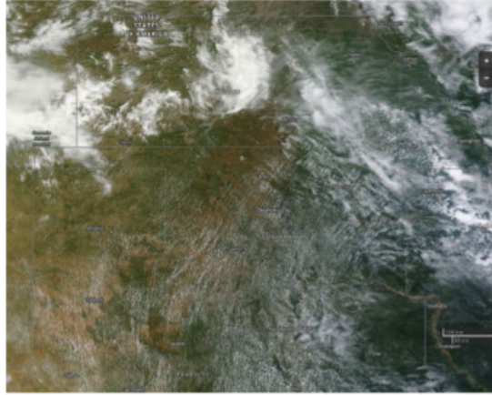
Figure 9. MODIS Terra corrected reflectance for 6-Jun-2015. Acquired from NASA EODIS Worldview, http://go.nasa.gov/1OmbCKp .
