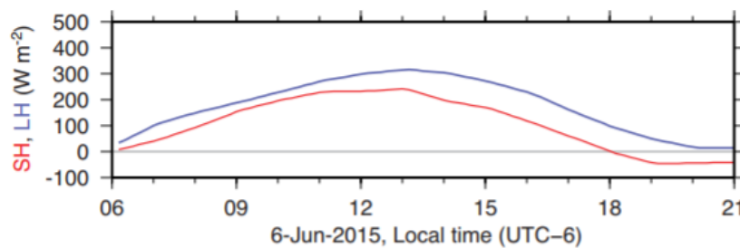
Figure 14. Surface sensible (red) and latent (blue) heat fluxes averaged for the SGP region by weighting fluxes based on percentage of land use type.
