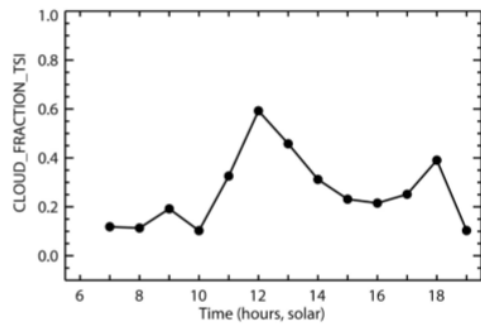
Figure 43. Cloud fraction derived from the TSI for 1-Aug-2015 at the Central Facility.
