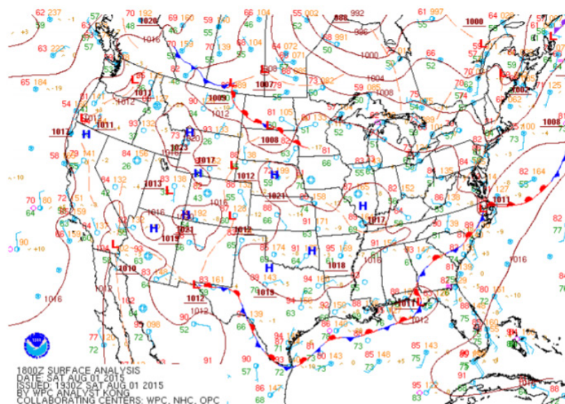
Figure 38. Surface analysis for 1-Aug-2015 18 UTC. Acquired from NWS Weather Prediction Center, http://wpc.ncep.noaa.gov/archives/web_pages/sfc/sfc_archive_maps.php?arcdte=08/01/2015&selmap=2015080118&maptpe=namussfc .
