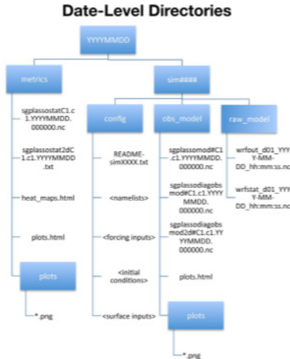
Figure 7. Schematic of the directory structure for each case date.
