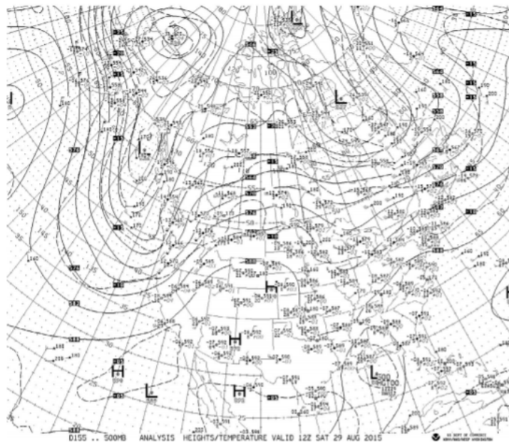
Figure 48. 500 hPa synoptic map for 29-Aug-2015 12 UTC. Acquired from Storm Research and Consulting, http://www.stormresearch.com/ncep/2015/2015_08/2015082912_500.tif .
