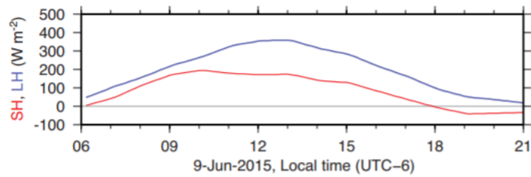
Figure 23. Surface sensible (red) and latent (blue) heat fluxes averaged for the SGP region by weighting fluxes based on percentage of land use type.
