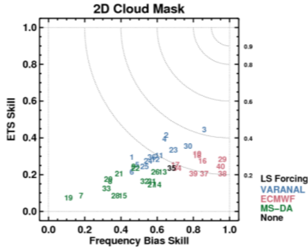
Figure 4. As for Figure 3 but for 2D cloud mask skill scores of ETS skill, S_{ETS} , and frequency bias skill, S_{Bias} . S_{ETS} is often lower than other skill scores, but this happens uniformly such that a low S_{ETS} could have comparable visual agreement with a higher time series skill score, e.g., S (LWP).
