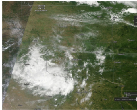
Figure 36. MODIS Terra corrected reflectance for 1-Aug-2015. Acquired from NASA EOSDIS Worldview, http://go.nasa.gov/1Omdnar .
