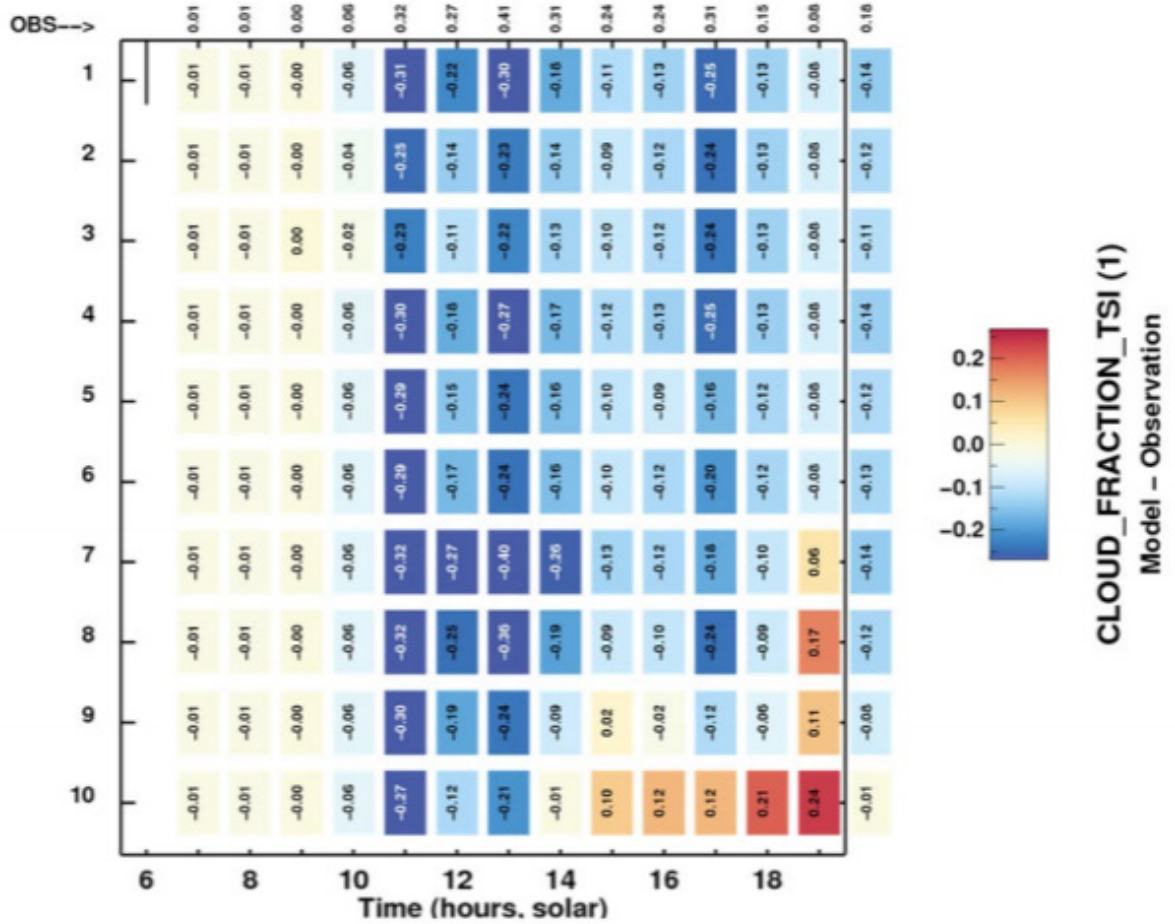
Figure 1. Heat map example of simulated cloud fraction compared to the TSI for the 27-Jun-2015 case. Simulation number is given by the left column and the local, solar time is given at the bottom. The top row gives the observational mean for each hour and the last value outside the box is the daily mean. The grid provides the corresponding differences of the simulated values (model-observation) that are color-coded by the key at the right.
