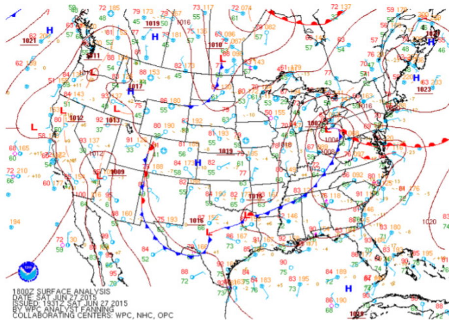
Figure 29. Surface analysis for 27-Jun-2015 18 UTC. Acquired from NSW Weather Prediction Center, http://www.wpc.ncep.noaa.gov/archives/web_pages/sfc/sfc_archive_maps.php?arcdte=06/27/2015&selmap=2015062718&motype=namussfc .
