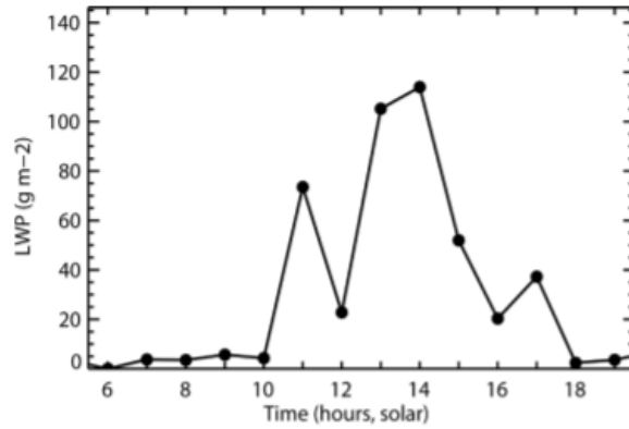
Figure 33. Cloud liquid water path for 27-Jun-2015 at the Central Facility based on MWRRet and AERIoe.
