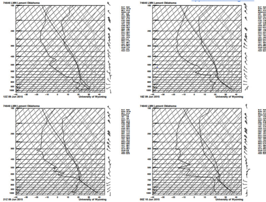
Figure 22. Skew-T log-P diagrams from Lamont, OK for 9-Jun-2015 at 12, 18, and 21 UTC and 10-Jun-2015 0 UTC. Acquired from U. Wyoming, http://weather.uwyo.edu/upperair/sounding.html .
