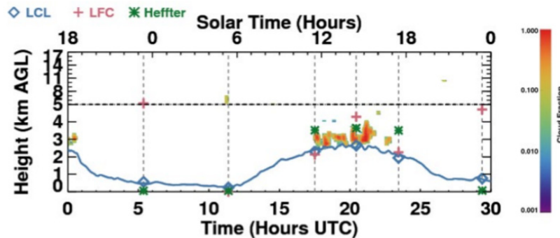
Figure 26. Cloud fraction profiles derived from the KAZR-ARSCL for 9-Jun-2015 at the Central Facility. Note the non-linear vertical axis that emphasizes the lower troposphere. Also indicated are the LCL, LFC, and PBL height based on the Heffter methodology, each of which is calculated from the SONDE product.
