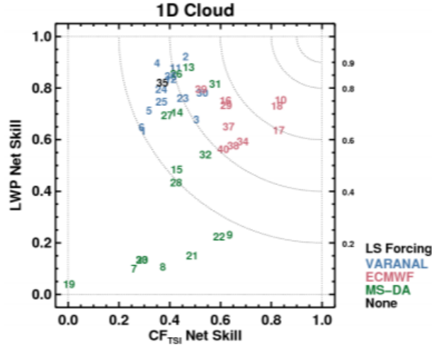
Figure 5. As for Figure 3 but for two single variable net-skill scores, S(\text{LWP}) and S(\text{CF}(\text{TSI})) . In this way simulation performance for two separate skill scores can be visualized. Should equation 8 use these two skill scores as input, it would result in a single multivariable-net-skill score for each pairing, S(\text{LWP}, \text{CF}(\text{TSI})) , that is referred to as the 1D cloud skill score .
