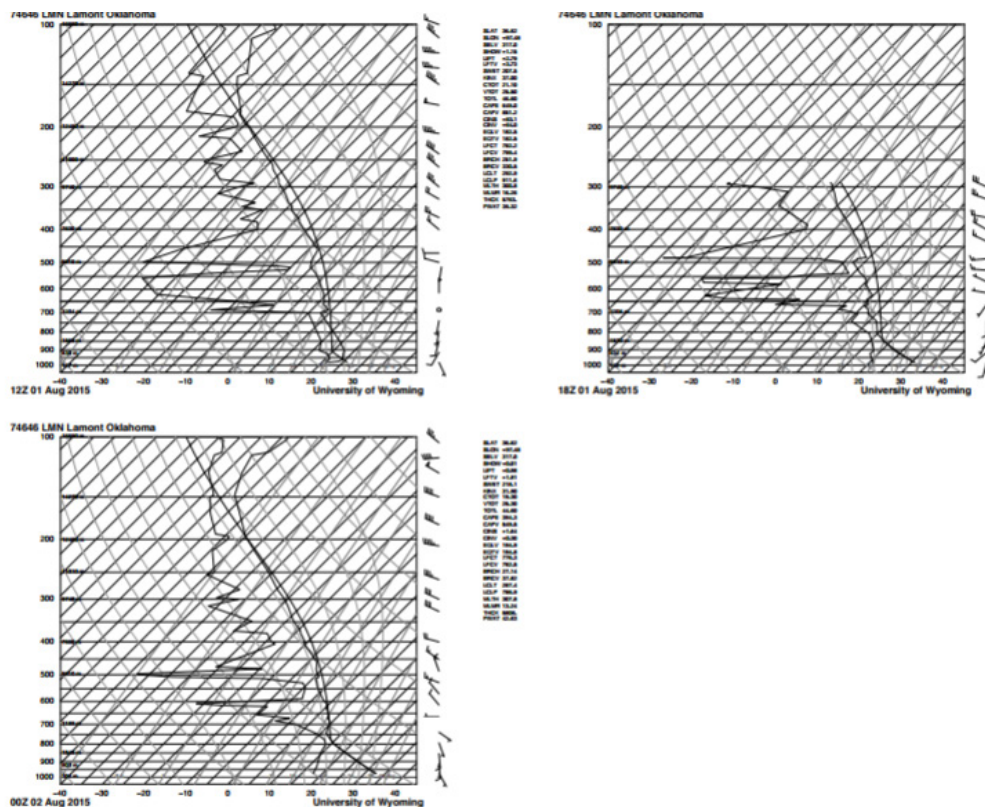
Figure 40. Skew-T log-P diagrams from Lamont, OK for 1-Aug-2015 at 12 and 18 UTC and 2-Aug-2015 0 UTC. Acquired from U. Wyoming, http://weather.uwyo.edu/upperair/sounding.html .
