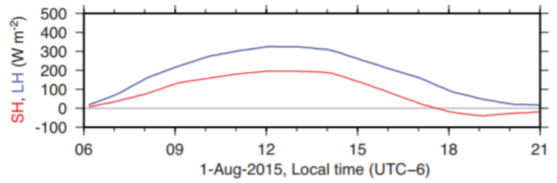
Figure 41. Surface sensible (red) and latent (blue) heat fluxes averaged for the SGP region by weighing fluxes based on percentage of land use type.
