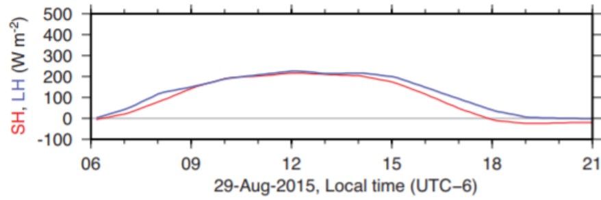
Figure 50. Surface sensible (red) and latent (blue) heat fluxes averaged for the SGP region by weighting fluxes based on percentage of land use type.
