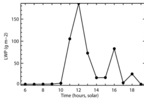
Figure 42. Cloud liquid water path for 1-Aug-2015 at the Central Facility based on MWRRet and AERIoe.
