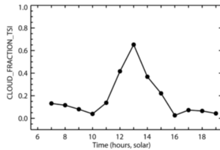
Figure 52. Cloud fraction derived from the TSI for 29-Aug-2015 at the Central Facility.
