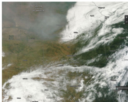
Figure 45. MODIS Terra corrected reflectance for 29-Aug-2015. Acquired from NASA EOSDIS Worldview, http://go.nasa.gov/1OmdU5G .
