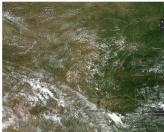
Figure 19. MODIS Aqua corrected reflectance for 9-Jun-2015. Acquired from NASA EOSDIS Worldview, http://go.nasa.gov/1OmdwL1 .
