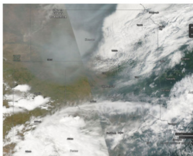
Figure 46. MODIS Aqua corrected reflectance for 29-Aug-2015. Acquired from NASA EOSDIS Worldview, http://go.nasa.gov/1PpGrZi .
