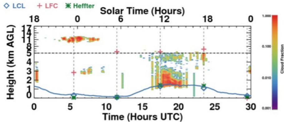
Figure 53. Cloud fraction profiles derived from the KAZR-ARSCL for 29-Aug-2015 at the Central Facility. Note the non-linear vertical axis that emphasizes the lower troposphere. Also
