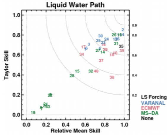
Figure 3. Scatter plot of LWP Taylor skill score, S_T (LWP), and relative mean skill score, S_{RM} (LWP), obtained from their time series comparison to observations. Each point represents a simulated day and the numbers indicate the simulation ID. Colors indicate the large-scale forcing used as indicated in the legend, where “none” is a simulation without large-scale forcing. The 40 simulations shown are from the 27-Jun-2015 case. Dashed curves are for constant values of net-skill scores, S (LWP), notated at the right axis. The closer a point is to the upper-right-hand corner (1,1), the better the simulation performance for this metric.
