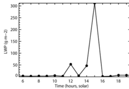
Figure 24. Cloud liquid water path for 9-Jun-2015 at the Central Facility based on MWRRet and AERIoe.
