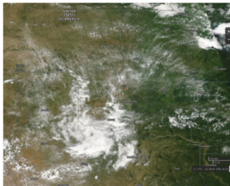
Figure 37. MODIS Aqua corrected reflectance for 1-Aug-2015. Acquired from NASA EOSDIS Worldview, http://go.nasa.gov/1PpFMHu .
