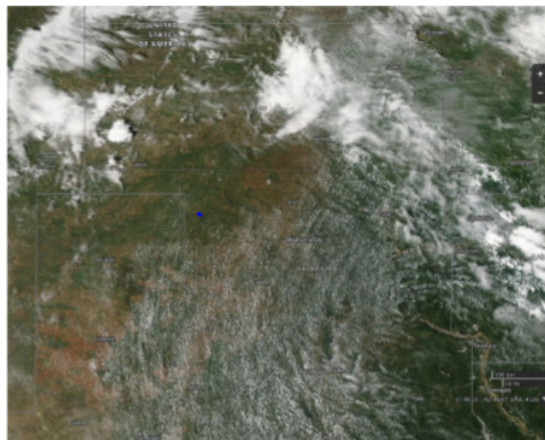
Figure 10. MODIS Aqua corrected reflectance for 6-Jun-2015. Acquired from NASA EODIS Worldview, http://go.nasa.gov/1PpDate .
