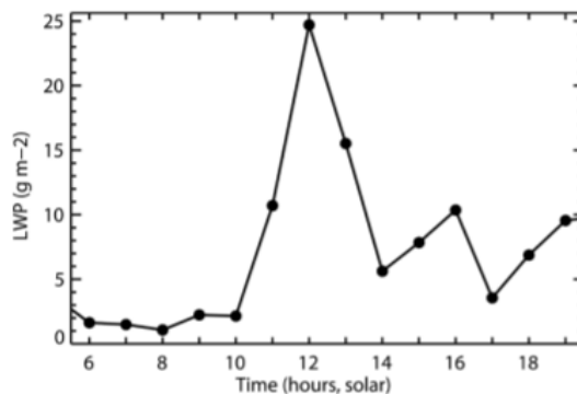
Figure 15. Cloud liquid water path for 6-Jun-2015 at the Central Facility based on MWRRet and AERIoe.
