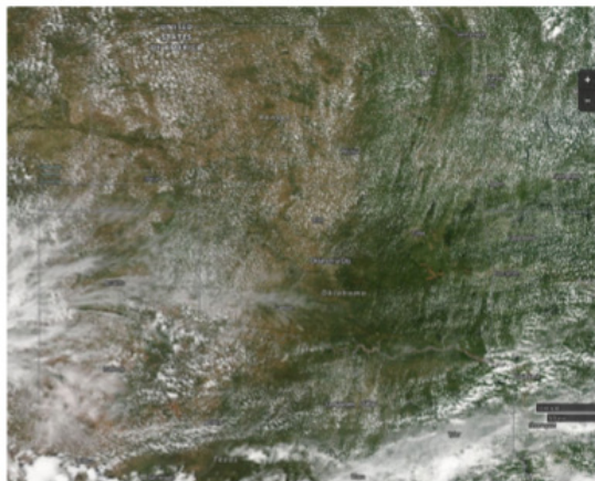
Figure 28. MODIS Aqua corrected reflectance for 27-Jun-2015. Acquired from NASA EOSDIS Worldview, http://go.nasa.gov/1PpFqAt .
