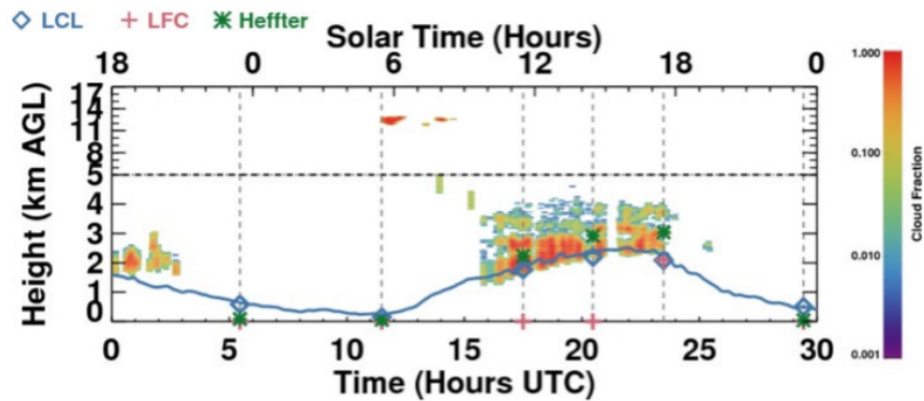
Figure 35. Cloud fraction profiles derived from the KAZR-ARSCL for 27-Jun-2015 at the Central Facility. Note the non-linear vertical axis that emphasizes the lower troposphere. Also indicated are the LCL, LFC, and PBL height based on the Heffter methodology, each of which is calculated from the SONDE product.
