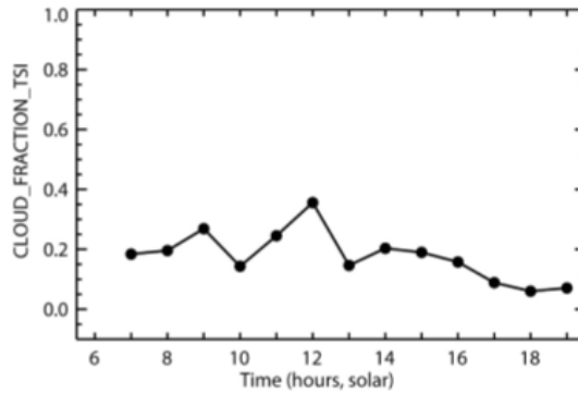
Figure 16. Cloud fraction derived from the TSI for 6-Jun-2015 at the Central Facility.
