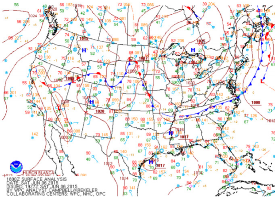
Figure 11. Surface analysis for 6-Jun-2015 18 UTC. Acquired from NWS Weather Prediction Center. http://www.wpc.ncep.noaa.gov/archives/web_pages/sfc/sfc_archive_maps.php?arcdte=06/06/2015&selmap=2015060618&motype=namussfc .
