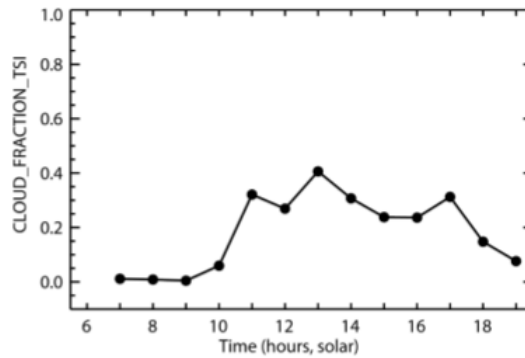
Figure 34. Cloud fraction derived from the TSI for 27-Jun-2015 at the Central Facility.
