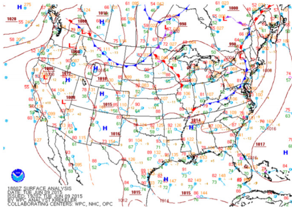
Figure 20. Surface analysis for 9-Jun-2015 18 UTC. Acquired from NWS Weather Prediction Center, http://www.wpc.ncep.noaa.gov/archives/web_pages/sfc/sfc_archive_maps.php?arcdte=06/09/2015&selmap=2015060918&maptype=namussfc .
