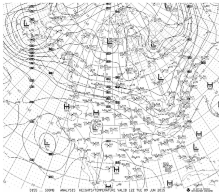
Figure 21. 500 hPa synoptic map for 9-Jun-2015 12 UTC. Acquired from Storm Research and Consulting, http://www.stormresearch.com/ncep/2015/2015_06/2015060912_500.tif .
