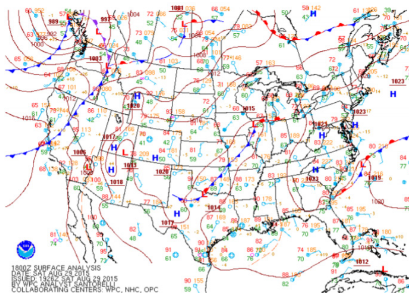
Figure 47. Surface analysis for 29-Aug-2015 18 UTC. Acquired from NWS Weather Prediction Center, http://www.wpc.ncep.noaa.gov/archives/web_pages/sfc/sfc_archive_maps.php?arcdte=08/29/2015&selman=2015082918&maptype=namussfc .
