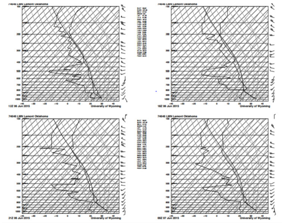
Figure 13. Skew-T log-P diagrams from Lamont, OK for 6-Jun-2015 at 12, 18, and 21 UTC and 7-Jun-2015 0 UTC. Acquired from U. Wyoming, http://weather.uwyo.edu/upperair/sounding.html .
