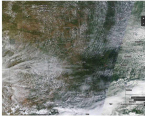
Figure 27. MODIS Terra corrected reflectance for 27-Jun-2015. Acquired from NASA EOSDIS Worldview, http://go.nasa.gov/1PpFqRd .
