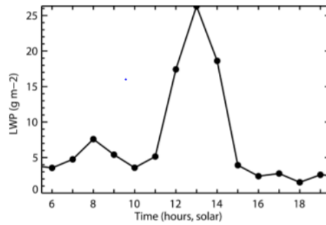
Figure 51. Cloud liquid water path for 29-Aug-2015 at the Central Facility on MWRRet and AERIoe.
