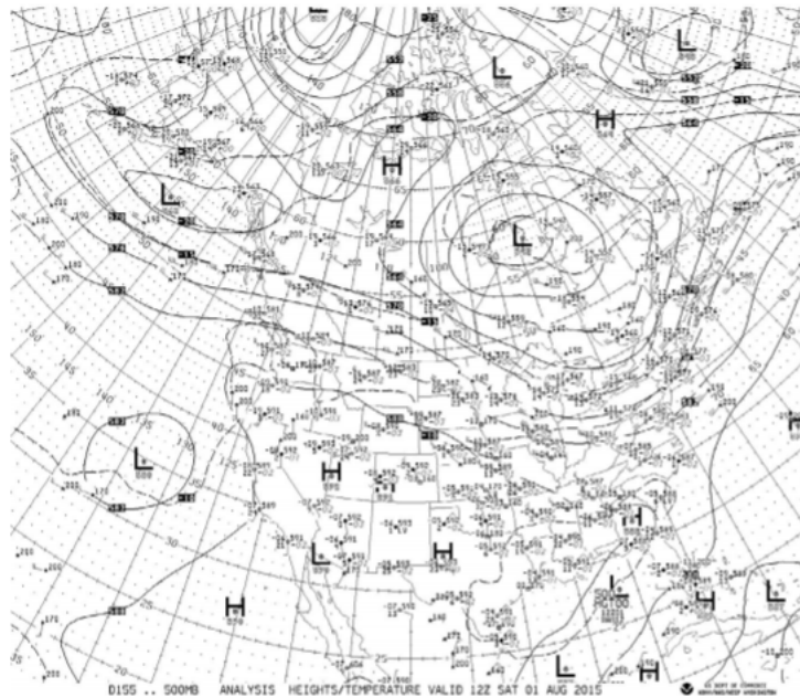
Figure 39. 500 hPa synoptic map for 1-Aug-2015 12 UTC. Acquired from Storm Research and Consulting, http://www.stormresearch.com/ncep/2015/2015_06/2015060912_500.tif .
