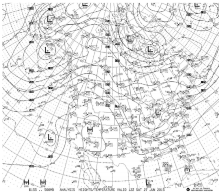
Figure 30. 500 hPa synoptic map for 27-Jun-2015 12 UTC. Acquired from Storm Research and Consulting, http://www.stormresearch.com/ncp/2015/2015_06/2015060912_500.tif .
