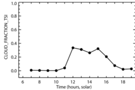
Figure 25. Cloud fraction derived from the TSI for 9-June-2015 at the Central Facility.
