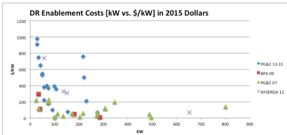
Figure 9. Comparison of costs for AutoDR systems from 2007 to present from PG&E, NYSERDA, and BPA with trimmed sample of highest outliers
