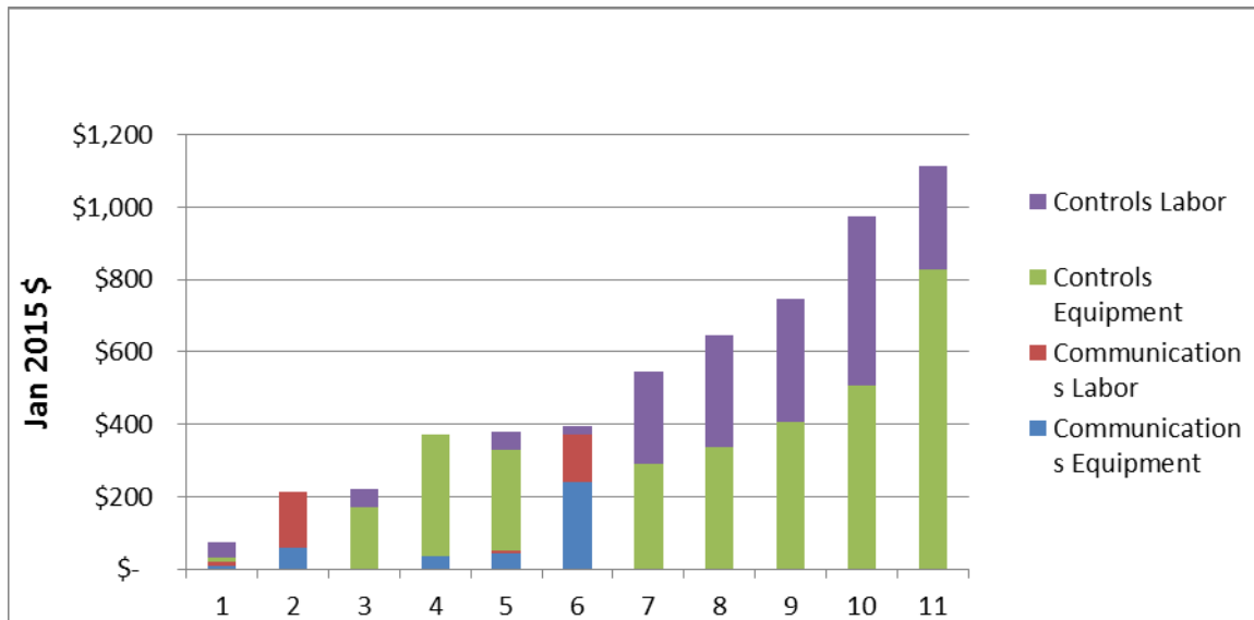
Figure A1 – Installed Cost Breakdown for Selected Sites (PG&E 2013-15)
