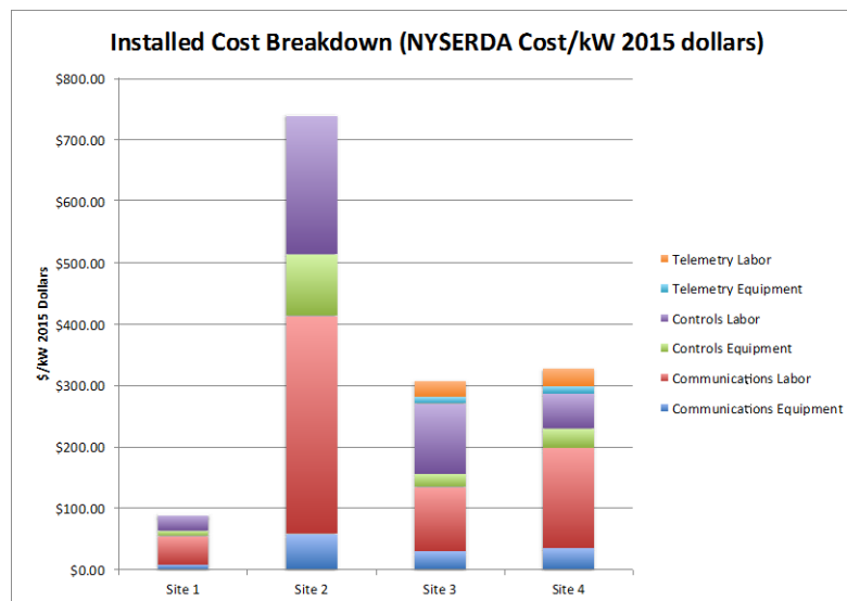
Figure 6. Costs for AutoDR systems in NYSERDA territory, in 2015 dollars
