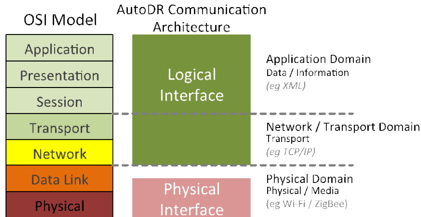
Figure 2. AutoDR control and communications system framework
