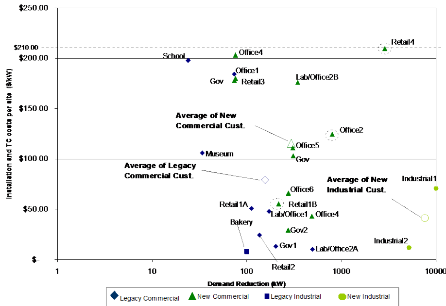
Figure 4. Costs for automated DR systems for 23 facilities in 2007 dollars
