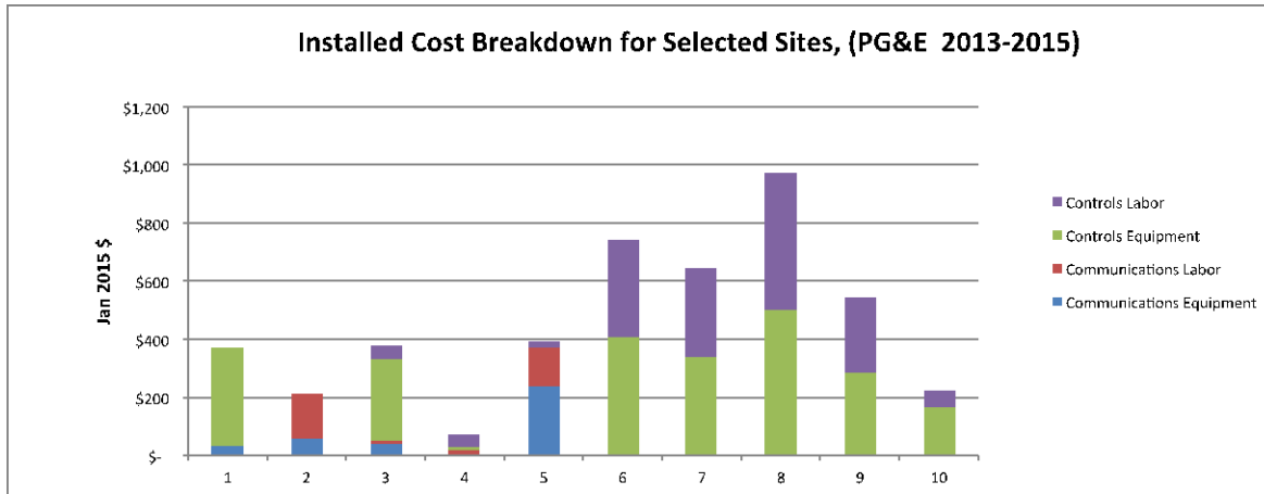
Figure 7. Costs for recent PG&E AutoDR sites using OpenADR 2.0.
