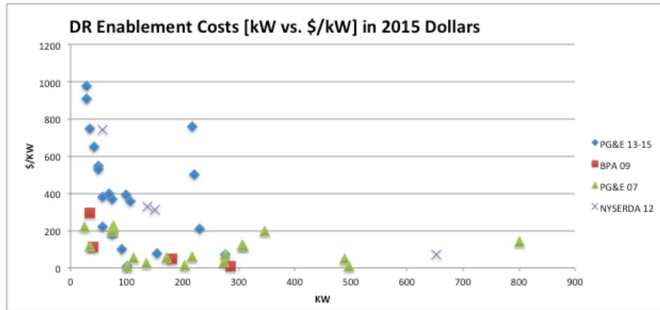
Figure A2 Comparison of costs for Auto DR systems from 2007 to present from PG&E, NYSERDA, and BPA programs (48 customers)
