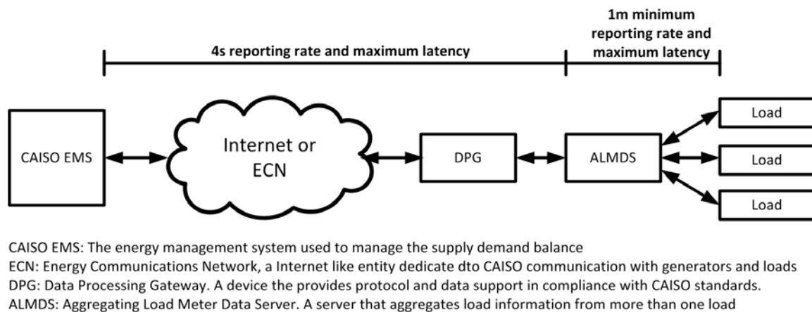
Figure 3. Schematic showing CAISO communication latency and reporting rate requirements for demand-side aggregated loads
