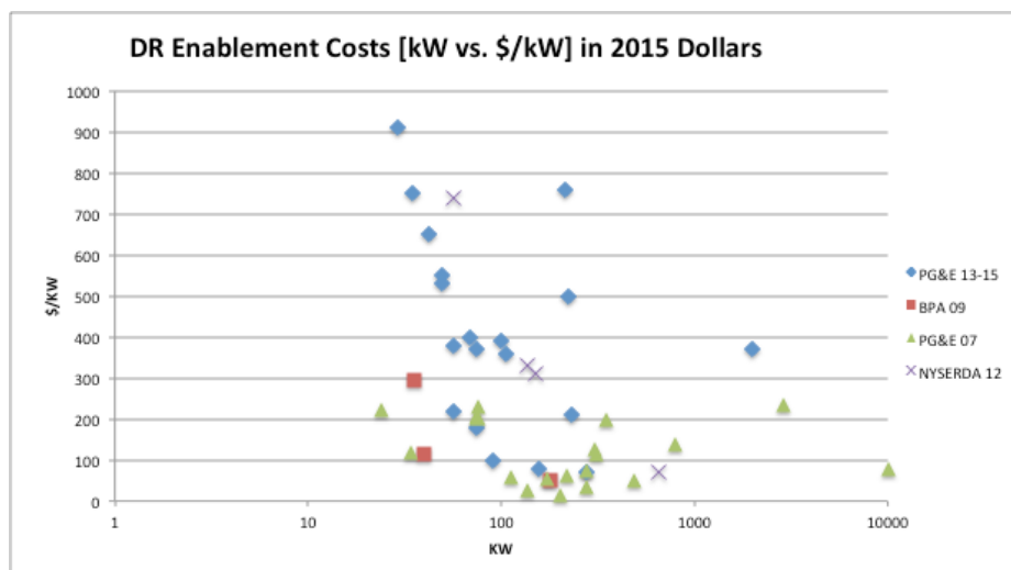
Figure A1 Comparison of costs for Auto DR systems from 2007 to present from PG&E, NYSERDA, and BPA programs (46 customers)
