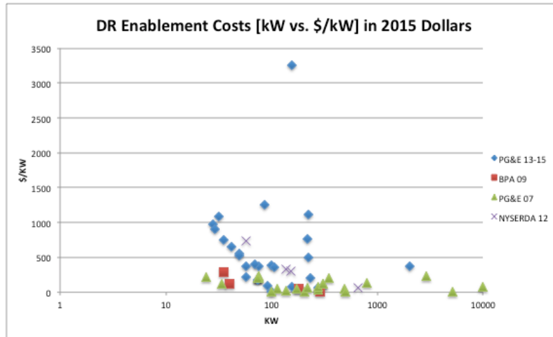
Figure 8. Comparison of costs for AutoDR systems from 2007 to present from PG&E, NYSERDA, and BPA programs
