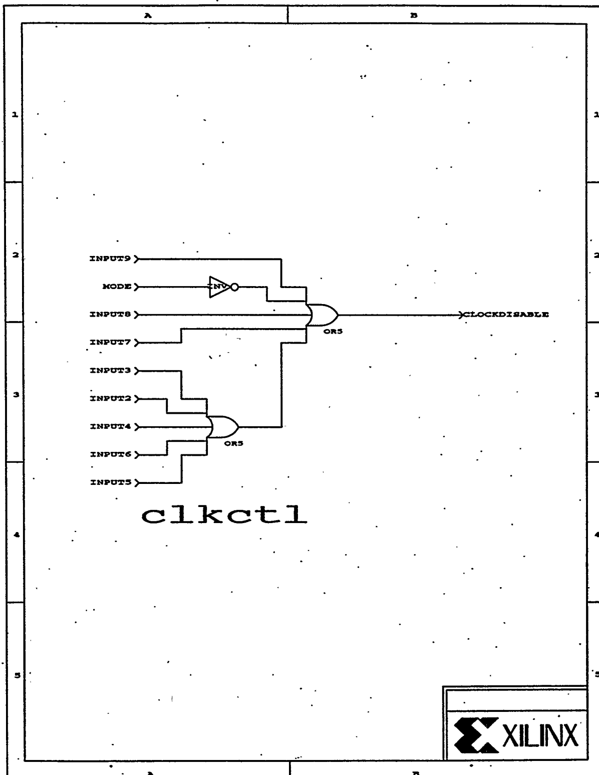
Figure L. Operating mode clock steering module.
