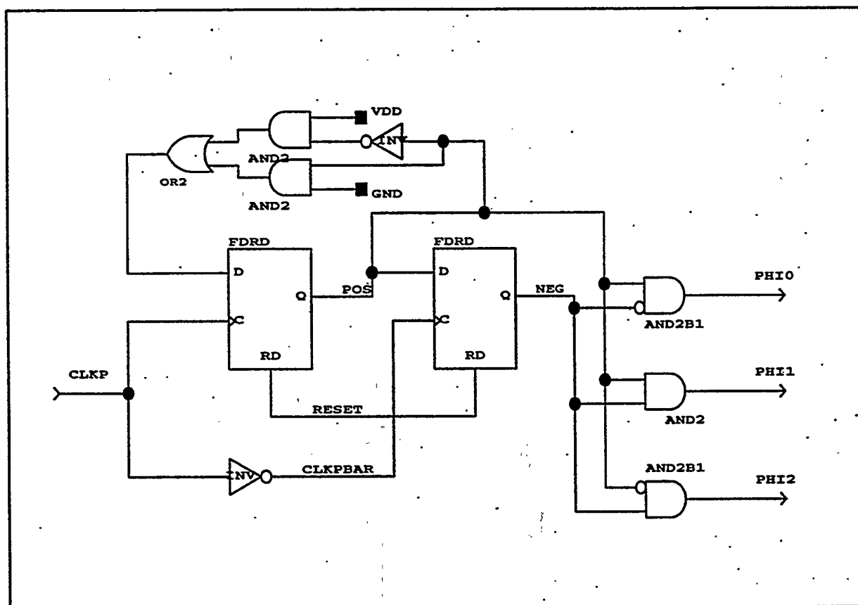
Figure 8. Glitch free clock sequencer.
