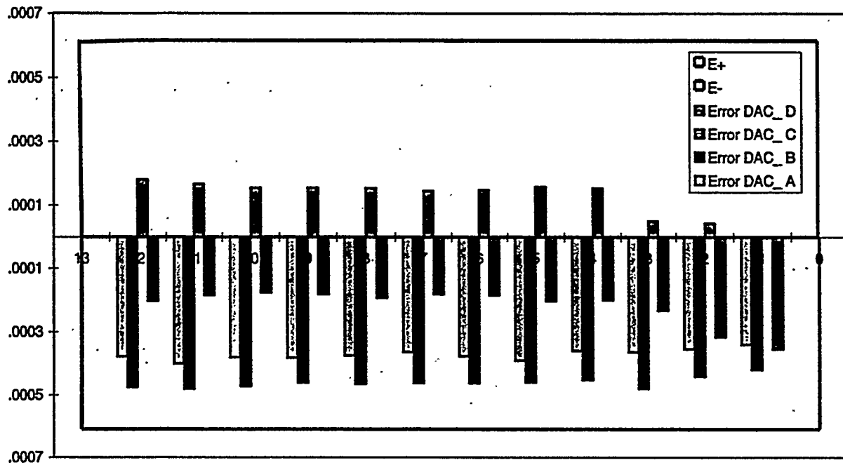
Figure 14. MAX 537 Error (Vactual - Vmeasured).
