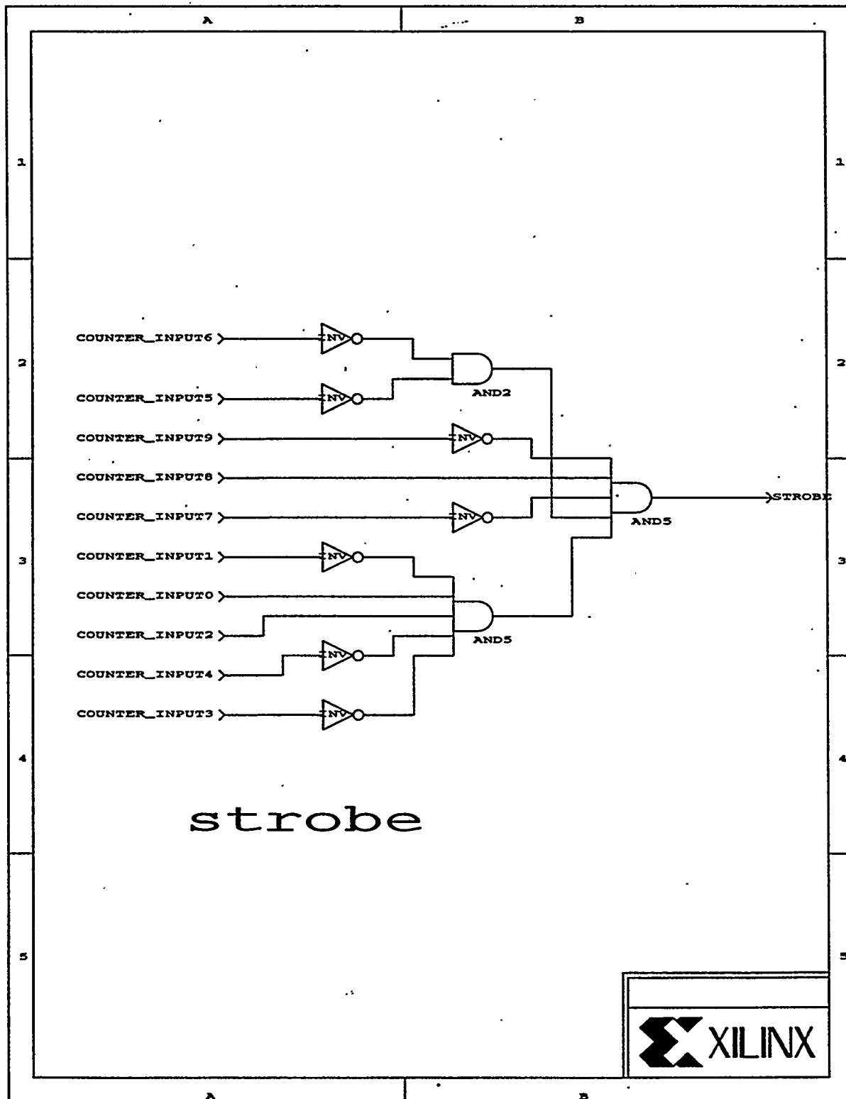
Figure K. Internal reset generator
