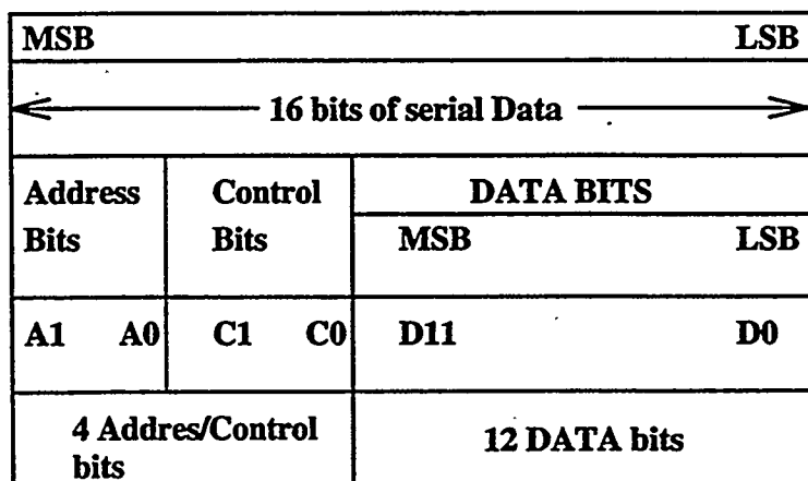
Figure. 3. Serial-Data Format (MSB sent first)
