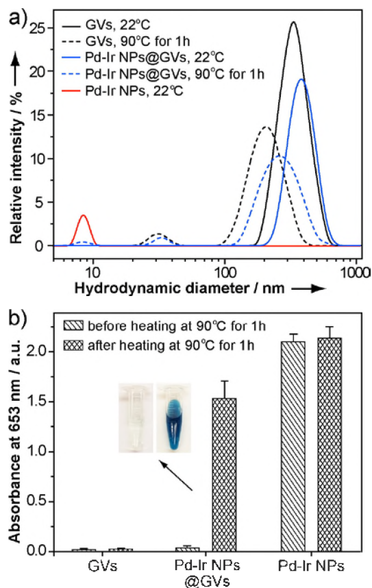
Figure 4. Comparison of the properties of Pd-Ir NPs@GVs before and after heat treatment (90 °C, 1 h). (a) DLS analysis of different samples: GV (black), Pd-Ir NPs@GV (blue), and Pd-Ir NP (red); (b) Absorbance at 653 nm measured from catalytic reaction solutions containing different particles (marked under the bars) at t = 2 min. Concentrations of GV were kept the same for suspensions of GV and Pd-Ir NPs@GV, while the concentrations of Pd-Ir NP were kept the same for suspensions of Pd-Ir NPs@GV and Pd-Ir NP. Inset shows photographs of reaction solutions corresponding to Pd-Ir NPs@GV. All tests in (a) and (b) were conducted at room temperature ( \sim 22 °C).
