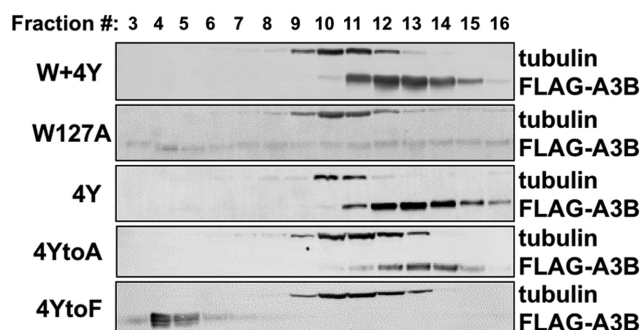
Figure 4. Analysis of the oligomeric status of the A3B mutants. W+4Y refers to W127A + Y13D/Y28A/Y83D/Y162D mutant, 4Y refers to Y13D/Y28A/Y83D/Y162D mutant, 4YtoA refers to Y13A/Y28A/Y83A/Y162A mutant, 4YtoF refers to Y13F/Y28F/Y83F/Y162F mutant.
